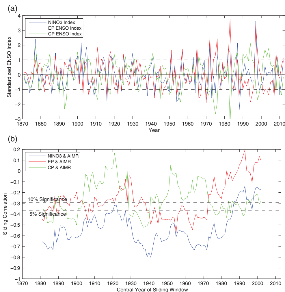
Figure 1. (a) Interannual time series of the Niño-3 SST anomaly index (blue), the EP ENSO index (red), and the CP ENSO index (green) for boreal summer season (June–September) during the 1871–2012 period. These series have been standardized to have zero mean and unit standard deviation. (b) Sliding correlations on a 21-year moving window between the ENSO indices and the AIMR index during the 1871–2012 period. The horizontal dashed lines indicate the one-tailed p=0.05 and p=0.1 significance levels.
