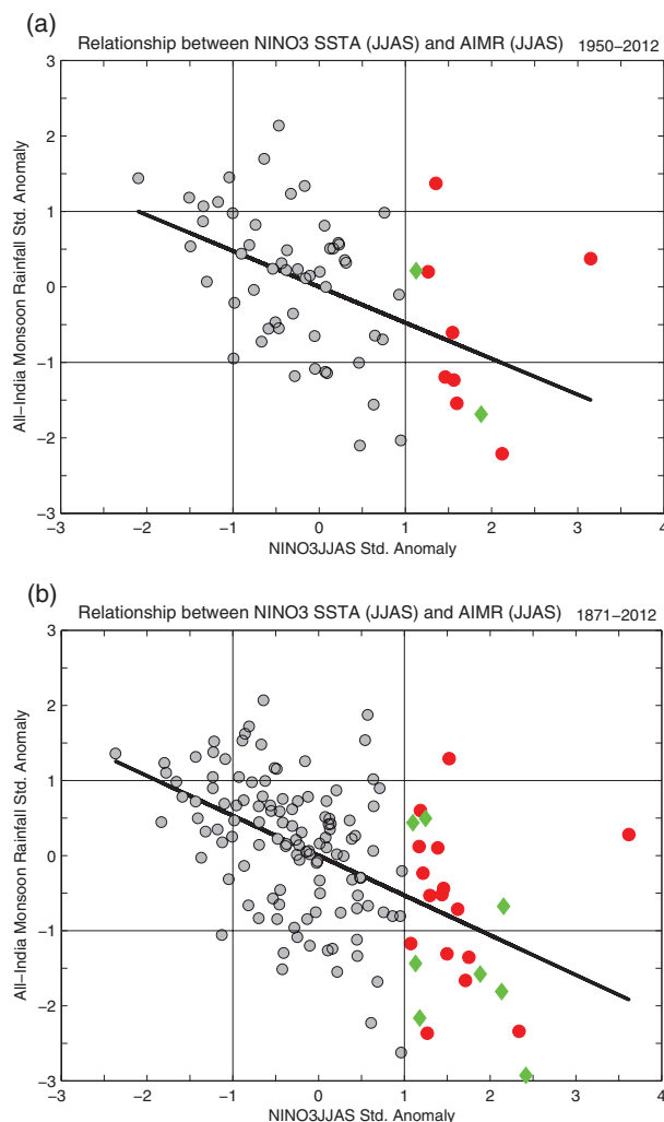
Figure 2. The standardized summer mean (June–September) Niño-3 SST anomaly index and the standardized All-India monsoon rainfall (AIMR) index during (a) the 1950–2012 period and (b) 1871–2012 period. Linear regression of the AIMR index against the Niño-3 index is shown in thick black line. EP and CP El Niño events with standardized Niño-3 SST anomaly index > 1.0 are denoted by red dots and green diamonds, respectively.
