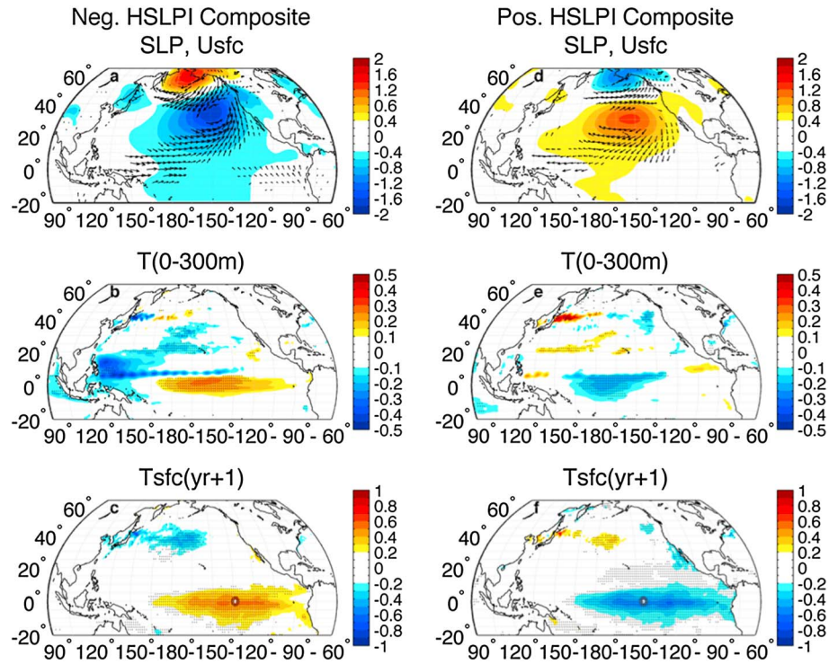
Figure 2. (a) Shading: Mean November–March SLP anomalies from 20CRv2 during years in which \text{HSLPI} < -0.5\sigma . Minimum contour is \pm 0.4\text{hPa} ; contour interval is 0.2\text{hPa} . Vectors: Mean November–March 10m wind vector anomalies from 20CRv2 during years in which \text{HSLPI} < -0.5\sigma . Only shown are those with an anomalous magnitude that is significant at the 90% confidence limit, based upon a one-sample t test of the mean assuming a normal distribution with unknown variance. (b) Shading: Mean November–March subsurface temperature anomalies from SODA, averaged between 0 and 300m, during years in which \text{HSLPI} < -0.5\sigma . Shading interval is 0.05^\circ\text{C} ; minimum shading is \pm 0.1^\circ\text{C} . Stippling indicates regions where composite anomalies are significant at the 90% confidence limit, based upon a one-sample t test of the mean assuming a normal distribution with unknown variance. (c) Composite of November–January SST anomalies from SODA when \text{HSLPI} < -0.5\sigma the previous year. Shading interval is 0.1^\circ\text{C} ; minimum shading is \pm 0.2^\circ\text{C} . Stippling as in Figure 2b. Circle indicates median CHI longitude for all subsequent HSLPI-related warm events, as found in Figure 1b. (d, e, f) Same as Figures 2a, 2b, and 2c except for years in which \text{HSLPI} > 0.5\sigma . Circle indicates median CHI longitude for all subsequent HSLPI-related cold events.
