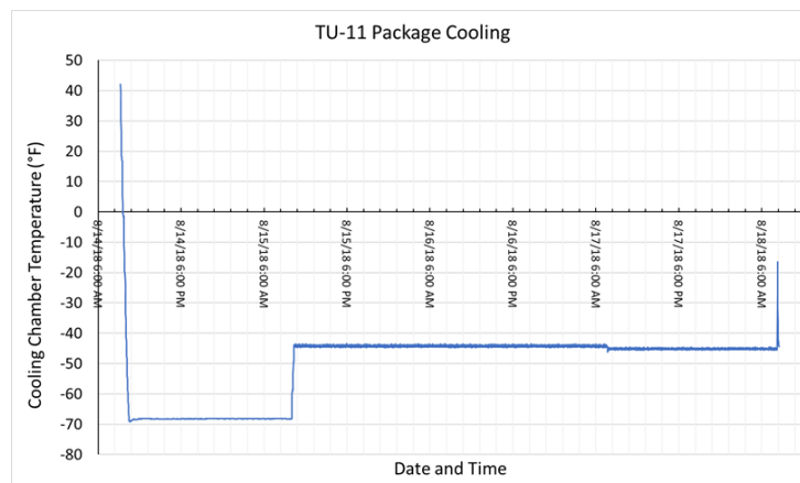
Figure 3. TU-11 cooling temperature profile
