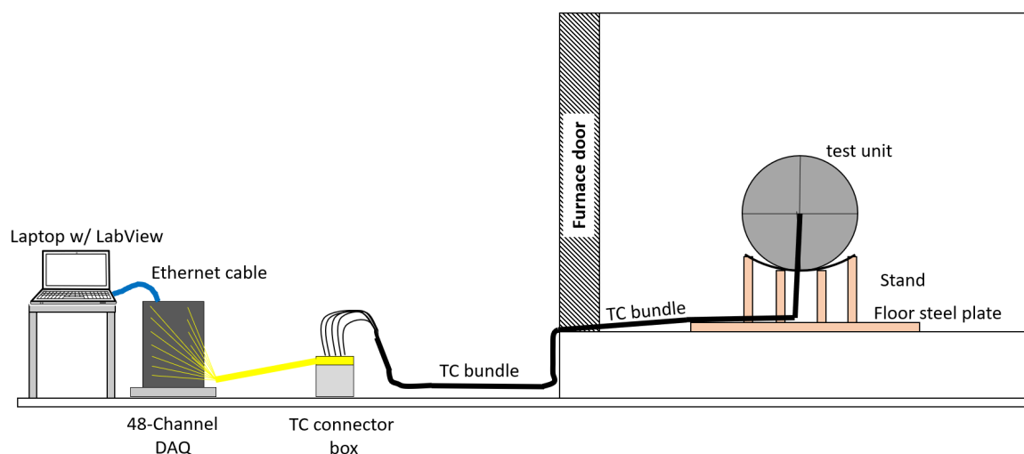
Figure 6. Thermal test instrumentation setup
