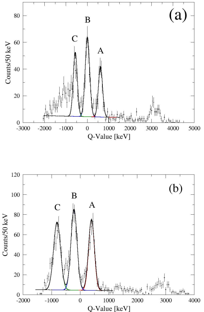
FIG. 1. (color online) Q -value spectra of (a) ^{126}\text{Sn}(d, p) and (b) ^{128}\text{Sn}(d, p) reaction measurements in inverse kinematics, summed over all angles. The uncertainties on the data are purely statistical. Colored curves represent the fits to each state and the background. A solid black line represents the sum of all of the fits and the background. The centroids extracted from the individual fits for panel (a) are Q_A = 0.62 \pm 0.04 MeV, Q_B = 0.01 \pm 0.05 MeV, and Q_C = -0.56 \pm 0.05 MeV and for panel (b) are Q_A = 0.40 \pm 0.05 MeV, Q_B = -0.21 \pm 0.05 MeV, and Q_C = -0.81 \pm 0.06 MeV. The uncertainties on the centroids are determined from the error in the fit.
