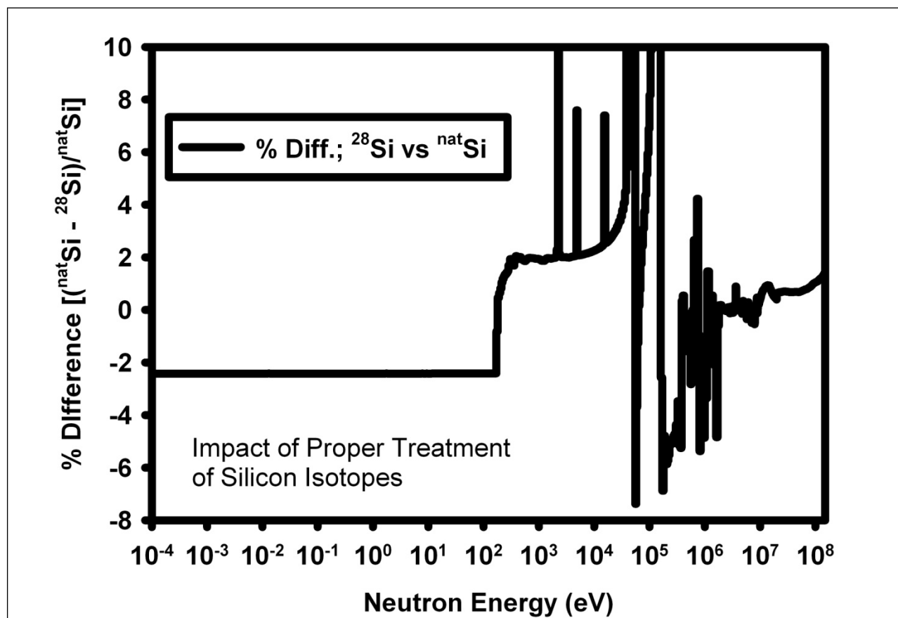
Figure 17: Difference between ^{28}\text{Si} and ^{\text{nat}}\text{Si} NRT-based Damage Metric
