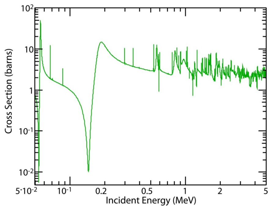
Figure 14: Total Cross Section Near the 1-MeV Energy Region
