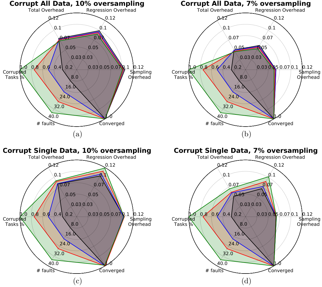
Figure 5: Statistical results obtained from the ensemble runs performed for the resilience analysis. The radar-plots correspond to the following four cases: first row shows results when all data in a sampling task is corrupted, with \rho = 1.1 (a) and \rho = 1.07 (b); second row shows results for single data point corruption in a sampling task, with \rho = 1.1 (c) and \rho = 1.07 (d).
