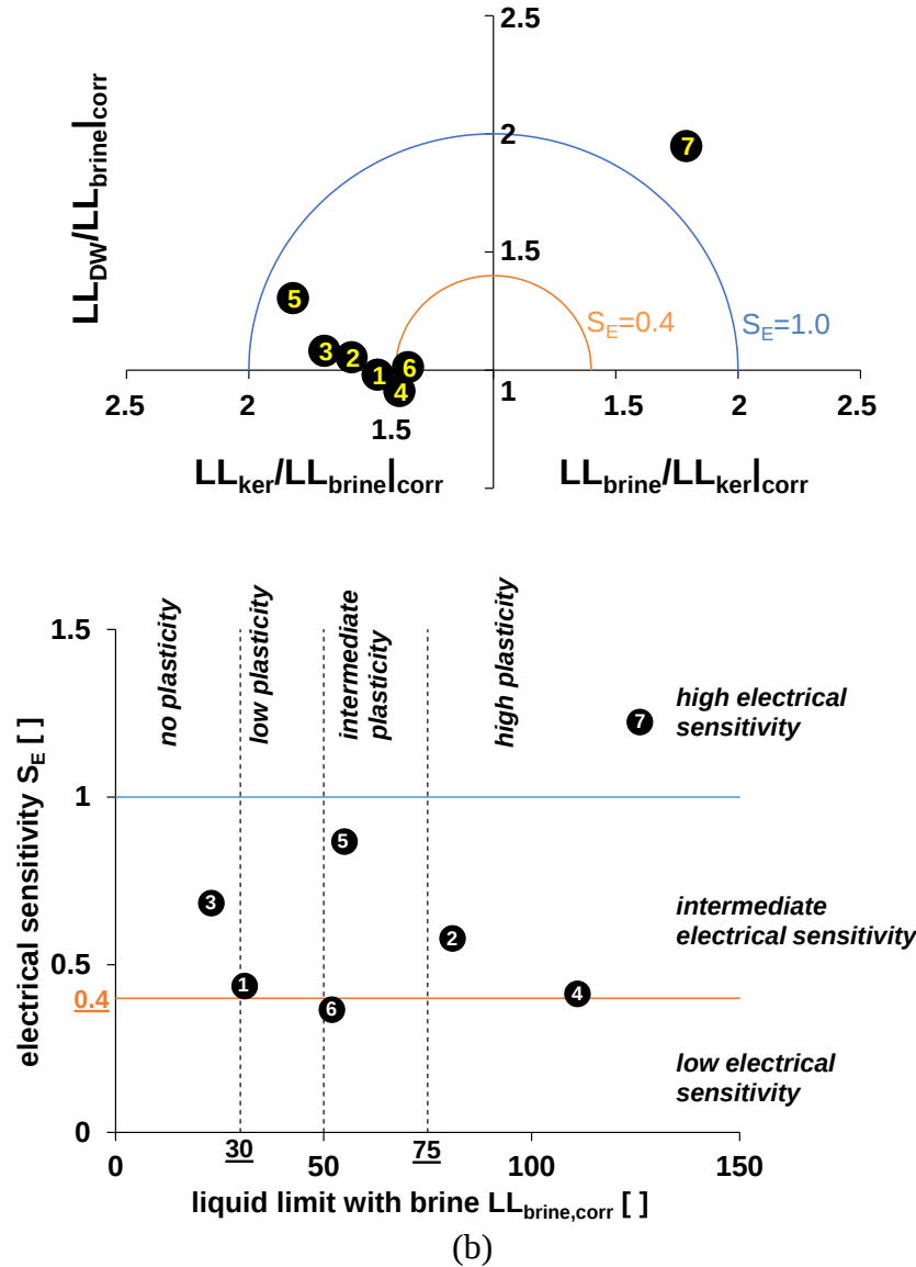
Figure 1. Charts for soil classification based on electrical sensitivity. Numbered black circles refer to the sediments in Tables 1 and 2. (a) Normalized liquid limit ratio of deionized water and kerosene to brine. The subscript corr refers to a correction for the salt mass in the brine and also for the low specific gravity of the kerosene (See Jang et al., 2018, Journal of Geophysical Research ). (b) Fines classification based on electrical sensitivity, S_E . See Jang et al., 2018, Journal of Geophysical Research for details on the corrections and S_E calculations.
