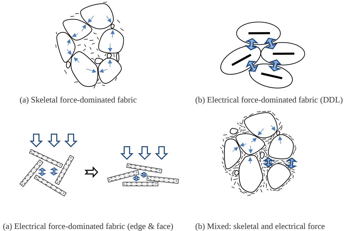
Figure 7. Fabric-based external stress transfer mechanisms. Larger grains are shown as irregular outlined shapes; electrically-sensitive clays are shown as dashes. (a) Skeletal-force dominated fabric, which can form during segregated sedimentation, experiences stress transfer (blue arrows) primarily through contacts between large grains such as silica silt in deionized water. (b) Electrical-force dominated fabric such as the bentonite (dashes) is controlled by DDL thickness (ellipsoids), and thus tends to be relatively compressible. (c) Electrical-force dominated fabric, such as kaolinite, can form high void fabric at low stress and in fresh water, but that fabric is compressible and will collapse under moderate stress. (d) Mixed fabric of skeletal (single-ended arrows) and electrical stress-transfer contacts (double-ended arrows), which can form during homogeneous sedimentation, such as silica silt in 2M-brine, will be more compressible than the purely skeletal force dominated sediment (Hueckel, 1992; Mitchell and Soga, 2005; Santamarina et al., 2001).
