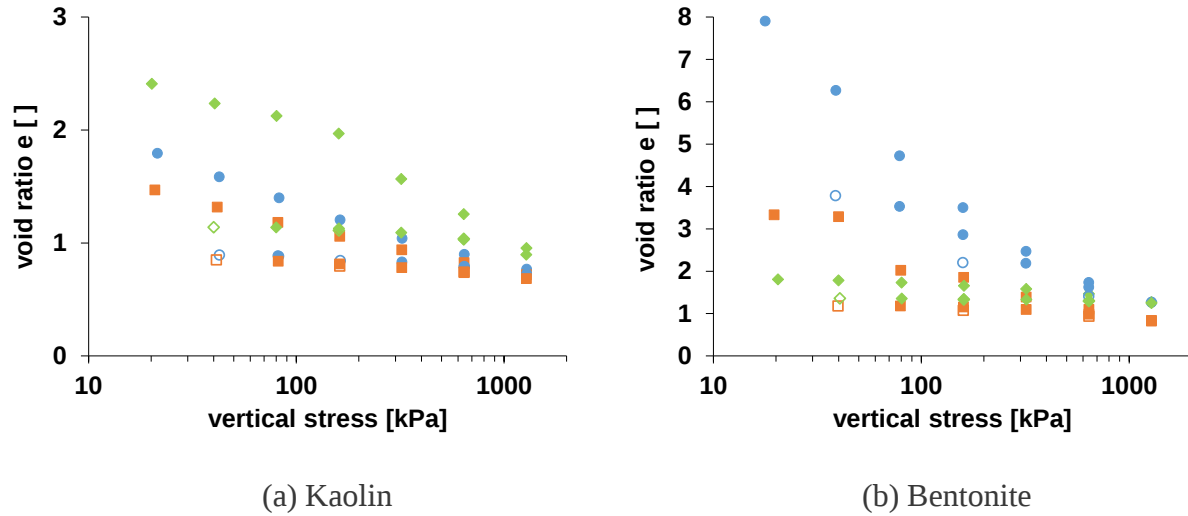
Figure 5. Consolidation results in deionized water (circle), 2M brine (square) and kerosene (diamond) for (a) kaolin and (b) bentonite. Solid symbols are loading and reloading steps, and the open symbols are unloading steps. As anticipated from Figures 2 and 4, the initial void ratio is higher for both types of fines in fresh water than in brine, with the difference being much more pronounced in bentonite. This is expected from the large difference in final sedimentation height for bentonite in fresh water and brine relative to kaolin in Figure 4.
