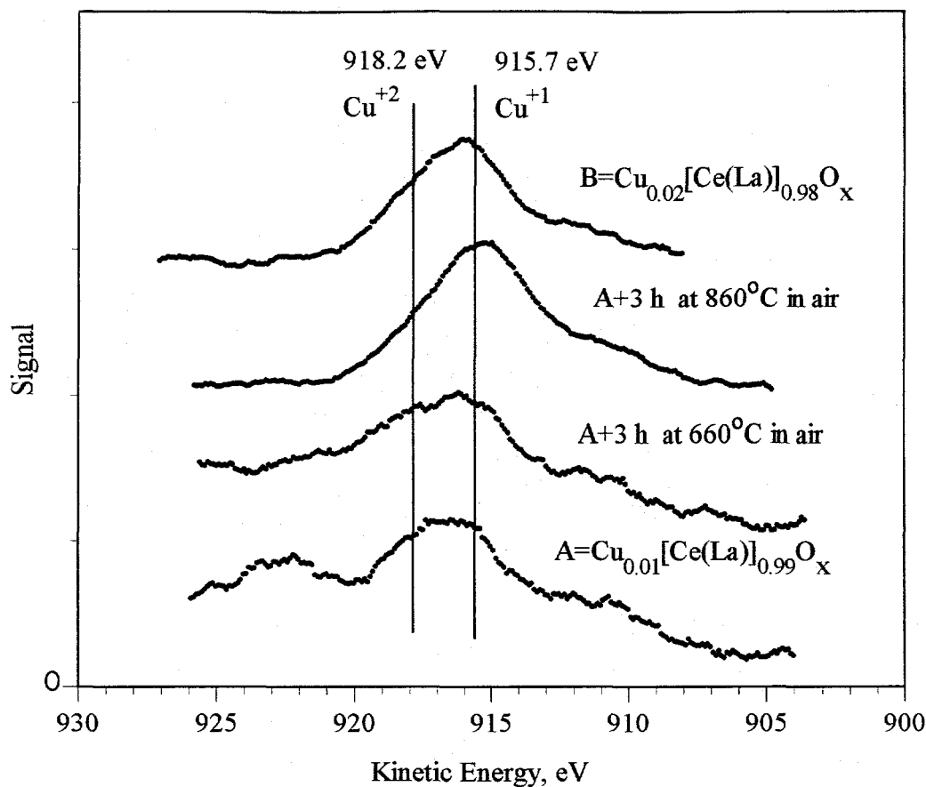
Figure 6.5b Kinetic Energy Spectra of the Auger \text{L}_{3\text{VV}} Electron of the \text{Cu}_{0.01}[\text{Ce}(\text{La})]_{0.99}\text{O}_x \text{Cu}_{0.02}[\text{Ce}(\text{La})]_{0.98}\text{O}_x Catalysts.
