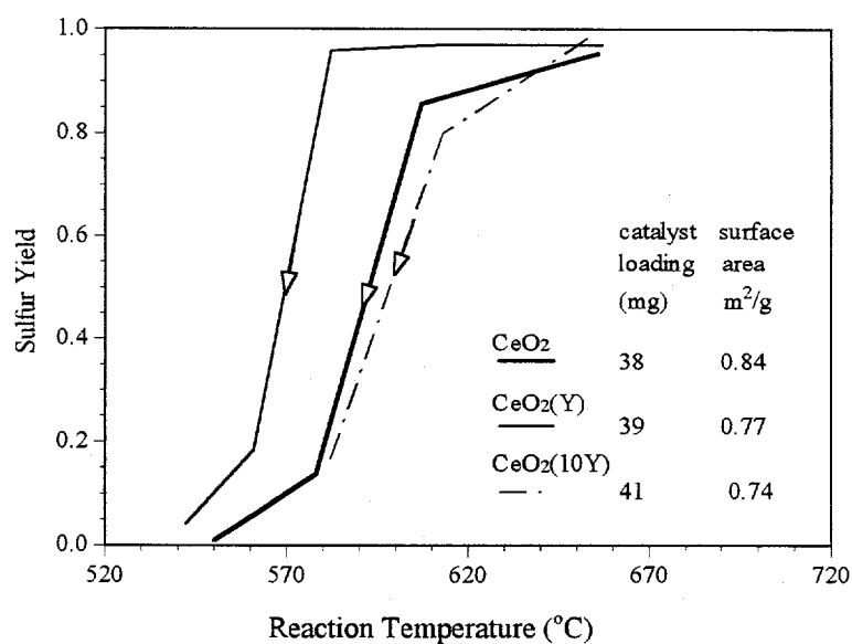
Figure 3.2 Effect of Y 2 O 3 Dopant Content in Ceria on Catalyst Activity ( [CO]/[SO_2]=2 ; 1% SO 2 , 0.012 s·g/cc(STP)).
