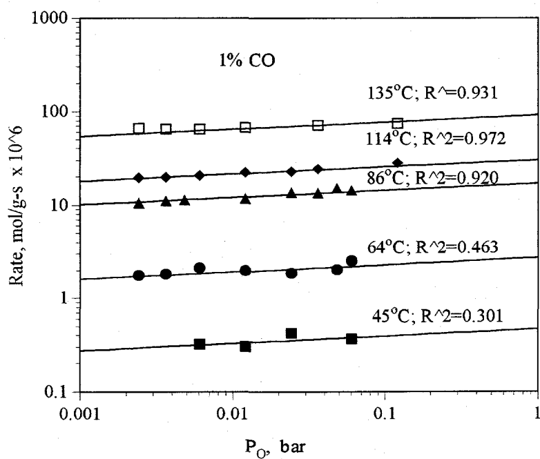
Figure 6.8 Variation of CO Oxidation Rate over the Cu_{0.15}[Ce(La)]_{0.85}O_x Catalyst with Partial Pressure of Oxygen under Constant P_{CO} .
