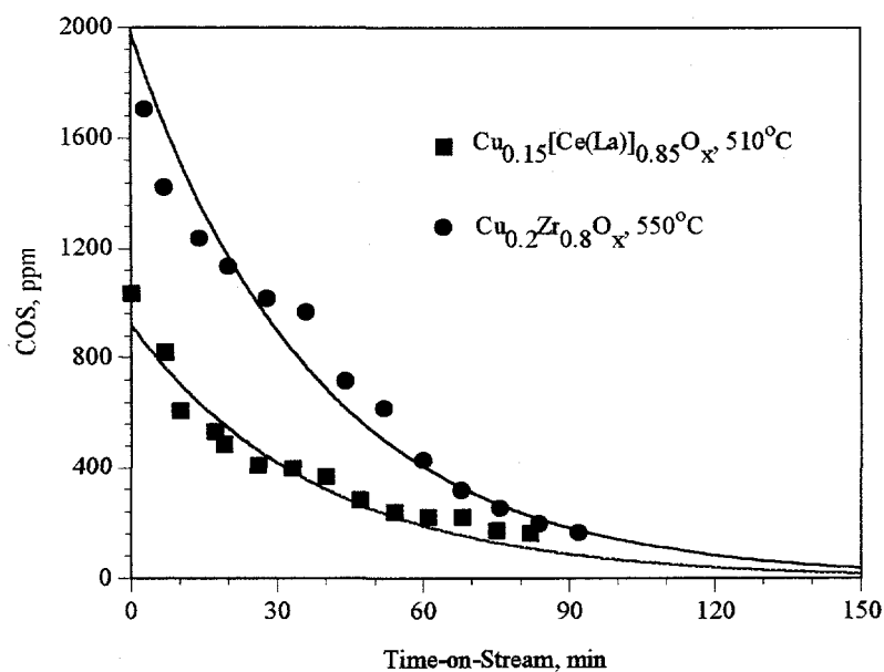
Figure 4.20 COS Evolution Profile During 2% \text{CO}/\text{He} Scavenging of Spent Catalysts.
