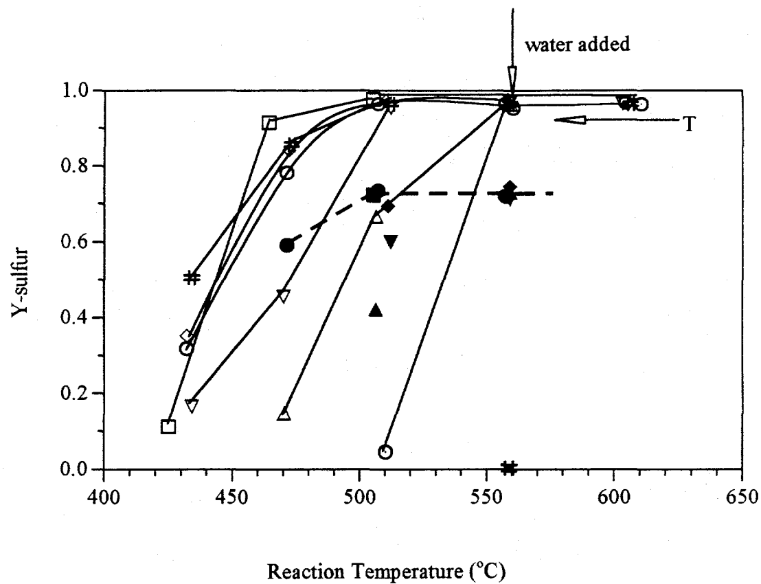
Figure 4.2 Fall-off Behavior and Water Vapor Effect on the Transition Metal-Impregnated Ceria Catalysts. \square = Cu/CeO 2 , \diamond = Ni/CeO 2 , \triangle = Pt/CeO 2 , \nabla = Mn/CeO 2 , \circ = Co/CeO 2 , \# = Cr/CeO 2 , \odot = CeO 2 . Unfilled symbols for dry gas (1% SO 2 , 2% CO, 97% He), The filled ones for wet gas (1% SO 2 , 2% CO, 2% H 2 O, 95% He).
