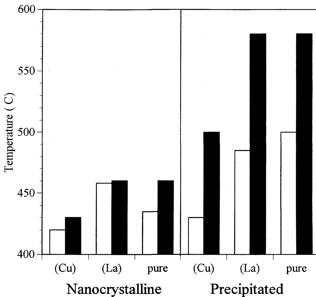
Figure 4.21 Light-off (filled bars) and fall-off (open bars) temperatures of precipitated and non-stoichiometric cerium oxide catalysts for SO 2 reduction by CO (1% SO 2 , 2% CO, 0.09s·g/cc).
