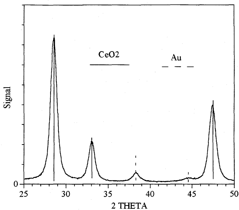
Figure 6.1a XRD Pattern of the \text{Au}_{0.05}[\text{Ce}(\text{La})]_{0.95}\text{O}_x Catalyst.
