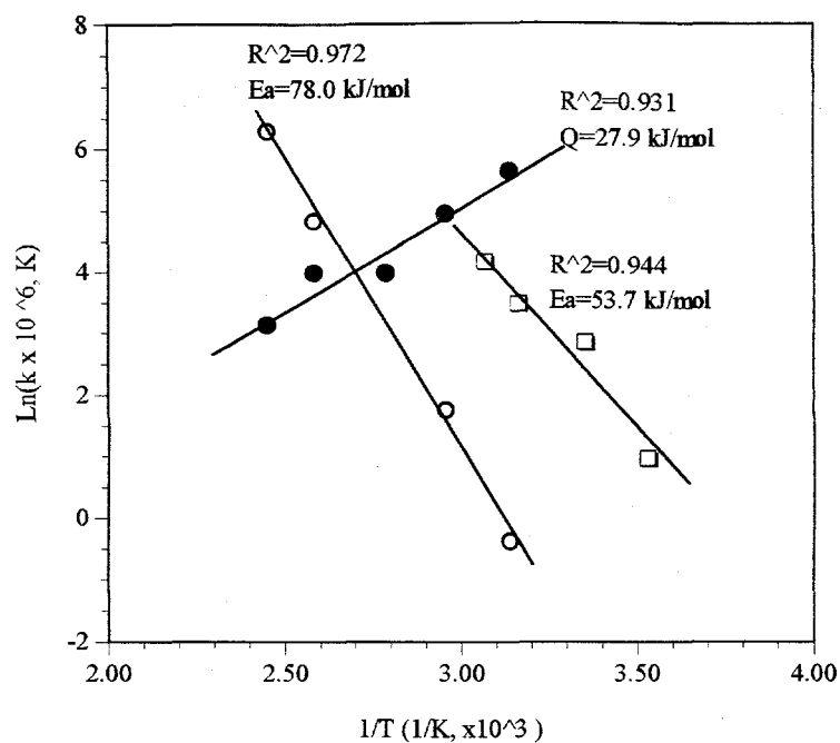
Figure 6.9 Arrhenius Plots of Constants k and K for CO Oxidation over \text{Au}_{0.05}[\text{Ce}(\text{La})]_{0.95}\text{O}_x and \text{Cu}_{0.15}[\text{Ce}(\text{La})]_{0.85}\text{O}_x Catalysts. \square k for \text{Au}_{0.05}[\text{Ce}(\text{La})]_{0.95}\text{O}_x , \circ k_{\text{CO}} for \text{Cu}_{0.15}[\text{Ce}(\text{La})]_{0.85}\text{O}_x , \bullet K_{\text{CO}} for \text{Cu}_{0.15}[\text{Ce}(\text{La})]_{0.85}\text{O}_x .
