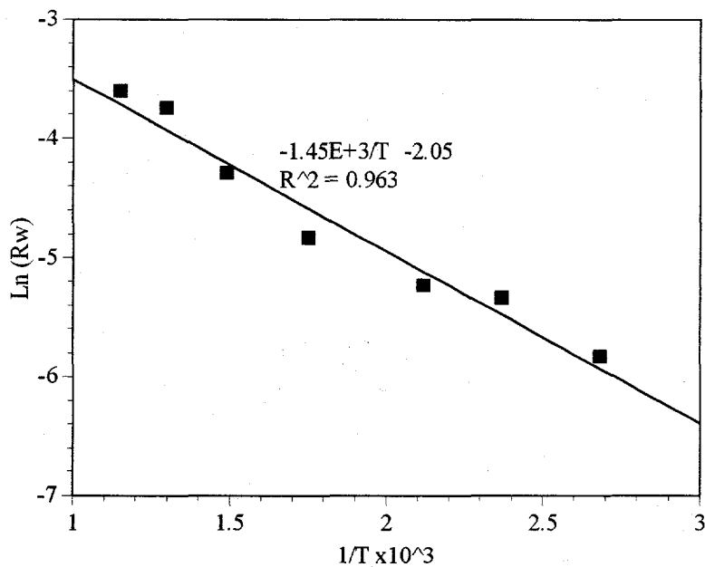
Figure 4.18 Arrhenius plot of the initial reduction rate of \text{Cu}_{0.15}[\text{Ce}(\text{La})]_{0.85}\text{O}_x catalyst by 0.5% \text{CO}/\text{N}_2 .
