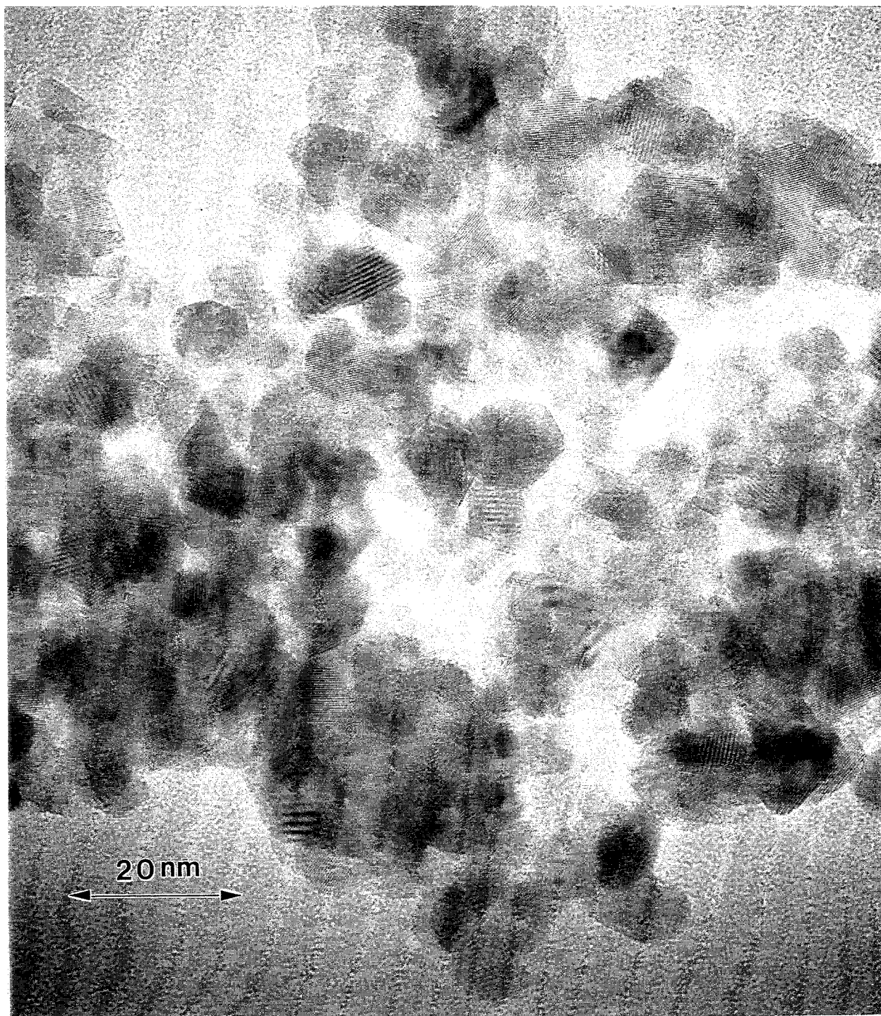
Figure 2.7 TEM Micrograph of 15 at.% CuO x /CeO 2 Catalyst.
