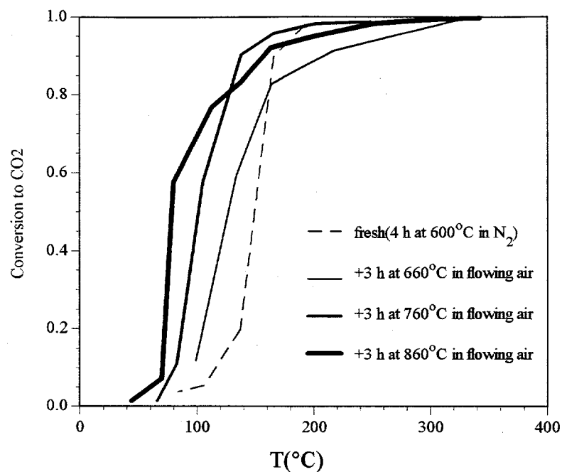
Figure 5.2 Effect of Thermal Treatment on the \text{Cu}_{0.01}[\text{Ce}(\text{La})]_{0.99}\text{O}_x Catalyst Activity for CO Oxidation (100 sccm: 2% CO, 16% O 2 ).
