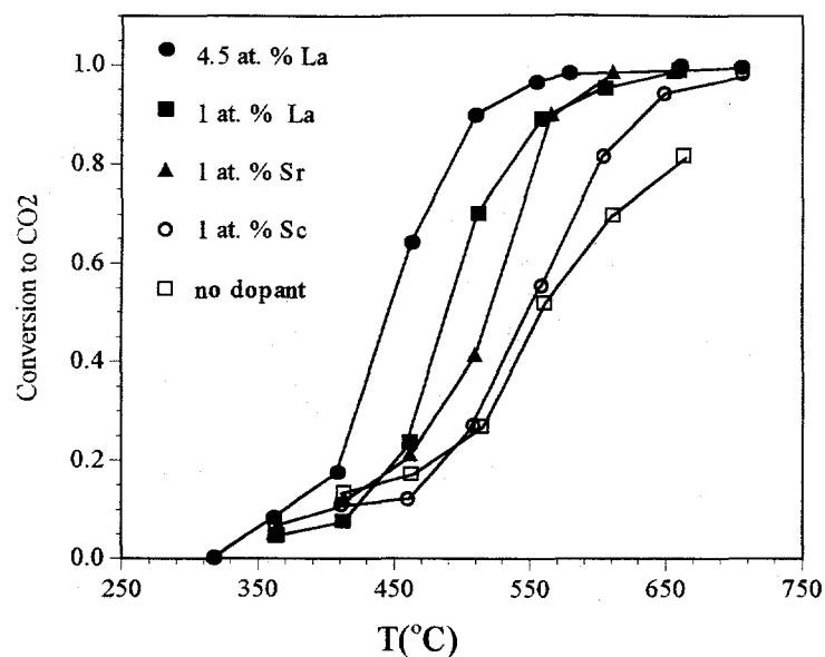
Figure 5.13 Effect of Dopant in the \text{Cu}_{0.15}\text{Ce}_{0.85}\text{O}_x Catalyst on Methane Oxidation Activity (0.09s-g/cc, 2 % \text{CH}_4 , 16 % \text{O}_2 ; catalyst surface area \approx 30 \text{ m}^2/\text{g} ).
