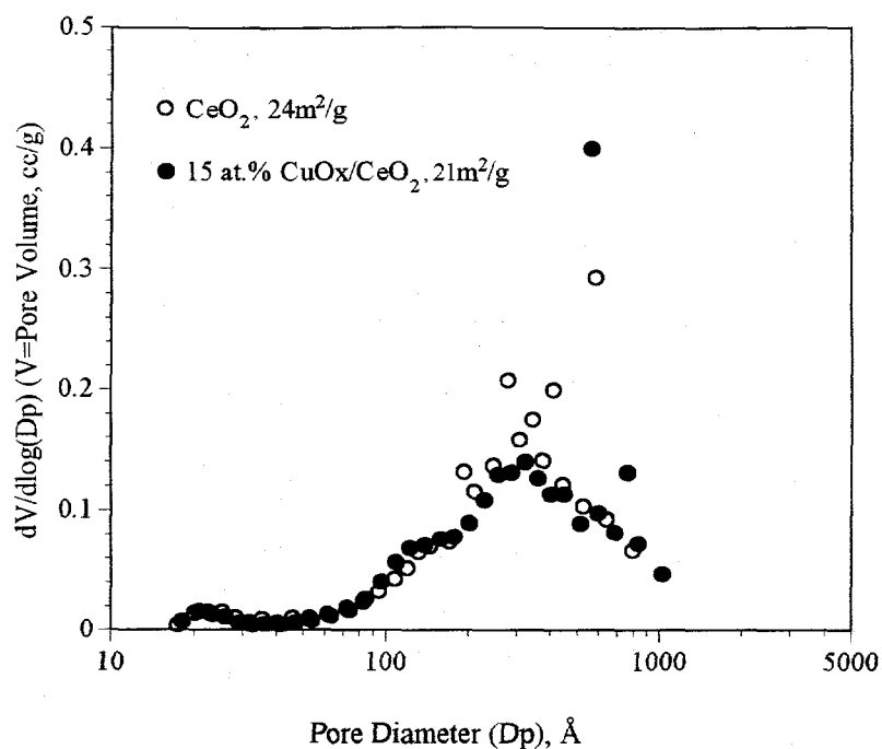
Figure 2.3 dV/d\log(D_p) Desorption Pore Volume Plots For \text{CeO}_2 Support and 15 at.% \text{CuOx}/\text{CeO}_2 .
