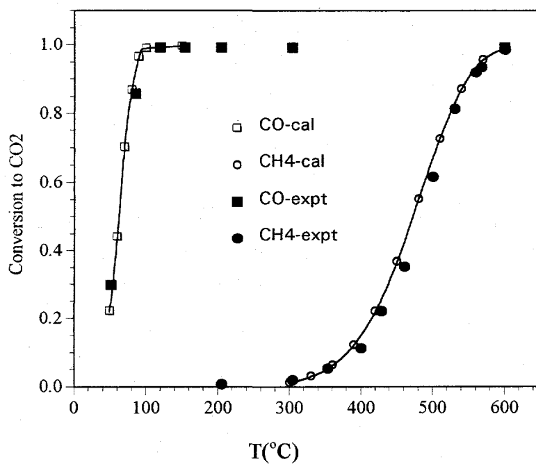
Figure 6.16 Comparison of Calculated Light-off Curves with Experimental Data ( \text{Cu}_{0.15}[\text{Ce}(\text{La})]_{0.85}\text{O}_x catalyst; 0.09 g-s/cc; 0.228% \text{CH}_4 , 0.1% \text{CO} , 1% \text{O}_2 ).
