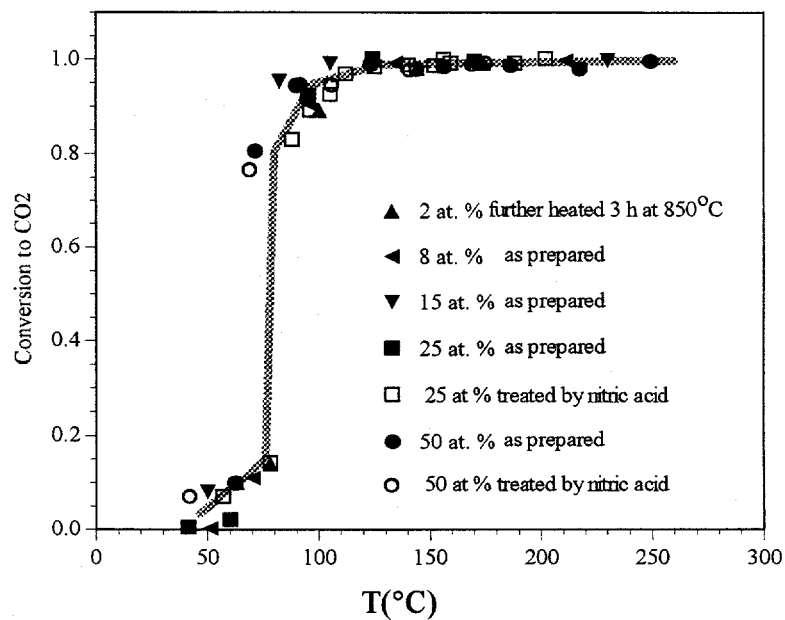
Figure 5.3 Effect of Bulk Copper Content in \text{Cu}_x[\text{Ce}(\text{La})]_{1-x}\text{O}_{2-x} Catalyst on CO Oxidation Activity (100 sccm: 2 % CO, 16 % O 2 ; surface areas \approx 30 \text{ m}^2/\text{g} ).
