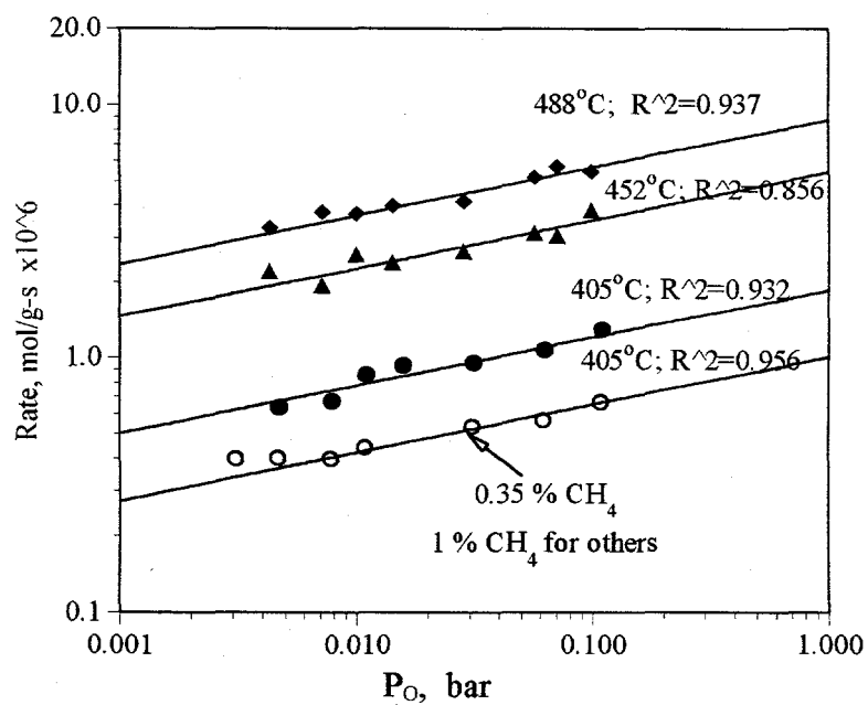
Figure 6.14 Variation of Methane Oxidation Rate over the \text{Cu}_{0.15}[\text{Ce(La)}]_{0.85}\text{O}_x Catalyst with Partial Pressure of Oxygen under Constant P_m .
