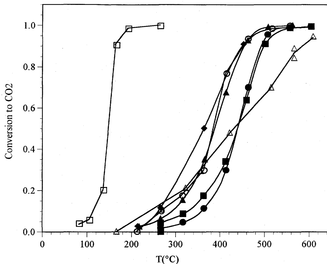
Figure 5.1 Light-off of CO Oxidation over Various 1 at.% Doped Ceria Catalysts and \text{Zr}_{0.9}\text{Y}_{0.1}\text{O}_{1.9} Catalyst (100 sccm: 2% CO, 16% O 2 ; surface areas: \text{Zr}_{0.9}\text{Y}_{0.1}\text{O}_{1.9} =42 m 2 /g, 1 at.% Cu= 57 m 2 /g, others \cong 28 m 2 /g). □ Cu-[Ce(La)]O 2 prepared by 4-h heating in N 2 at 600°C, ◆ La, ▲ Sr, ○ no dopant, ■ Sc, ● Gd, △ \text{Zr}_{0.9}\text{Y}_{0.1}\text{O}_{1.9} .
