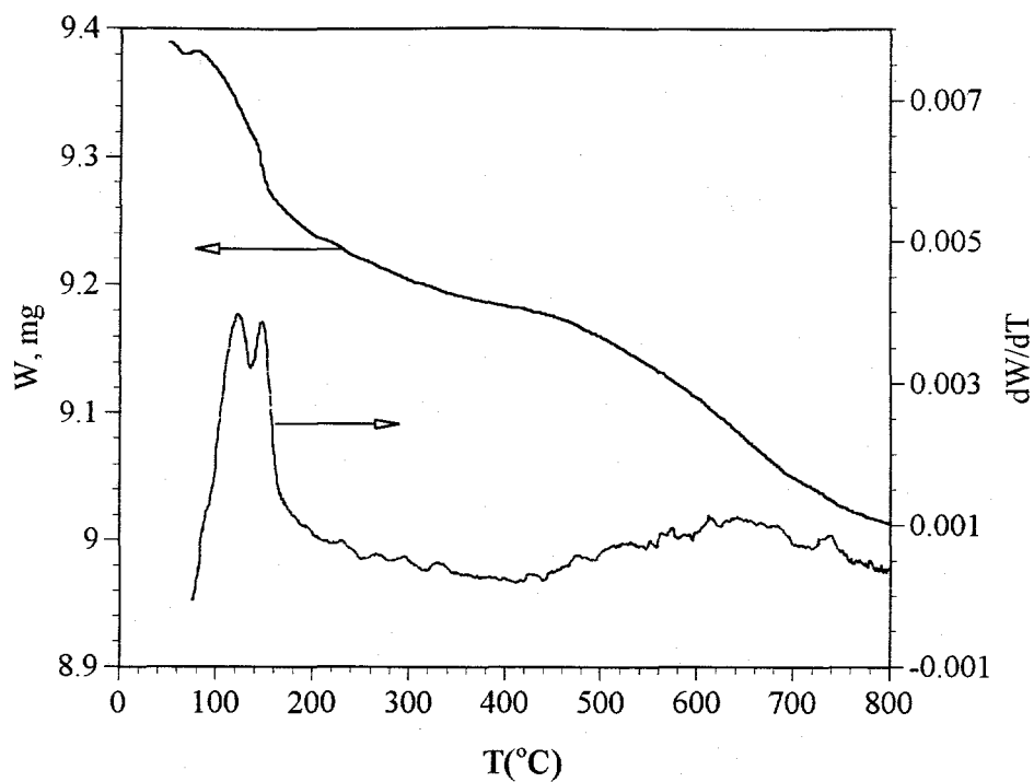
Figure 4.17 Temperature-programmed reduction profile of \text{Cu}_{0.15}[\text{Ce}(\text{La})]_{0.85}\text{O}_x catalyst by 3.5% \text{CO}/\text{N}_2 .
