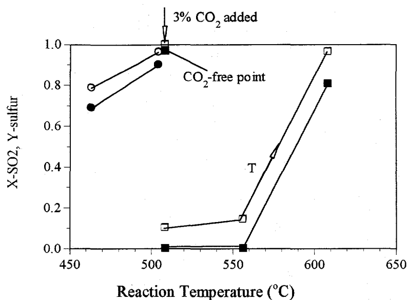
Figure 4.5 Effect of CO 2 on Catalyst Activity and Selectivity (1% SO 2 , 2% CO, 3% CO 2 , 94% He). \square = La 0.1 Ce 0.9 O 1.95 , \circ = Cu/CeO 2 . Unfilled symbols for X-SO 2 and the filled ones for Y-sulfur ( \blacksquare , \bullet ).
