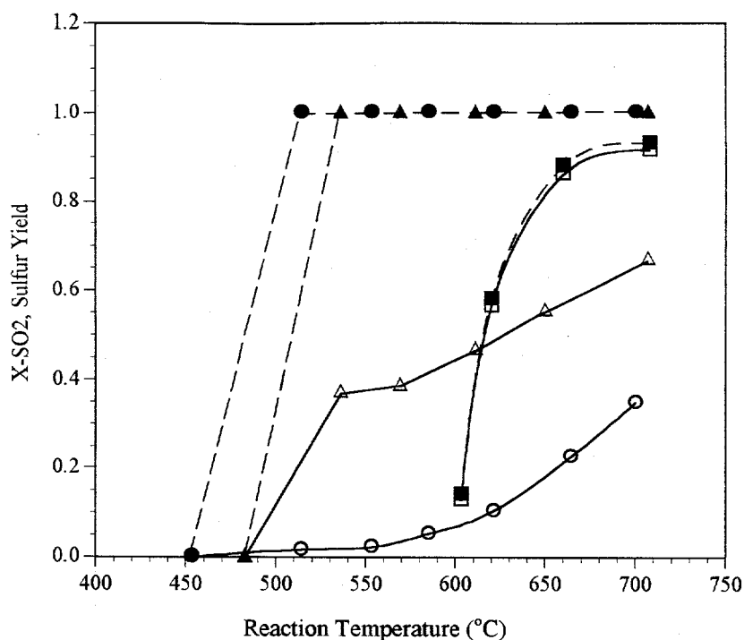
Figure 3.1 Elemental Sulfur Yield and SO 2 Conversion on Bulk CeO 2 Catalyst ( R_{CO}=[CO]/[SO_2] ; 1% SO 2 , 0.017s·g/cc(STP)). R_{CO}=4 : ○ ●; R_{CO}=3 : ▲ △; R_{CO}=1.9 : ■ □ (filled symbols for SO 2 conversion, unfilled ones for sulfur yield).
