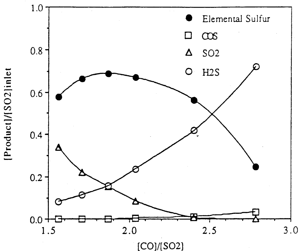
Figure 3.9 Product Distribution with the [CO]/[SO 2 ] Ratio on CeO 2 (La) Catalyst in the Presence of Water Vapor at 610°C (1% SO 2 , 1.5% H 2 O; 0.043s·g/cc).
