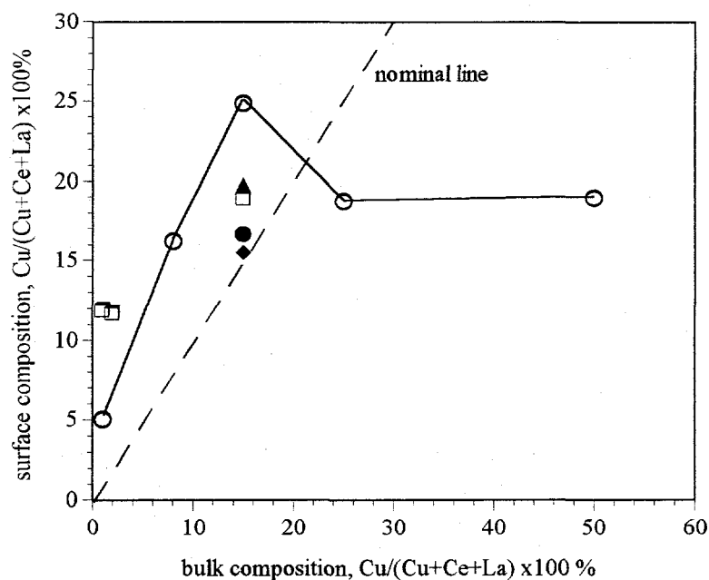
Figure 6.12 Variation of the Surface Copper Fraction of the Cu-Ce(La)-O Catalyst with Bulk Composition and Thermal Treatment. \circ as prepared by 4-h calcination at 650^{\circ}C in air, \square further heated for 3 h in flowing air at 860^{\circ}C , \blacktriangle reduced by 25% H_2/He for 2 h at 300^{\circ}C , \blacklozenge reduced by 25% H_2/He for 1 h at 600^{\circ}C , \bullet prepared by impregnation.
