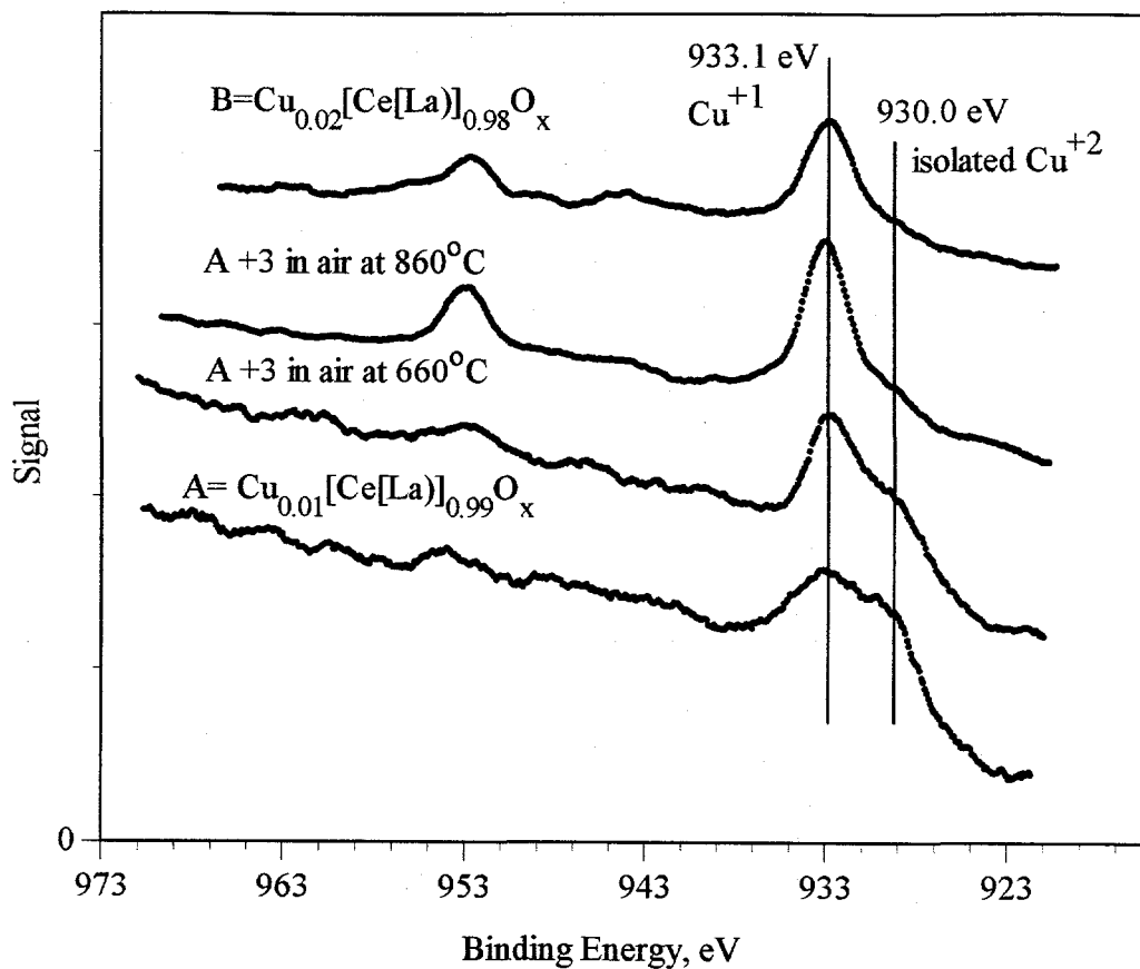
Figure 6.5a \text{Cu}2\text{p} XP Spectra of \text{Cu}_{0.01}[\text{Ce}(\text{La})]_{0.99}\text{O}_x and \text{Cu}_{0.02}[\text{Ce}(\text{La})]_{0.98}\text{O}_x Catalysts ( \text{Cu}_{0.01}[\text{Ce}(\text{La})]_{0.99}\text{O}_x prepared by 4 h calcination in \text{N}_2 at 600^\circ\text{C} ; \text{Cu}_{0.02}[\text{Ce}(\text{La})]_{0.98}\text{O}_x prepared by 4-h calcination at 650^\circ\text{C} and 3-h calcination at 860^\circ\text{C} both in air).
