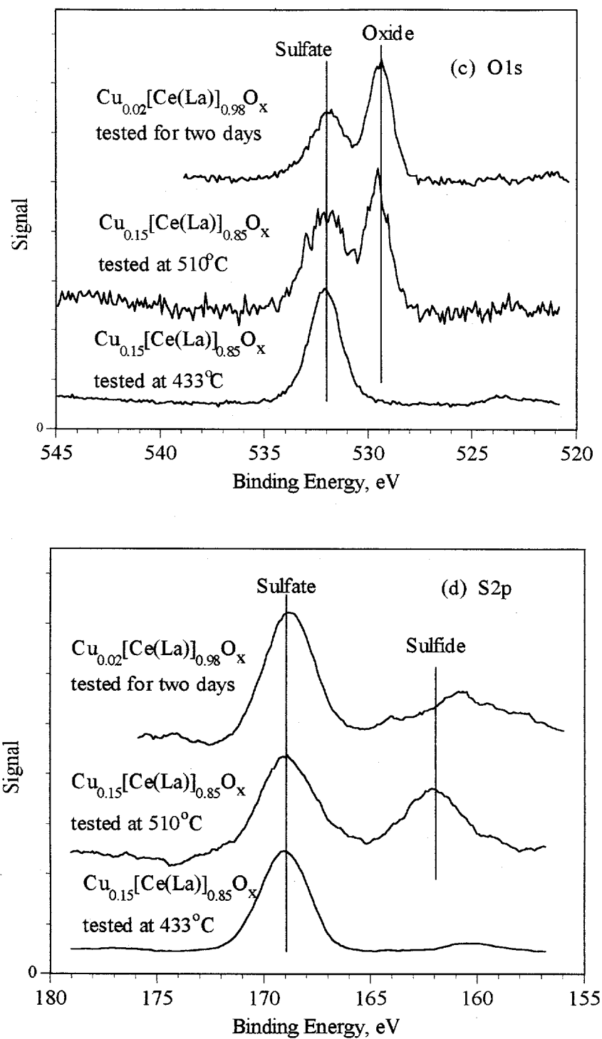
Figure 4.16 XPS of the Cu-Ce(La)-O catalyst used for SO 2 and CO reaction.
