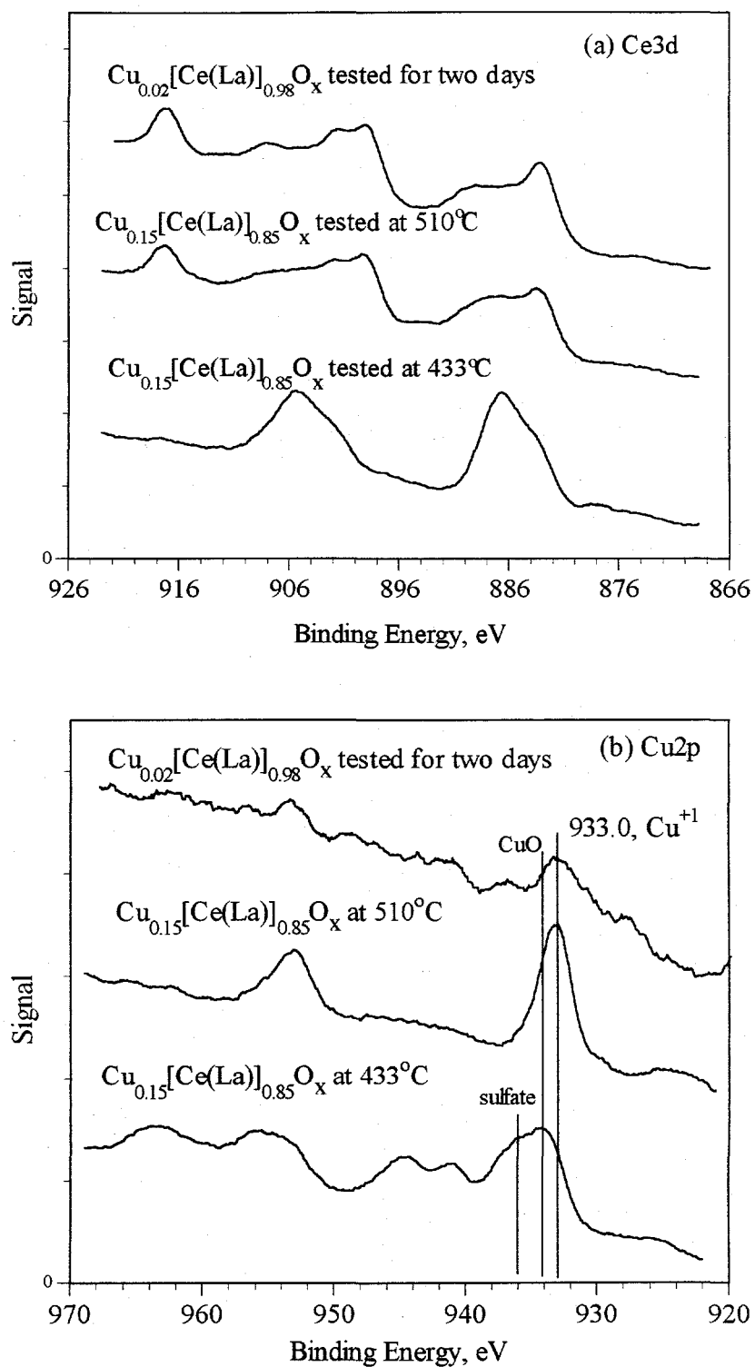
Figure 4.16 XPS of the Cu-Ce(La)-O catalyst used for SO 2 and CO reaction.
