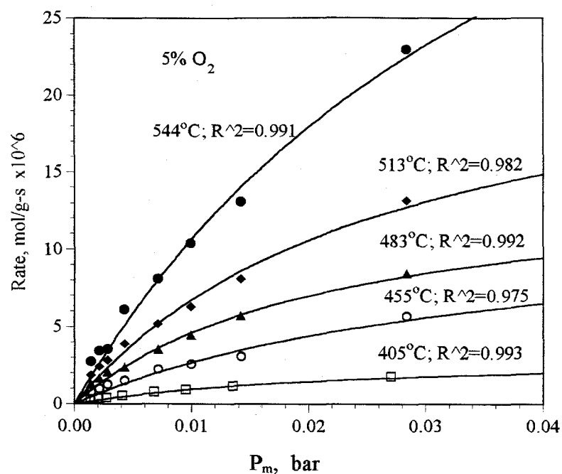
Figure 6.13 Variation of Methane Oxidation Rate over the \text{Cu}_{0.15}[\text{Ce(La)}]_{0.85}\text{O}_x Catalyst with Partial Pressure of Methane under Constant P_{\text{O}_2} .
