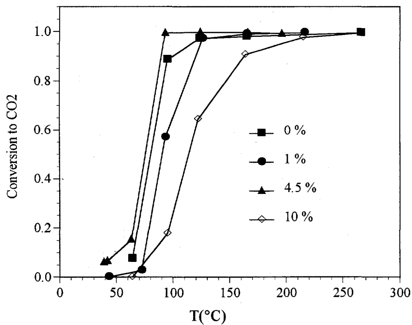
Figure 5.6 Effect of La Dopant Content on the CO Oxidation Activity of \text{Cu}_{0.15}\text{Ce}_{0.85}\text{O}_x Catalyst (100 sccm: 2 % CO, 16 % \text{O}_2 ; surface areas \approx 30 \text{ m}^2/\text{g} ).
