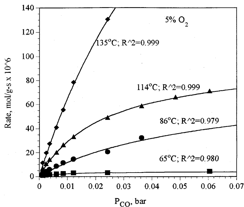
Figure 6.7 Variation of CO Oxidation Rate over the Cu_{0.15}[Ce(La)]_{0.85}O_x Catalyst with Partial Pressure of CO under Constant P_{O_2} .
