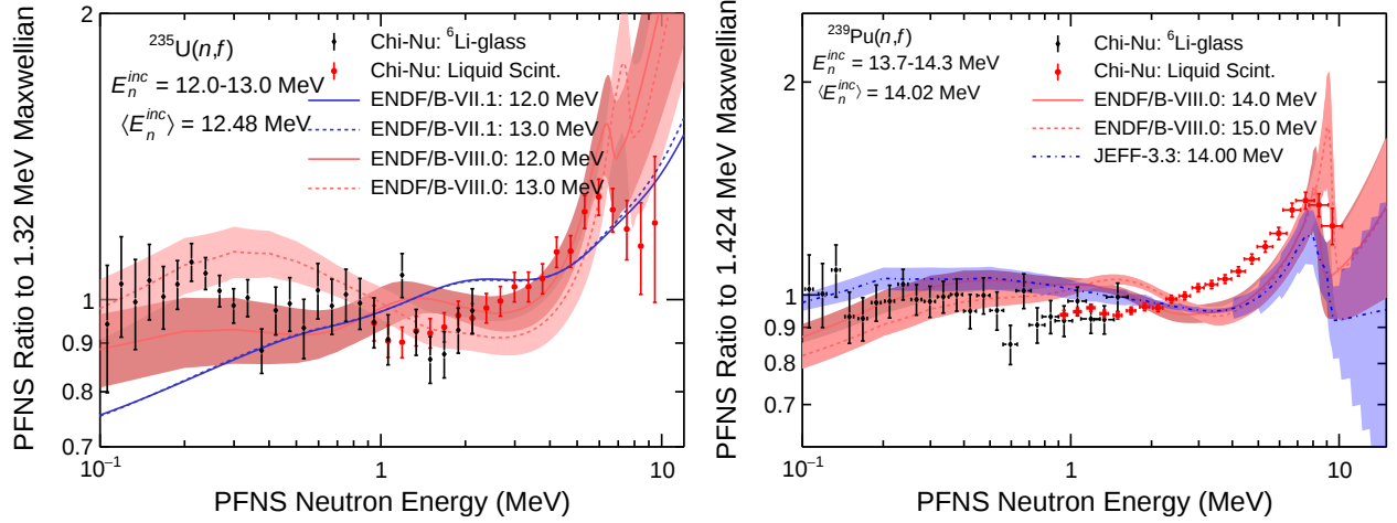
Figure 3. Third-chance fission and pre-equilibrium PFNS features observed by the Chi-Nu experiment for neutron-induced fission of ^{235}\text{U} (left) and ^{239}\text{Pu} (right) are shown here. The bands and trends correspond to evaluations at relevant incident neutron energies [11–13].
