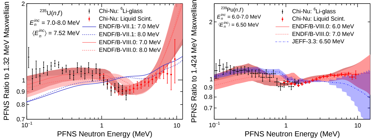
Figure 2. Second-chance fission PFNS features observed by the Chi-Nu experiment for neutron-induced fission of ^{235}\text{U} (left) and ^{239}\text{Pu} (right) are shown here. The experimental incident neutron-energy ranges are shown in each plot. The bands and trends correspond to evaluations at relevant incident neutron energies [11–13].
