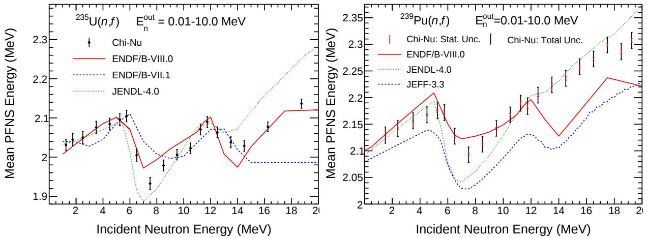
Figure 4. The trend of the average PFNS energy, \langle E \rangle , as a function E_n^{\text{inc}} is shown here for ^{235}\text{U} and ^{239}\text{Pu} in the left and right panels, respectively. Relevant evaluations are plotted as well for comparison. The ^{239}\text{Pu} \langle E \rangle uncertainties are also subdivided into statistical and systematic components to demonstrate the importance of identifying and quantifying all possible sources of systematic uncertainty. The ^{235}\text{U} only has a subset of the total known systematic uncertainty applied for the data in this proceedings.
