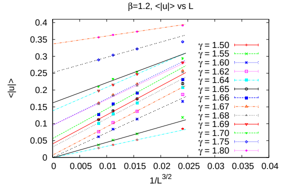
FIG. 7. Same as Fig. 4 at \beta = 1.2 . Instead of a sharp discontinuity at the transition, the order parameter appears to increase smoothly away from zero, somewhere in the neighborhood of \gamma \approx 1.62 . This is reminiscent of a continuous transition, although there is in fact no thermodynamic transition, or even a rapid crossover, at this point.
