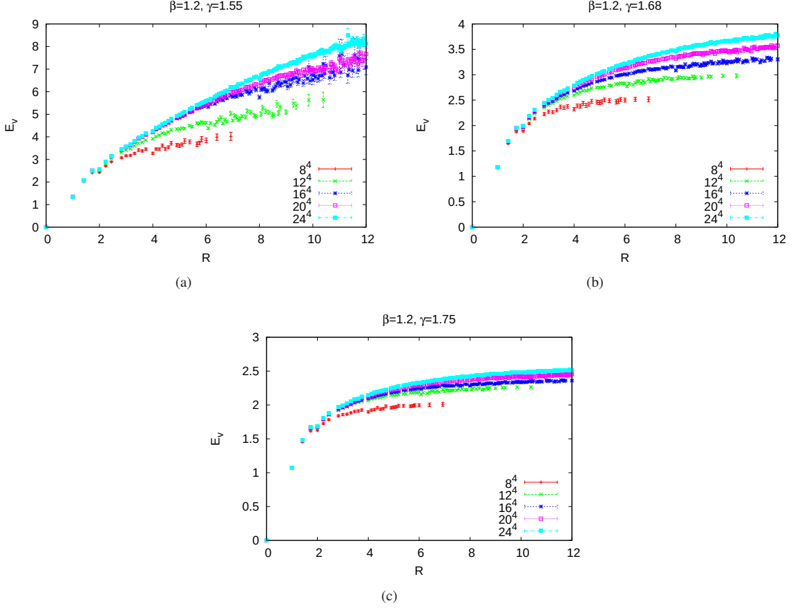
FIG. 8. E_V(R) vs. R for the Dirac states in the gauge-Higgs model, as in Fig. 3, but this time at \beta = 1.2 . (a) below the (continuous) remnant symmetry breaking transition at \gamma = 1.55 ; (b) close to, but slightly above the transition, at \gamma = 1.68 ; (c) above the transition at \gamma = 1.75 .
