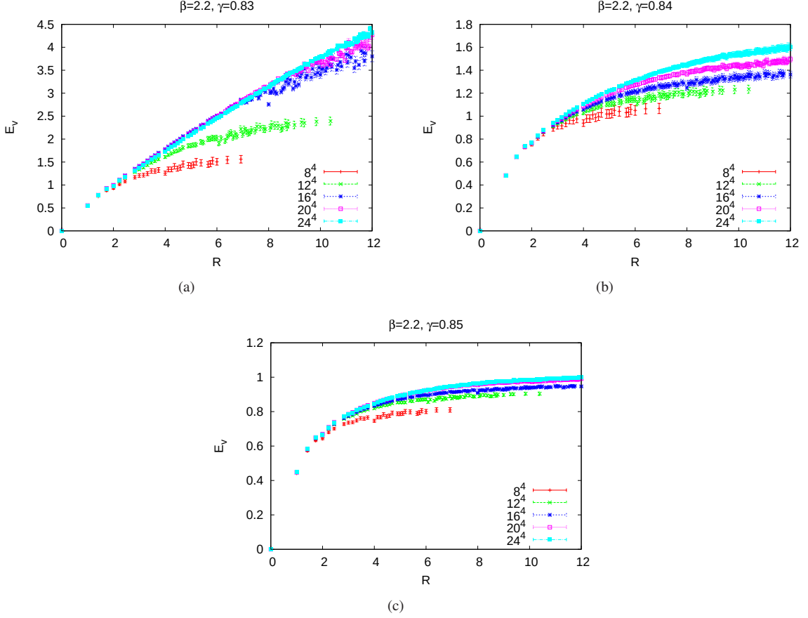
FIG. 3. E_V(R) vs. R for the Dirac states in the gauge-Higgs model at \beta = 2.2 . (a) just below the remnant symmetry breaking transition at \gamma = 0.83 ; (b) very close to the transition, at \gamma = 0.84 ; (c) just above the transition at \gamma = 0.85 .
