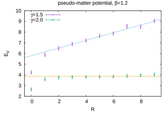
FIG. 10. The energy E_V(R) defined in (22) vs. R for pseudo-matter states in the gauge-Higgs model at \beta = 1.2 , compared at \gamma = 1.5 (confining region) and \gamma = 2.0 (Higgs region), and computed on a 20^4 lattice volume. The straight lines are best fits of the data at R \geq 2 to a linear rise ( \gamma = 1.5 ) and a constant ( \gamma = 2.0 ).
