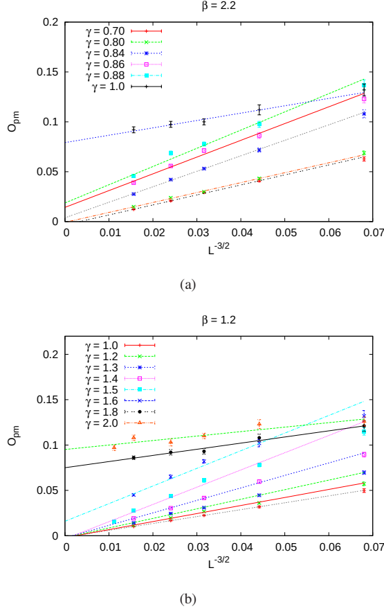
FIG. 9. The pseudo-matter order parameter O_{pm}^L , defined in (28) at (a) \beta = 2.2 , and (b) \beta = 1.2 , plotted vs. the inverse square root of the spatial volume L^{-3/2} , at a set of \gamma values. In both cases the order parameter reliably extrapolates to a positive value only at the higher \gamma values.
