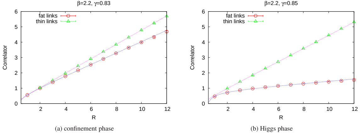
FIG. 11. E_V(R) vs. R for states created by Wilson line operators in the gauge-Higgs model at \beta = 2.2 . The figure compares Wilson line operators obtained from unmodified (“thin”) link variables and “fat” link variables. (a) just below the crossover transition in the “confinement phase,” at \gamma = 0.83 ; (b) just above the transition at \gamma = 0.85 . These operators, in contrast to the Dirac and pseudo-matter operators, do not detect the loss of S_c -confinement above the transition, since even in the Higgs region the energies rise linearly. But S_c -confinement requires that all V operators, not just some operators, satisfy the S_c -confinement condition, as explained in the text, otherwise the system is in the C-confinement phase.
