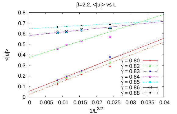
FIG. 4. The remnant symmetry order parameter \langle |u| \rangle at \beta = 2.2 vs. the inverse square root of 3-volume, L^{-3/2} . A rough extrapolation to the infinite volume limit is made by fitting a straight line to the three largest volume data points. Note the sudden jump in the extrapolated value between \gamma = 0.82 and \gamma = 0.84 , indicating the breaking of the remnant gauge symmetry.
