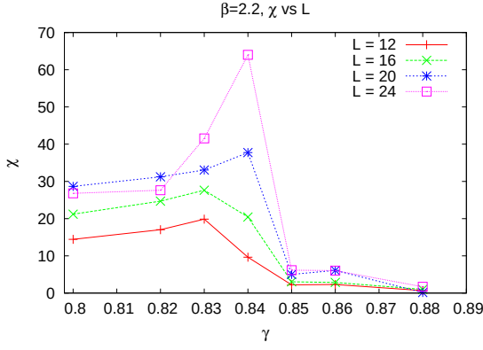
FIG. 5. Susceptibility \chi vs. \gamma in the |u| order parameter at \beta = 2.2 , at various lattice volumes of extension L . The sharp peak at \gamma = 0.84 corresponds to the remnant symmetry-breaking transition.
