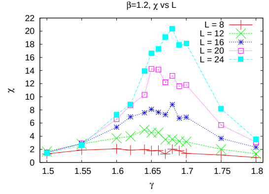
FIG. 6. Same as Fig. 5, at \beta = 1.2 . The peak in the susceptibility is much broader (by an order of magnitude) than the corresponding peak at \beta = 2.2 .
