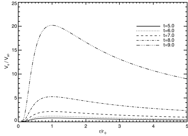
Figure 1. The normalized toroidal velocity v_\phi/v_{\phi 0} (see equation (13)) as a function of dimensionless radius r/r_0 . For this case \alpha/\gamma=0.1 and \gamma=0.41 .
