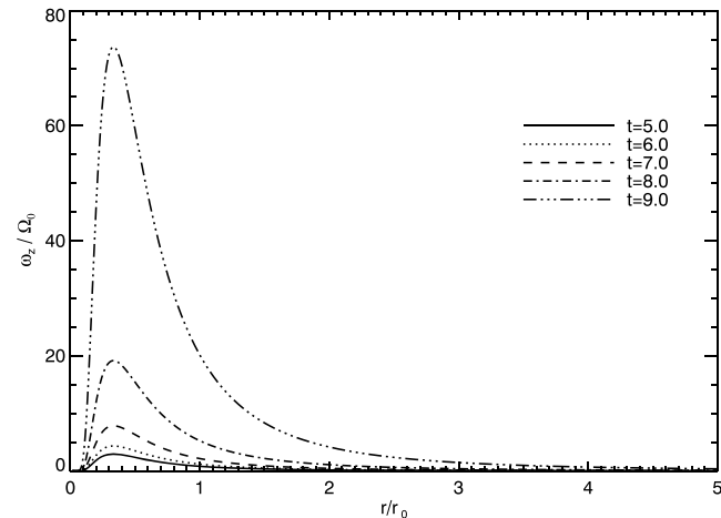
Figure 2. The normalized vertical component of vorticity \omega_z/\Omega_0 (see equation (13)) as a function of radius r/r_0 . For this case \alpha/\gamma is equal 0.1 and \gamma=0.41 , respectively.
