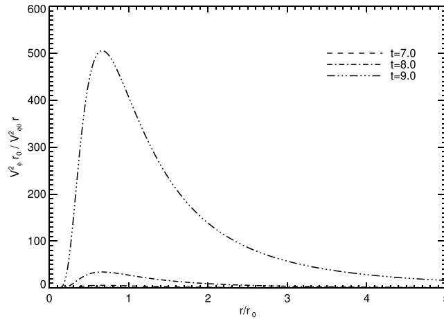
Figure 3. The normalized value of r_0 v_\phi^2 / v_{\phi 0}^2 r as a function of r/r_0 . Here \alpha/\gamma is equal 0.1. The values of r_0 v_\phi^2 / v_{\phi 0}^2 r for t=5.0 and 6.0 are small and not shown on the plot.
