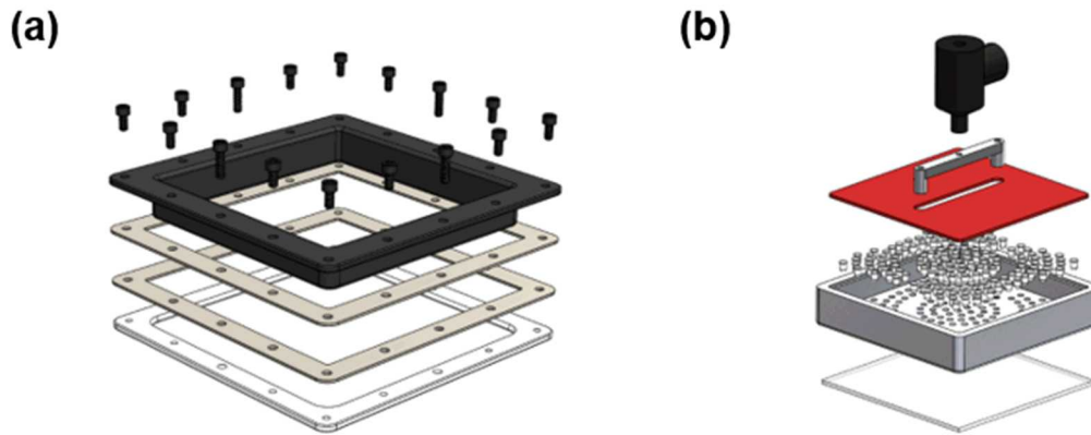
Figure 2: Digital renderings of the custom-designed parts, including (a) the stretched film resin tray and (b) the UV-backlit build plate.
