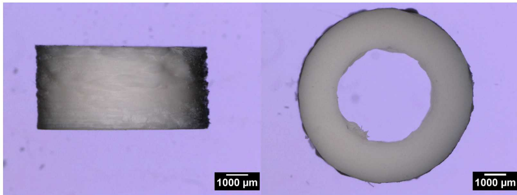
Figure 4. Side view and top view of an alumina ring structure printed with A16 alumina after sintering.
