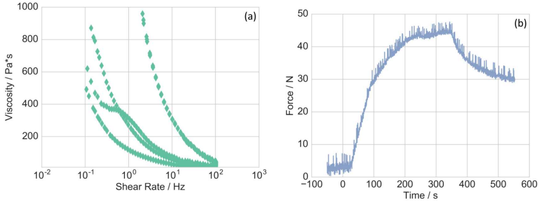
Figure 2. (a) Viscosity vs. shear rate of 81.5 wt% A15 in Genesis. Three sequential (b) Force curve for this paste with a constant dispensing rate with showing three distinct regions corresponding to onset, steady-state, and decay to idle force after dispensing is stopped at 350 seconds.
