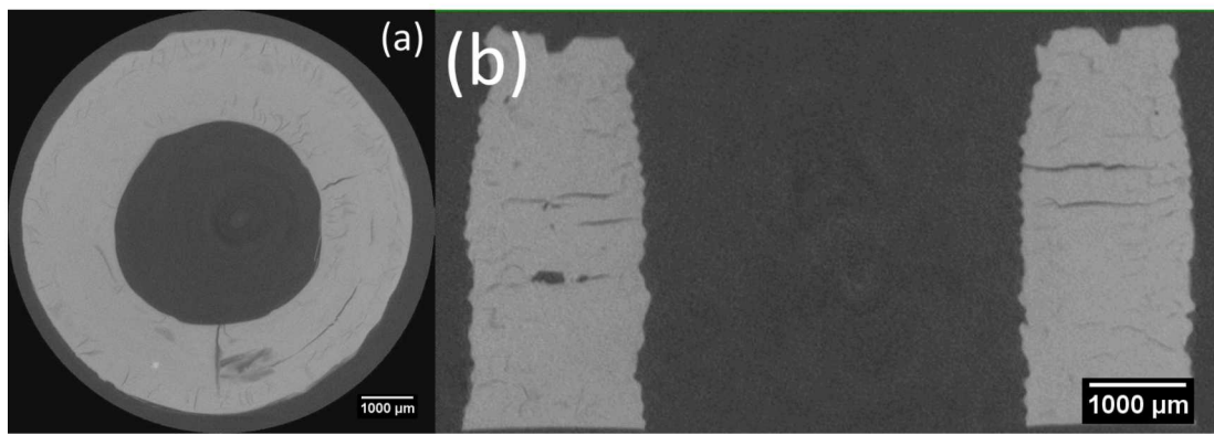
Figure 6. X-ray computed tomography of an Al6 ring structure. (a) Cross section through a ring structure in the X-Y plane and (b) cross section through a ring structure in the X-Z plane.
