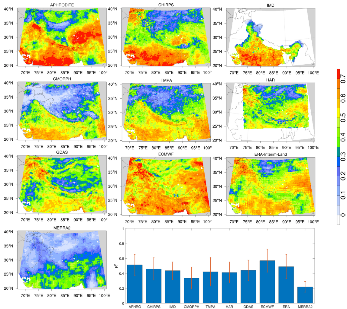
FIGURE 7 | Same as Figure 6, but for r^2 .
