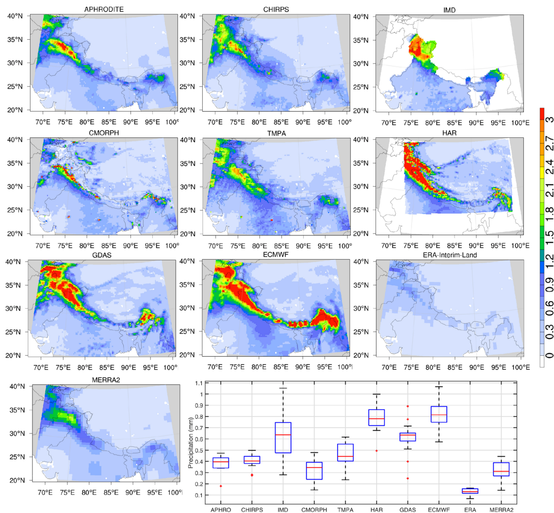
FIGURE 4 | Same as Figure 2 , but stratified for the peak winter months (December, January, February). The extreme data points/outliers are plotted individually using the “+” symbol.
