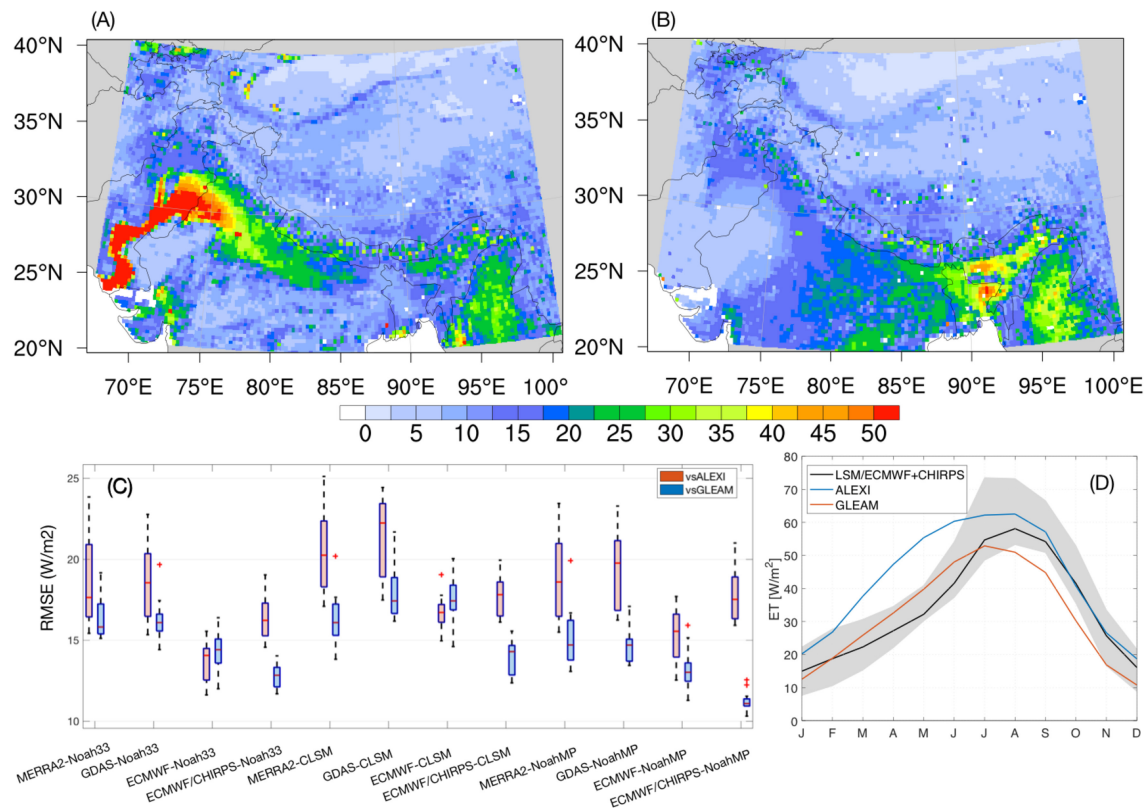
FIGURE 11 | Maps of ensemble mean RMSE ( W/m^2 ) of ET across the 12 ensemble members compared against ALEXI (A) and GLEAM (B), distribution of the domain-averaged RMSE from each of the 12 LSM runs (C) and the mean seasonal cycle of ET (D). The gray shading in (D) represents the spread in ET across the LSMs.
