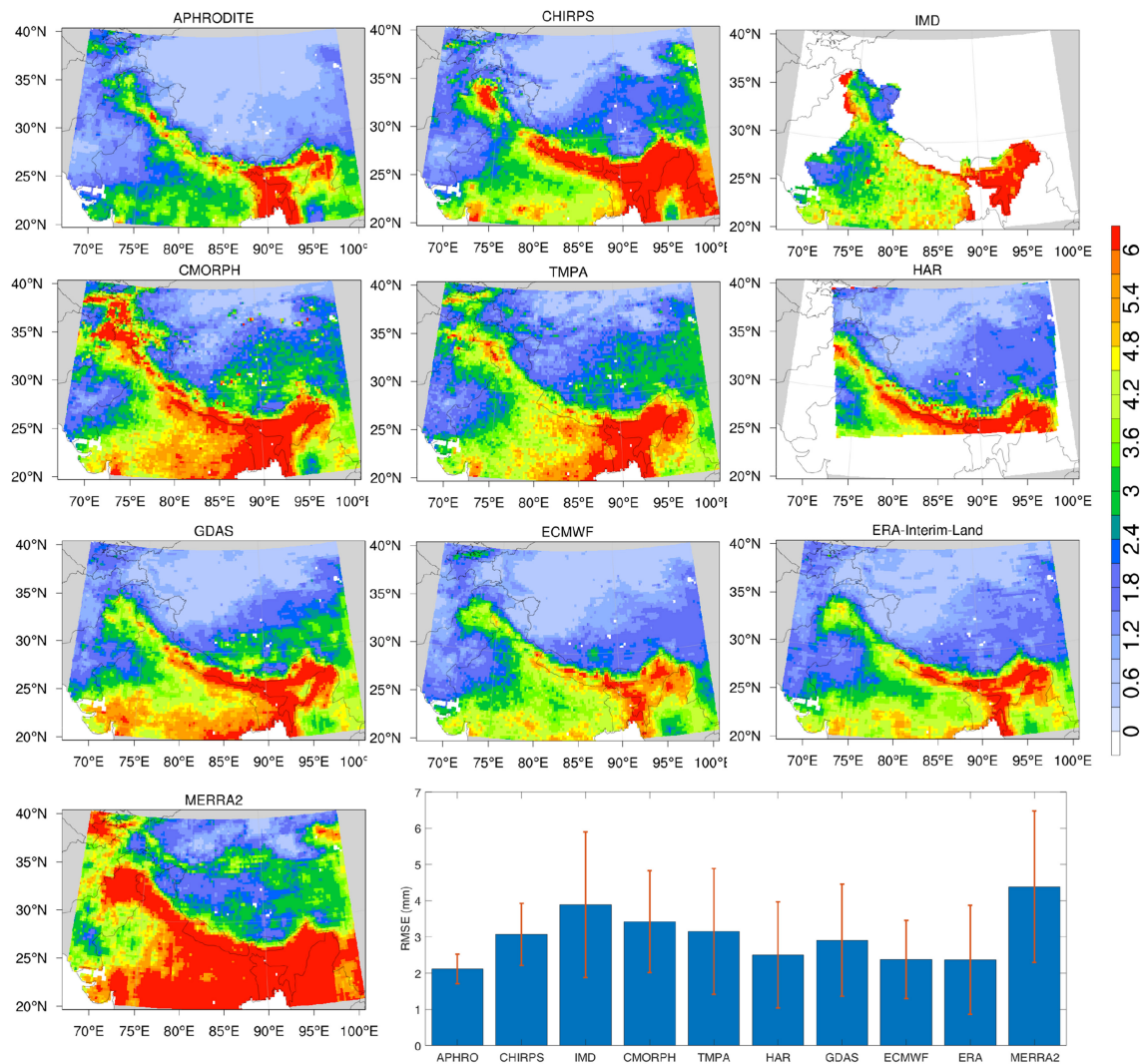
FIGURE 6 | RMSE of precipitation (mm) estimated using the ETC method. The value at each grid point represents the mean RMSE across 120 possible triplets among the 10 precipitation products. The error bars represent the mean standard deviation across the 120 triplets.
