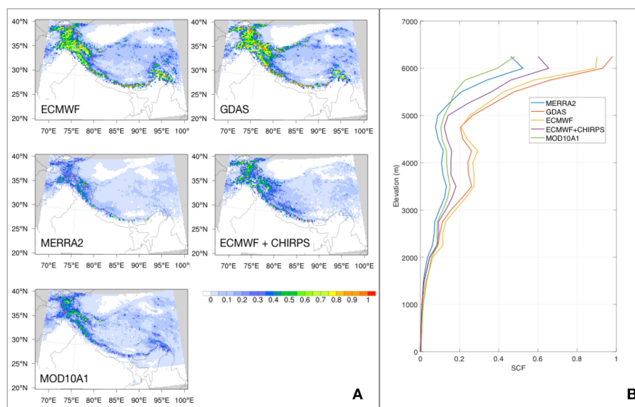
FIGURE 12 | Comparison of mean SCF estimates (unitless) from MOD10A1 and the model runs. (A) Shows the spatial maps of mean SCF whereas (B) shows the domain-averaged SCF stratified by elevation. The modeled estimates are averaged across the three LSMs for each forcing data.
