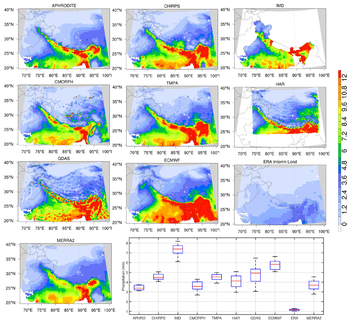
FIGURE 5 | Same as Figure 2 , but stratified for the summer months (June, July, August). The extreme data points/outliers are plotted individually using the "+" symbol.
