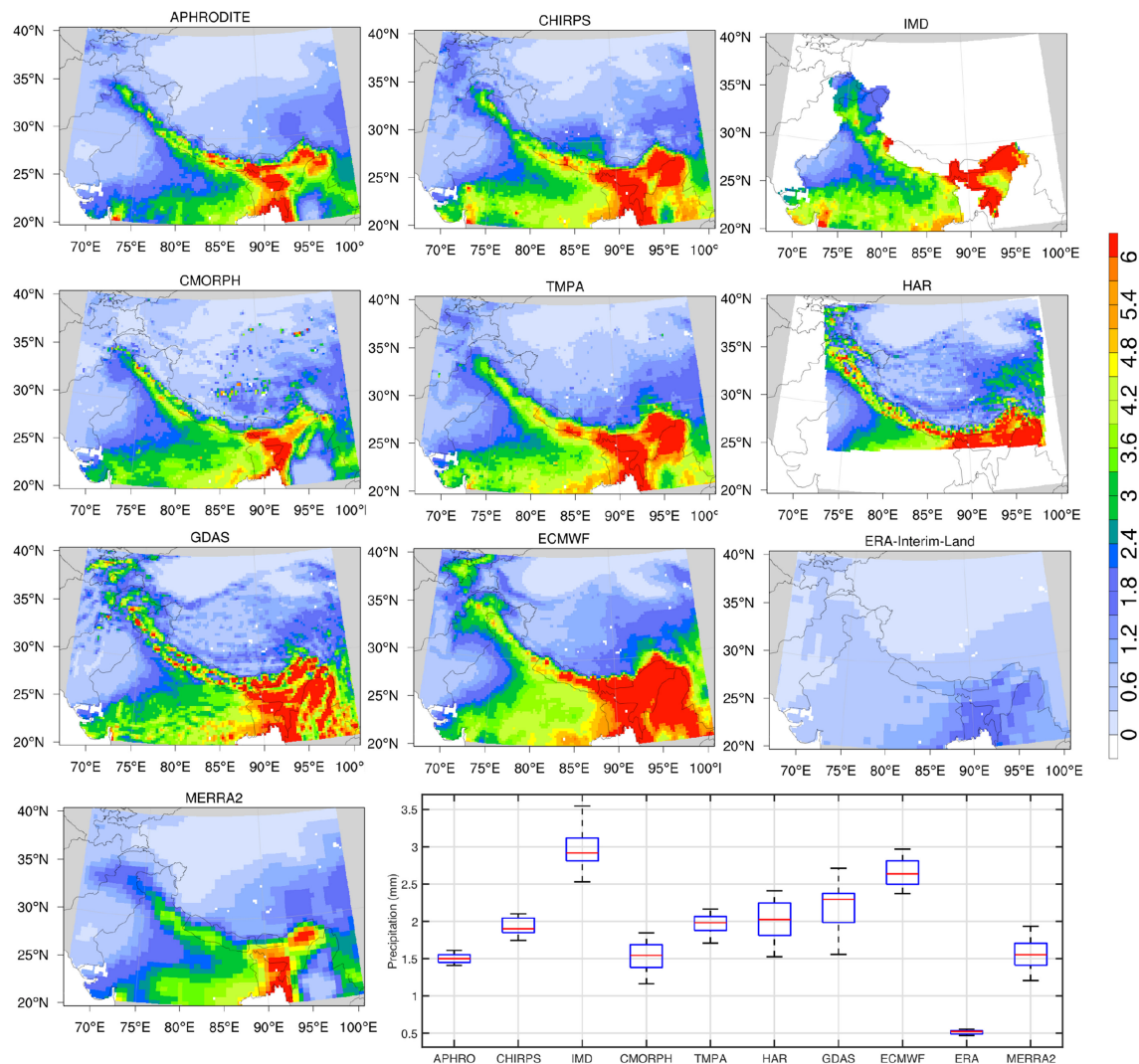
FIGURE 2 | Spatial maps of multi-annual mean precipitation (mm) and their distribution from 10 precipitation datasets ( Table 1 ). The box plot in the lower-right illustrates the median (red line), upper- and lower-quantiles (blue box) and the 25- and 75-th percentiles (black whiskers) of the multi-annual mean precipitation. Note that the IMD and HAR datasets are only available over part of the entire domain of interest.
