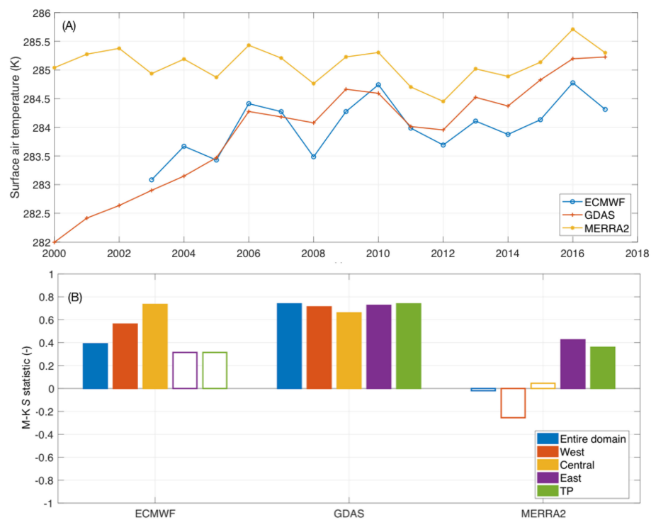
FIGURE 9 | Time series of domain-averaged mean annual near surface air temperature (A), and estimates of the Mann Kendall S-statistic (B) for the entire HMA and four sub-regions (Figure 1). The statistically significant trends are shown with filled boxes.
