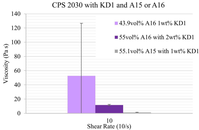
Figure 3. CPS 2030 with KD1 and A15 or A16.
