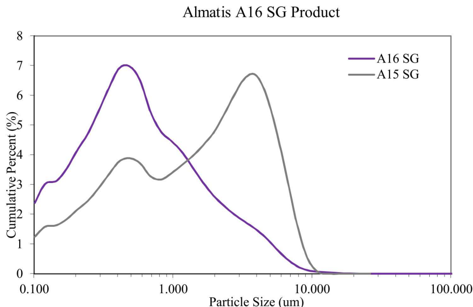
Figure 1. Typical particle size distribution curve for A15 SG and A16 SG (C. Compson, personal communication, May 9, 2018).
