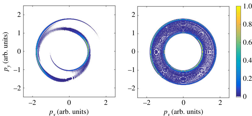
Figure 12. Simulated Auger electron momentum distribution resulting from core-level ionization with a 300 as X-ray pulse in the presence of a 2.4\ \mu\text{m} ( T_L = 8\ \text{fs} ), circularly polarized streaking field. The simulation is done in the strong-field approximation with a streaking field with U_p = 2.5\ \text{eV} , and assumes an isotropic distribution of Auger electron emission. (a) An Auger lifetime of 1 fs, so that, \tau_X < \tau_A < T_L . In (b), the Auger lifetime is 4 fs and comparable to the streaking laser period, i.e. \tau_X < \tau_A \sim T_L . As in figure 9, the Auger electron momentum distribution intensity is normalized to 1. (Online version in colour.)
