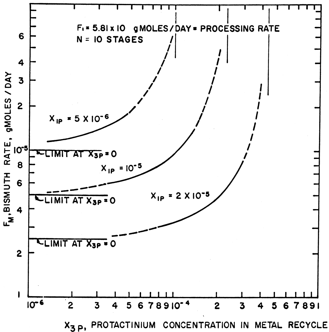
Fig. 7 Metal Rate for a Large Number of Stages.
