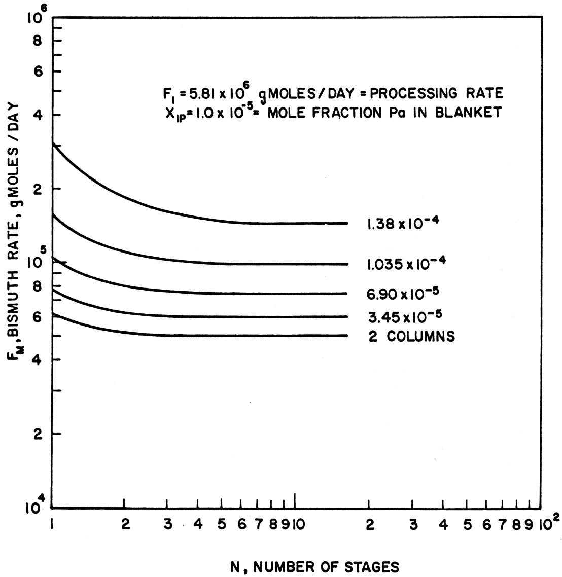
Fig. 5 Metal Rate for Processing a Blanket with 1 \times 10^{-5} Mole Fraction Protactinium.
