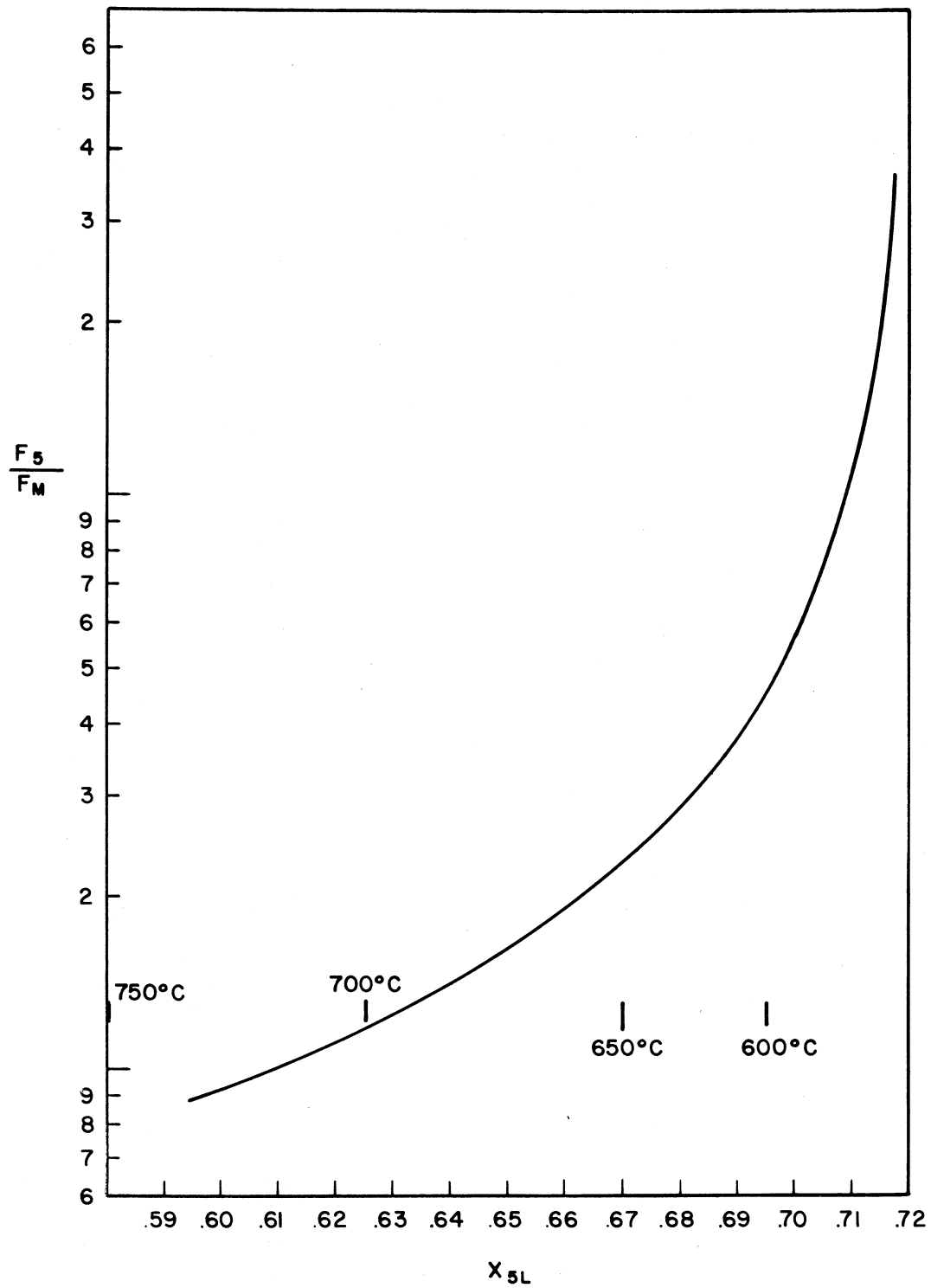
Fig. 8 Composition of Recycle Salt.
