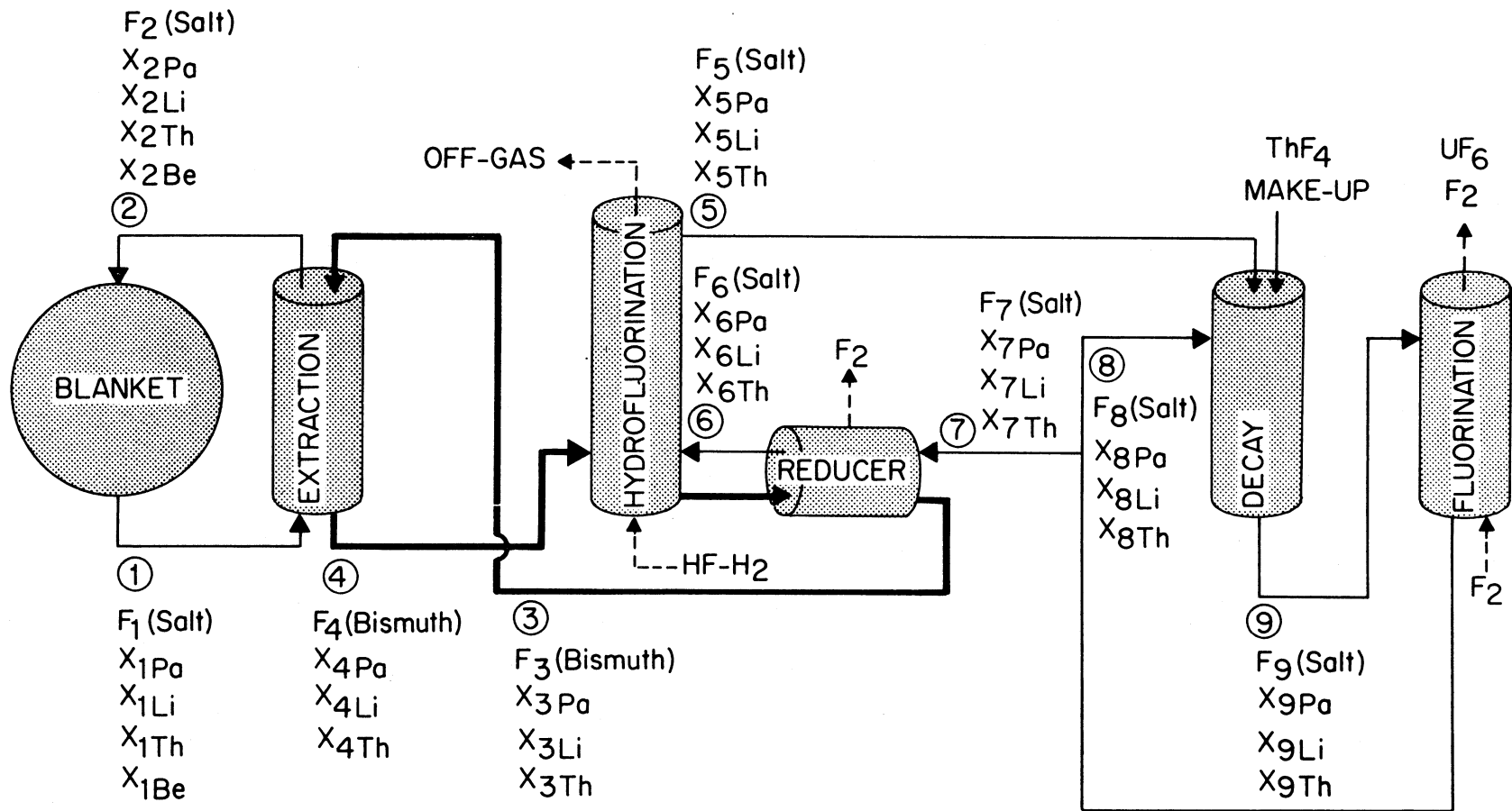
Fig. 1 Basic Flowsheet.
