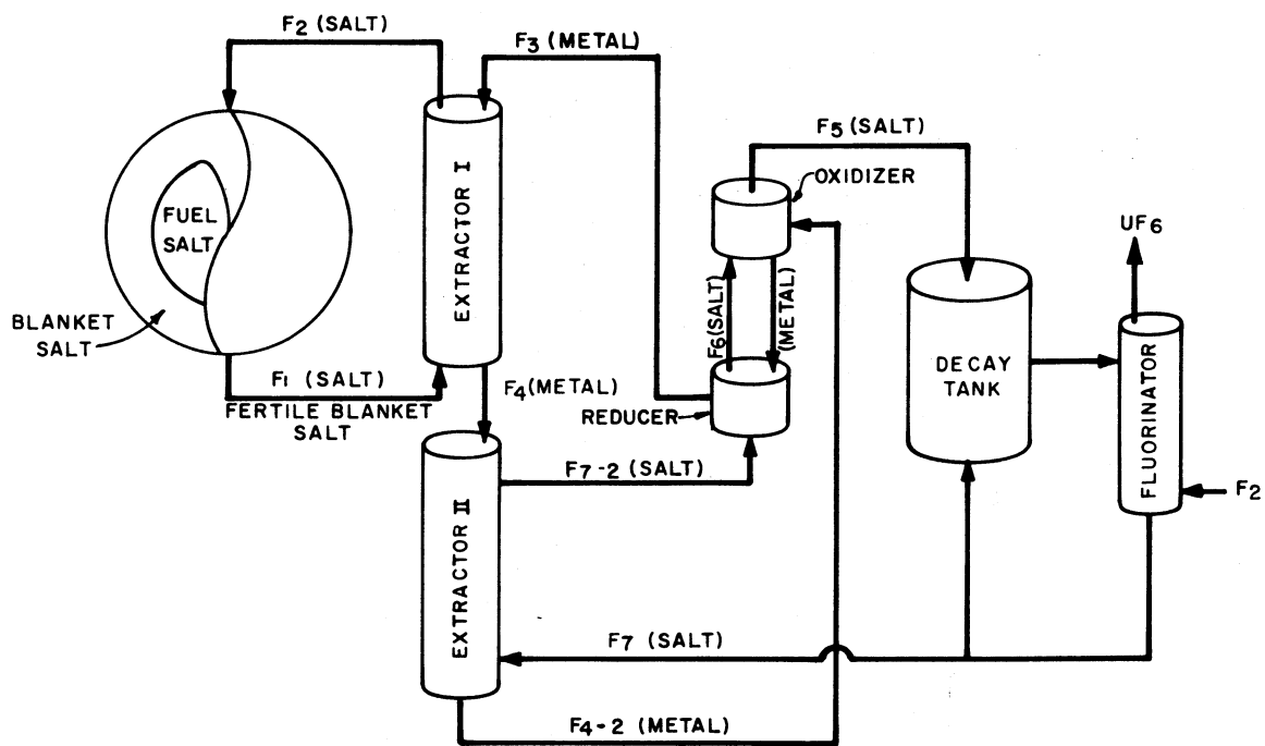
Fig. 2 Modified Flowsheet.
