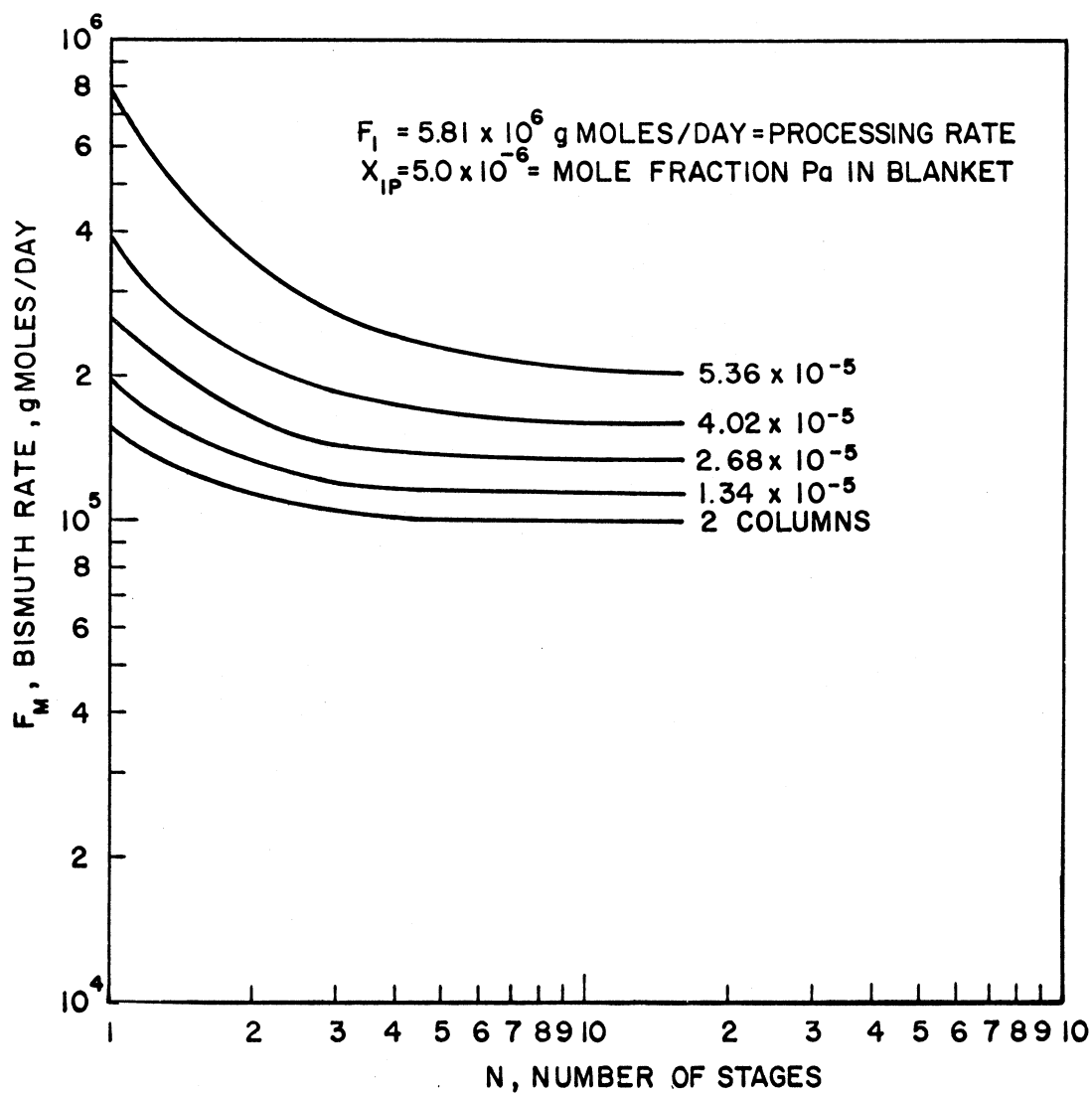
Fig. 4 Metal Rate for Processing a Blanket with 5 \times 10^{-6} Mole Fraction Protactinium.
