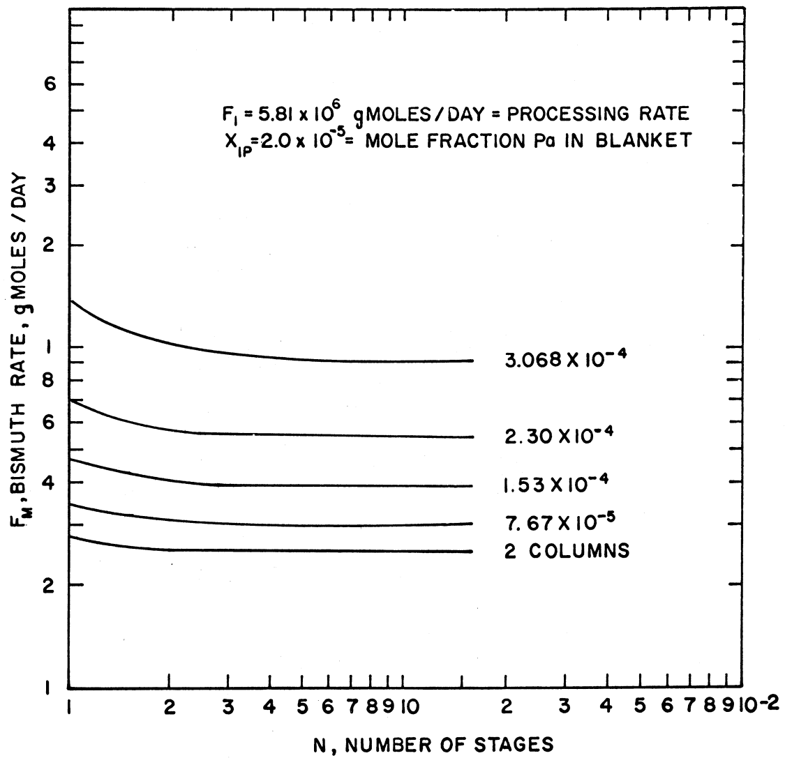
Fig. 6 Metal Rate for Processing a Blanket with 2 \times 10^{-5} Mole Fraction Protactinium.
