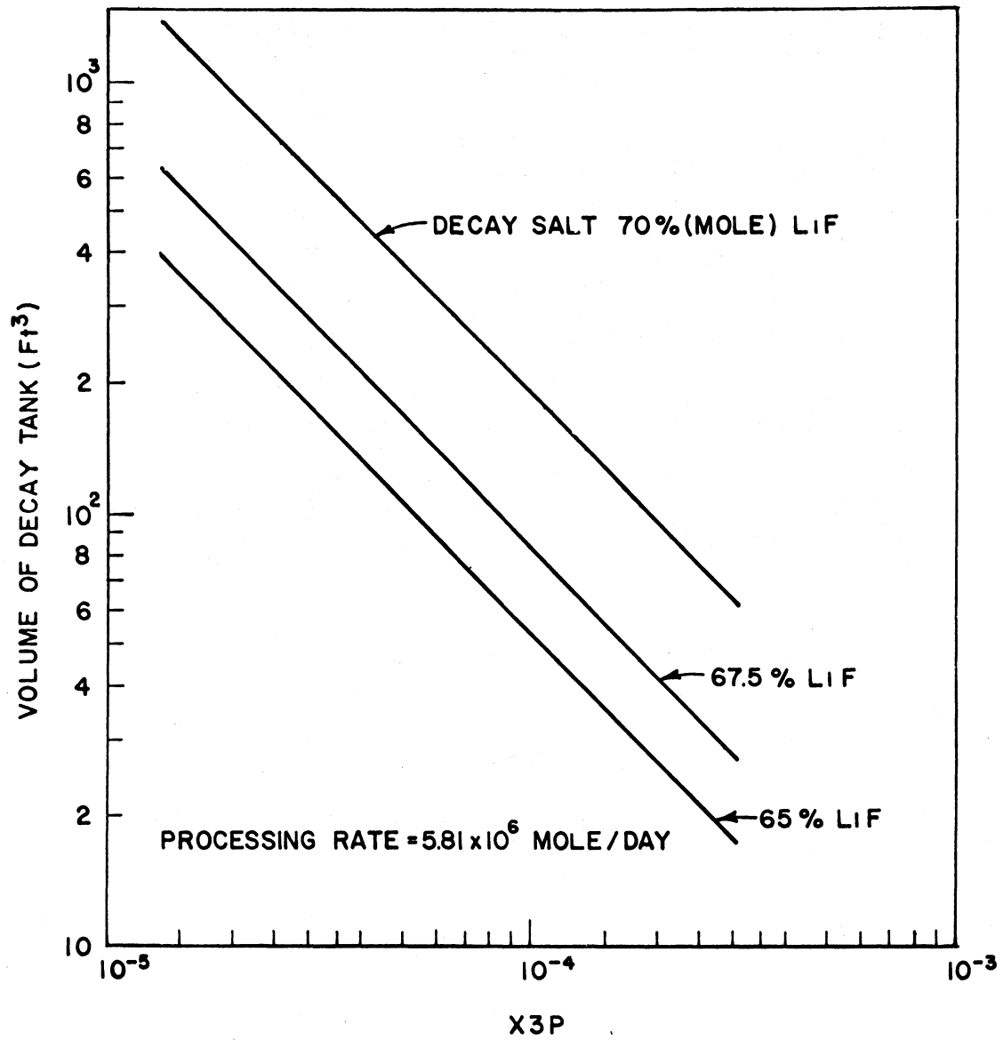
Fig. 9 Volume of the Decay Tank.
