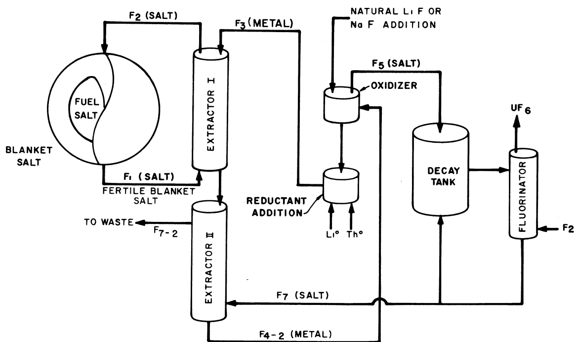
Fig. 3 "Throw-away" (or no reducer) Flowsheet.
