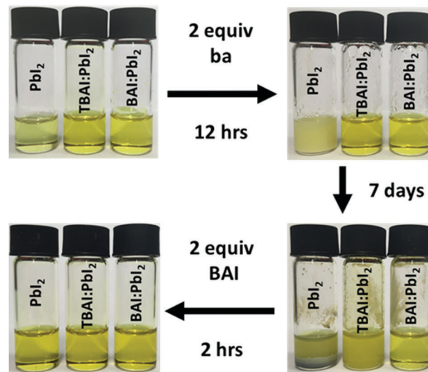
Fig. 1 Photographs of PbI_2 , TBAI: PbI_2 (molar ratio 1:1), and BAI: PbI_2 (molar ratio 1:1) dissolved in DMF reacting with 2 equivalents of butylamine (ba) additive at 55^\circ\text{C} . After one week, the resulting precipitates were fully reversible by the addition of excess BAI.
