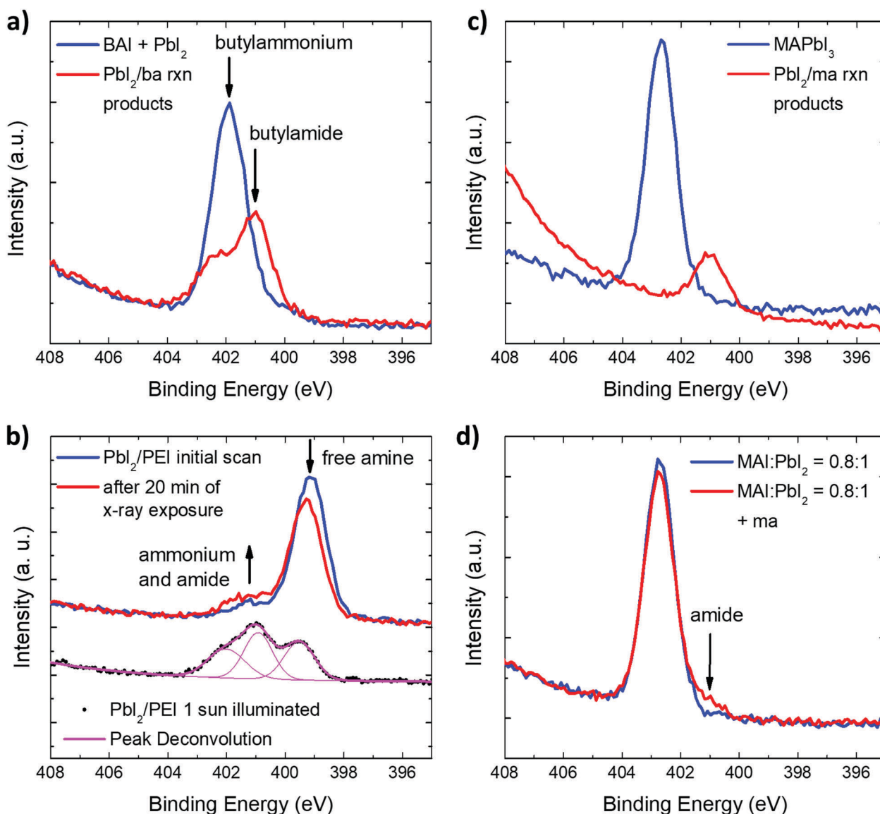
Fig. 4 N 1s XPS of (a) drop cast samples of \text{BAI}:\text{PbI}_2 (1 : 1 ratio in DMF) and the supernatant of the \text{PbI}_2 /butylamine reaction in DMF, (b) a thin film bilayer of \text{PbI}_2 /linear-PEI showing in situ changes in relative intensity of the free amine peak (BE \approx 399.5 eV) and amide/ammonium peaks (BE > 400 eV), (c) thin films of an \text{MAPbI}_3 control (1 : 1 MAI : \text{PbI}_2 ratio) and \text{PbI}_2 /methylamine reaction in DMF showing amide formation with methylamine, and (d) amide formation in a non-stoichiometric MAI : \text{PbI}_2 solution in DMF after the addition of methylamine.
