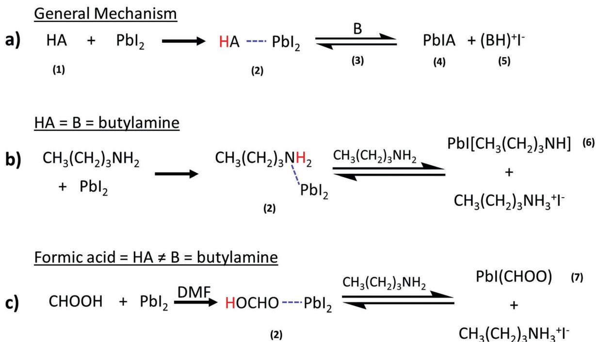
Scheme 1 (a) General mechanism in anhydrous conditions by which a protic molecule (HA) is acidified upon coordination to \text{PbI}_2 (denoted by H and dashed line) which can induce deprotonation by a suitable base (B). (b) Example of reaction when the same molecule, butylamine, acts as both the acid and the base. (c) Example for a reaction between HA and B (formic acid and butylamine in DMF) which would be unfavorable in the absence of \text{PbI}_2 but is promoted by the Lewis acidity of \text{PbI}_2 .
