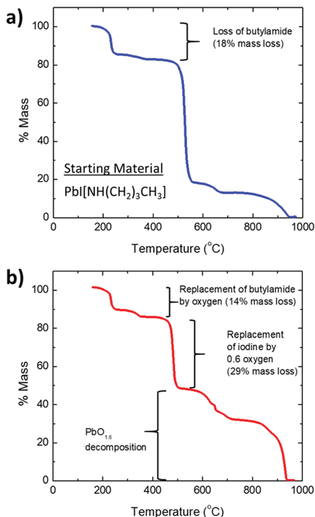
Fig. 5 TGA of the isolated precipitate from the reaction of \text{PbI}_2 and butylamine in DMF under (a) \text{N}_2 and (b) ambient air. The mass losses indicated for (a) butylamide removal and (b) replacement of butylamide by oxygen confirm the hypothesized starting composition of \text{PbI}[\text{CH}_3(\text{CH}_2)_3\text{NH}] .
