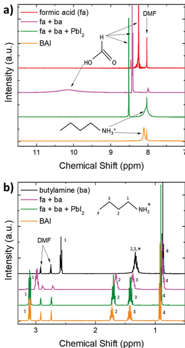
Fig. 6 1 H-NMR at (a) high and (b) low chemical shifts of combinations of formic acid (fa), butylamine (ba), and PbI 2 in deuterated DMF (d 7 -DMF). The spectra indicate that the presence of PbI 2 induces proton transfer from formic acid to butylamine in d 7 -DMF whereas no reaction is observed for the formic acid + butylamine control.
