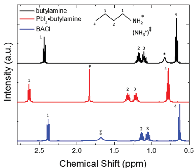
Fig. 2 Chemical shifts of the N-H protons measured by 1 H-NMR of butylamine, butylammonium, and PbI 2 -butylamine coordination complex in deuterated chloroform. The magnitude of the downfield shifts corroborates the acidification of butylamine complexed to Pb 2+ .
