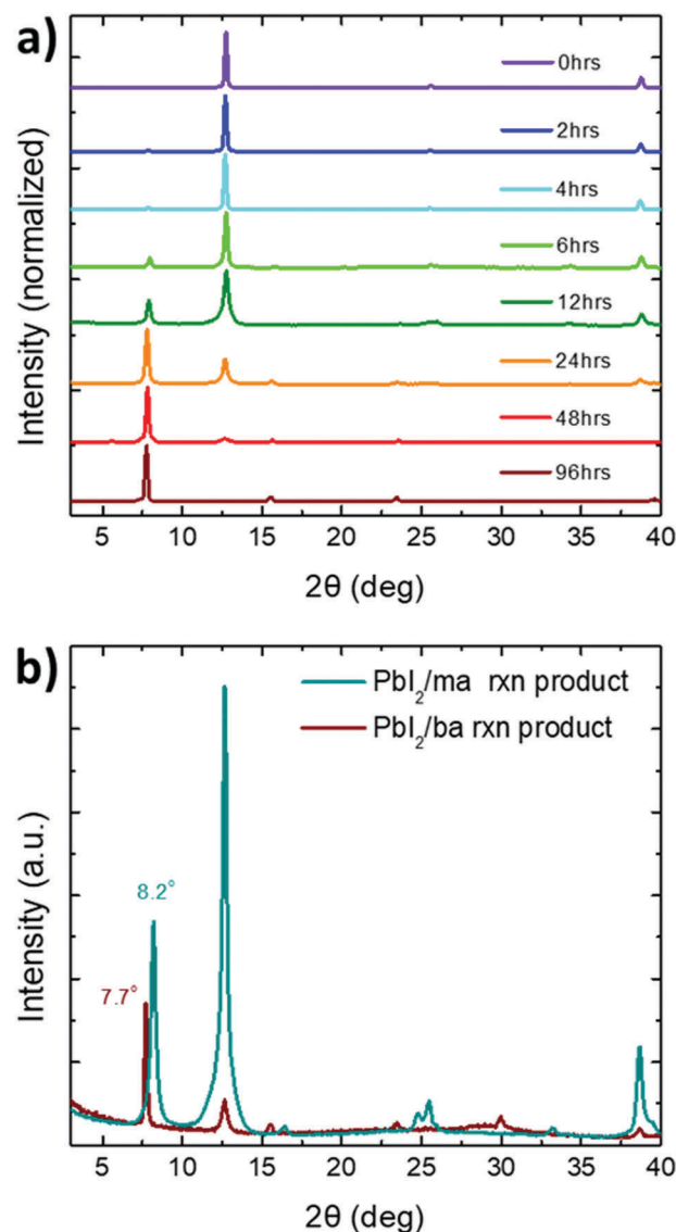
Fig. 3 (a) Normalized XRD patterns of drop cast samples of a PbI 2 /butylamine (1:2) solution in DMF as a function of reaction time showing a gradual shift from PbI 2 to a new phase potentially containing Pb-butylamide moieties. (b) Comparison of XRD of the PbI 2 /methylamine (ma) reaction product to PbI 2 /butylamine (ba) reaction product.
