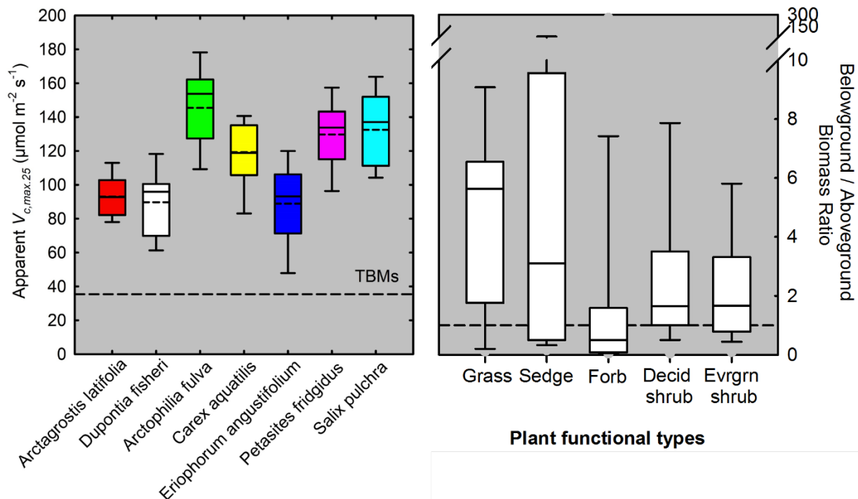
Figure 1. Observations and synthesis activities inform the improved representation of above- and below-ground plant traits in terrestrial biosphere models. (a) Apparent maximum carboxylation rate normalized to 25°C (apparent V_{c,max,25} ) measured in seven species located on the Barrow Environmental Observatory, Utqiagvik, Alaska. (b) Below- to above-ground biomass ratio of plant functional types across tundra ecosystems. Dashed lines in a, b represent current terrestrial biosphere model representation of these plant traits.
