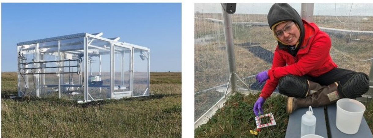
Figure 2. A Zero-Power Warming (ZPW) chamber. The chamber is warmed passively by solar radiation. The combination of an internal and an external heat exchanger modulates venting of the chamber, which enables the air temperature to be elevated by about 4^\circ\text{C} .
