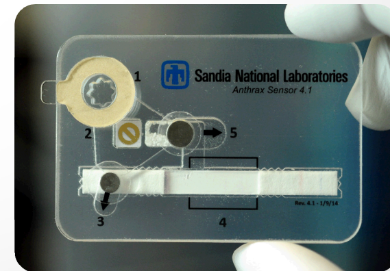
Portable anthrax detector (BaDx)
