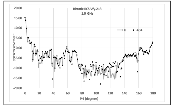
Figure 2. Comparison of bistatic RCS for the VFY-218 at 1GHz for the LU and ACA solution.
