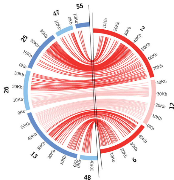
Figure 3. Alignment of three Deltaproteobacteria reconstructed synetic regions from the 5-m sample to a closely related genome reconstructed from the planktonic filtrate sample GWC2. Lines connect homologous genes.
