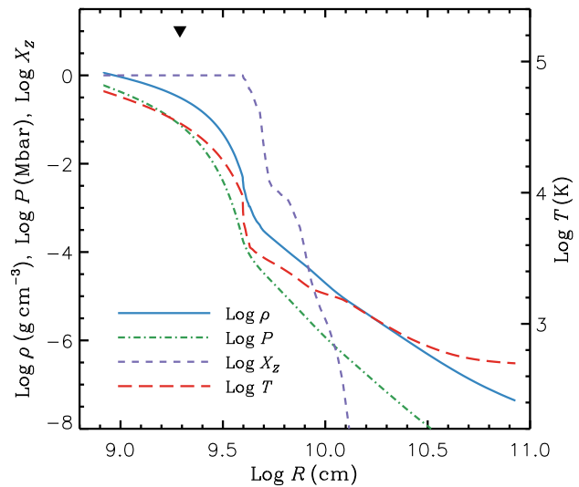
Figure 11. Structure of the model in Run 1.00(Rev) at time 1 \times 10^4 yr, at 1 AU just before the onset of migration. Solid curve (left scale): log density in \text{g cm}^{-3} ; dash-dot curve (left scale): log pressure in Mbar. The surface value (not plotted) is 7.56 \times 10^{-4} bar. Long-dashed curve (right scale): log temperature in K; short-dashed curve (left scale): log X_z , the log of the mass fraction of heavy elements. Filled triangle: the half-mass point in the envelope. The mean density of the inner core is 4.63 \text{ g cm}^{-3} . Note that the composition curve at \log r = 9.7 is practically discontinuous; it is resolved by a few grid points. Interior to that point, the model is convective; outside \log r = 9.91 it is radiative.
