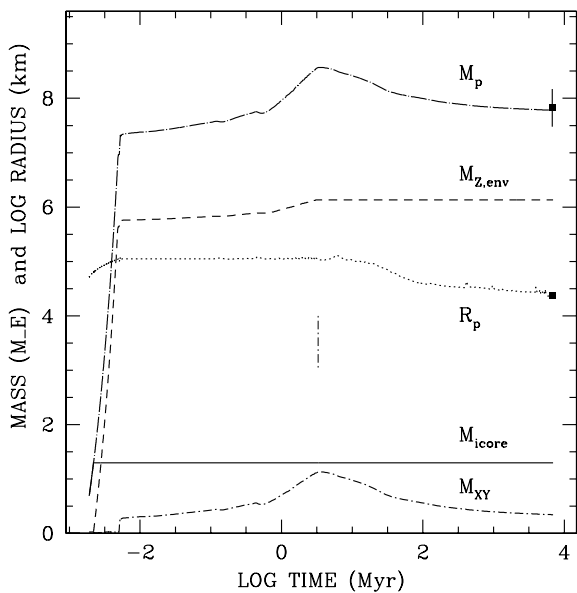
Figure 2. Evolution of Run 0.128(Rev). Upper (long dash-dot) curve: total mass M_p (in M_{\oplus} ); dashed curve: total heavy-element mass in the envelope M_{Z,\text{env}} ; dotted curve: outer log radius R_p (in km); solid curve: heavy-element inner core mass M_{\text{icore}} ; short dash-dot curve: hydrogen/helium mass in the envelope M_{\text{XY}} ; vertical dash-dot line: time of disk accretion cutoff. The observed mass of Kepler-36 c, with error bars at 84% confidence level, and the observed radius, are given as filled squares.
