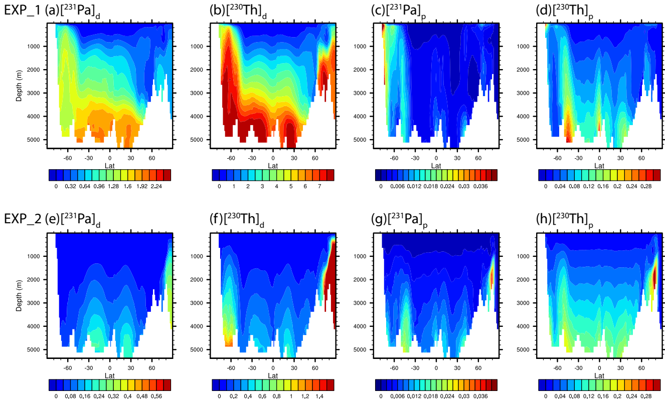
Figure 6. Atlantic zonal mean dissolved and particulate ^{231}\text{Pa} and ^{230}\text{Th} in Exp_1 and Exp_2 (unit: \text{dpm m}^{-3} ). Exp_1: (a) dissolved ^{231}\text{Pa} , (b) dissolved ^{230}\text{Th} , (c) particulate ^{231}\text{Pa} , (d) particulate ^{230}\text{Th} . Exp_2: (e) dissolved ^{231}\text{Pa} , (f) dissolved ^{230}\text{Th} , (g) particulate ^{231}\text{Pa} , (h) particulate ^{230}\text{Th} .
