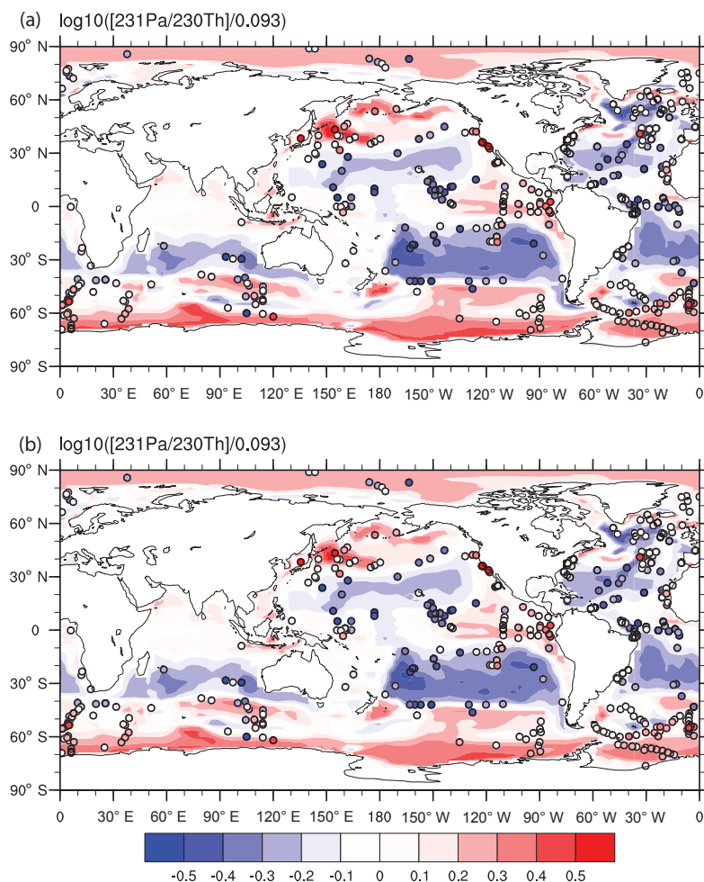
Figure 4. The sediment ^{231}\text{Pa}/^{230}\text{Th} activity ratio in CTRL for both p-fixed (a) and p-coupled version (b). Observations are attached as filled circles using the same color map. The ^{231}\text{Pa}/^{230}\text{Th} activity ratio is plotted relative to the production ratio of 0.093 on a \log_{10} scale.
