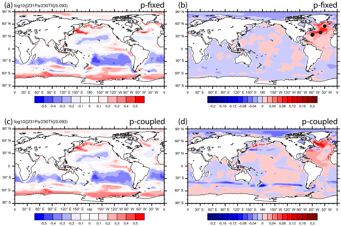
Figure 10. The sediment ^{231}\text{Pa} / ^{230}\text{Th} activity ratio during AMOC off state and the difference between AMOC off and CTRL. (a) P-fixed \log_{10}([^{231}\text{Pa} / ^{230}\text{Th}] / 0.093) in AMOC_off. (b) Difference in the p-fixed sediment ^{231}\text{Pa} / ^{230}\text{Th} activity ratio between AMOC_off and AMOC_on. Panels (c) and (d) are similar to (a) and (b) for the p-coupled sediment ^{231}\text{Pa} / ^{230}\text{Th} activity ratio. Black dots in (b) shows the locations of sites in Fig. 9 from north to south.
