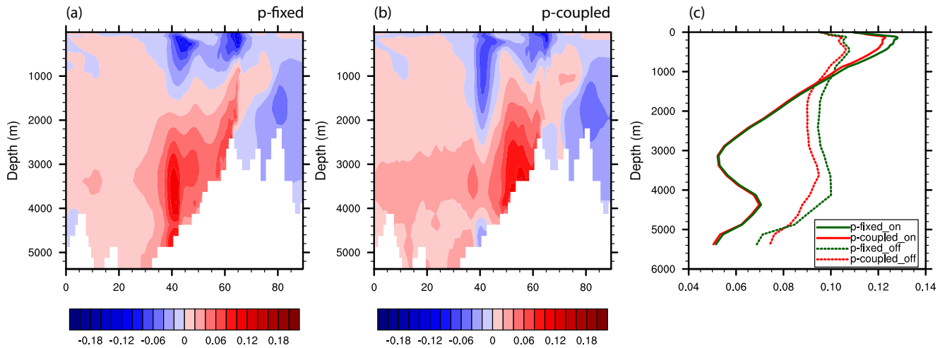
Figure 12. Difference of Atlantic zonal mean (a) p-fixed and (b) p-coupled particulate ^{231}\text{Pa} / ^{230}\text{Th} between AMOC_off and AMOC_on. (c) North Atlantic (20–60° N) average profile during AMOC_on (solid) and AMOC_off (dash) for p-fixed (green) and p-coupled (red) particulate ^{231}\text{Pa} / ^{230}\text{Th} .
