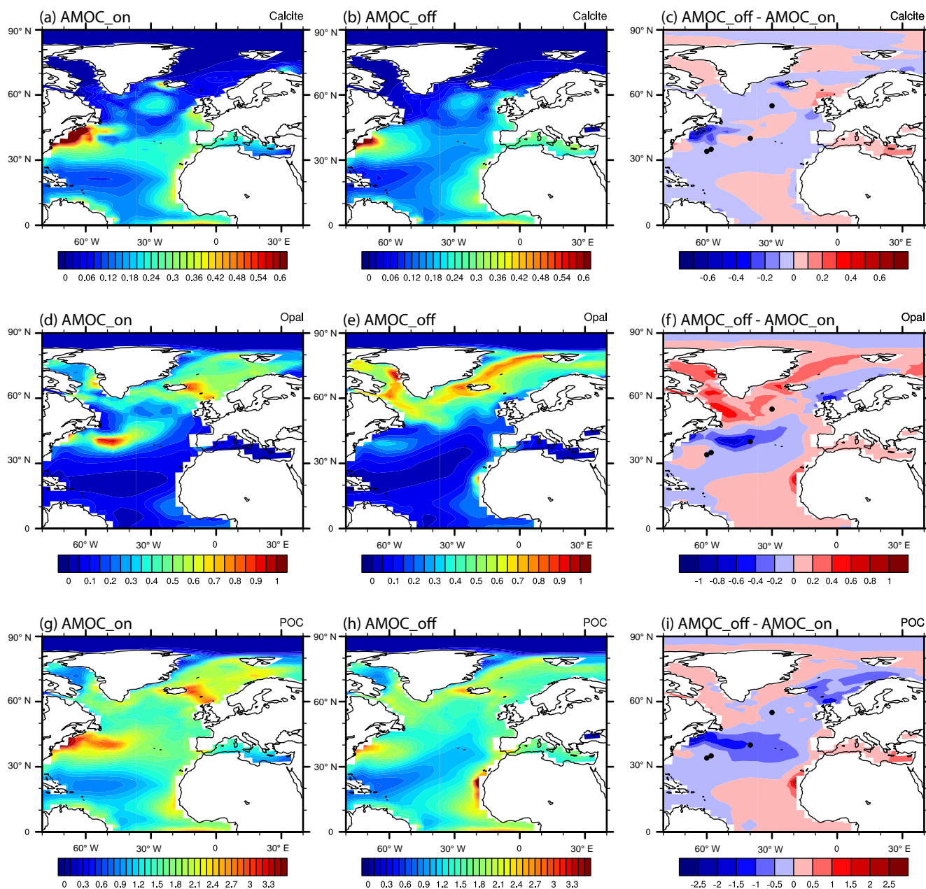
Figure 8. Comparison of particle fluxes between AMOC_on and AMOC_off. \text{CaCO}_3 flux at 105 m ( \text{mol m}^{-2} \text{yr}^{-1} ) during AMOC_on (a), AMOC_off (b) and the difference between AMOC_off and AMOC_on (c). Opal flux at 105 m ( \text{mol m}^{-2} \text{yr}^{-1} ) during AMOC_on (d), AMOC_off (e) and the difference between AMOC_off and AMOC_on (f). POC flux at 105 m ( \text{mol m}^{-2} \text{yr}^{-1} ) during AMOC_on (g), AMOC_off (h) and the difference between AMOC_off and AMOC_on (i).
