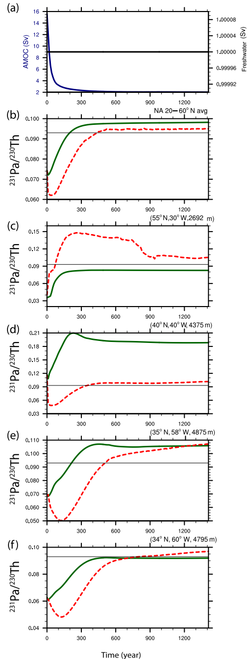
Figure 9. Time evolutions in HOSING. (a) Freshwater forcing (black) and AMOC strength (navy), which is defined as the maximum of the overturning stream function below 500m in the North Atlantic. (b) The North Atlantic average sediment ^{231}\text{Pa}/^{230}\text{Th} activity ratio from 20° N to 60° N: p-fixed (green) and p-coupled (red). The production ratio of 0.093 is indicated by a solid black line (similar to in c, d, e and f). (c) The sediment ^{231}\text{Pa}/^{230}\text{Th} activity ratio at (55° N, 30° W). (d) The sediment ^{231}\text{Pa}/^{230}\text{Th} activity ratio at (40° N, 40° W). (e) The sediment ^{231}\text{Pa}/^{230}\text{Th} activity ratio at (35° N, 58° W). (f) The sediment ^{231}\text{Pa}/^{230}\text{Th} activity ratio at (34° N, 60° W). Panels (e) and (f) show locations near the Bermuda Rise. Locations of each site are shown as dots in Fig. 8b.
