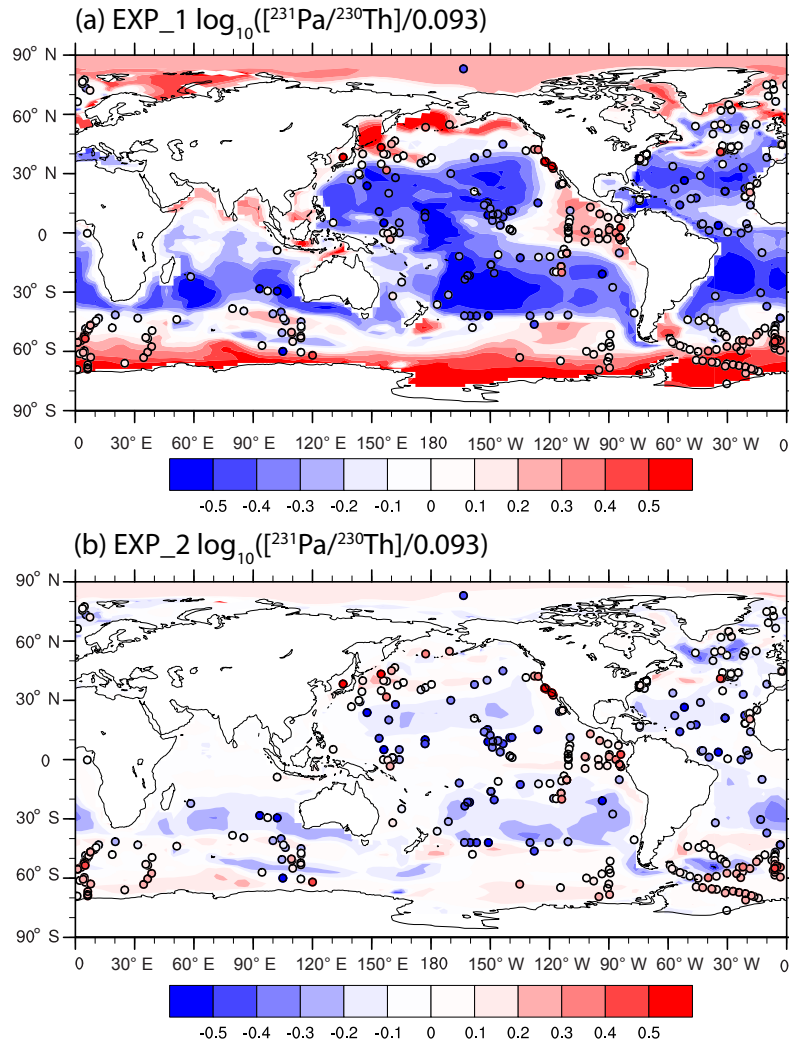
Figure 7. The sediment ^{231}\text{Pa}/^{230}\text{Th} activity ratio in Exp_1 (a) and Exp_2 (b). Observations are attached as filled circles using the same color map. The ^{231}\text{Pa}/^{230}\text{Th} activity ratio is plotted relative to the production ratio of 0.093 on a \log_{10} scale.
