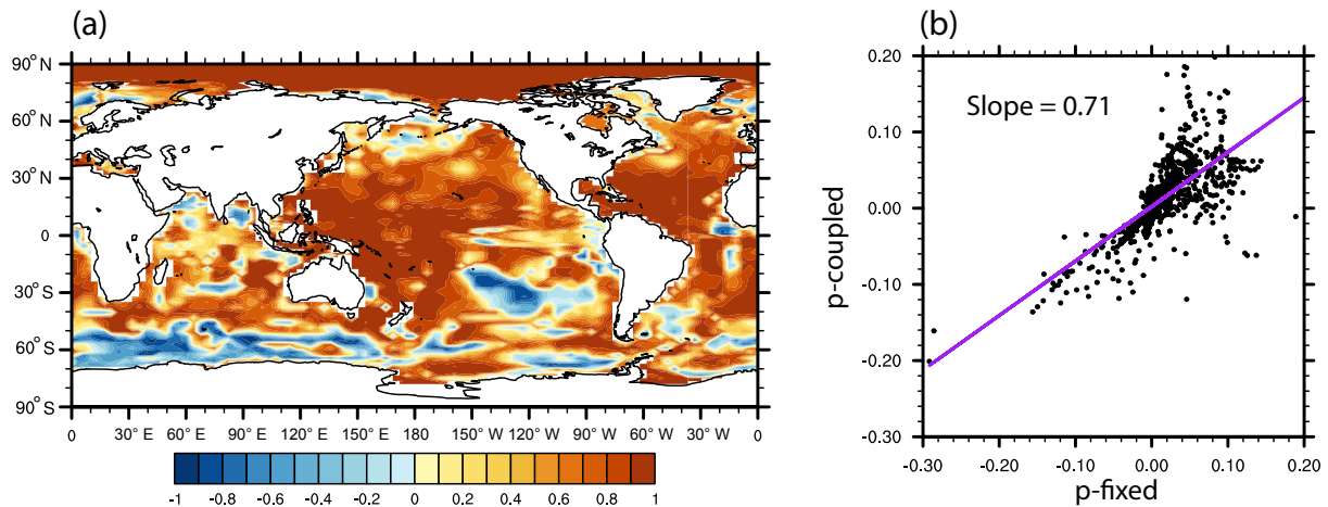
Figure 11. (a) Correlation of p-fixed and p-coupled evolution of the sediment ^{231}\text{Pa} / ^{230}\text{Th} activity ratio in HOSING. (b) Scatter plot of the p-fixed and p-coupled sediment ^{231}\text{Pa} / ^{230}\text{Th} activity ratio change from AMOC_on to AMOC_off in the Atlantic and the Southern Ocean ( 70^\circ\text{W} - 20^\circ\text{E} ). Purple line is the least-squares linear regression line and slope is the linear regression coefficient.
