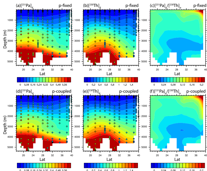
Figure 3. Dissolved ^{231}\text{Pa} , dissolved ^{230}\text{Th} and particulate ^{231}\text{Pa} / ^{230}\text{Th} in CTRL along GEOTRACES transect GA03 (Hayes et al., 2015) (the track is indicated in Fig. S4) for both p-fixed (top row) and p-coupled (bottom row) ^{231}\text{Pa} and ^{230}\text{Th} (colored contour). Observations of dissolved ^{231}\text{Pa} and ^{230}\text{Th} activity are superimposed as colored circles using the same color scale.
