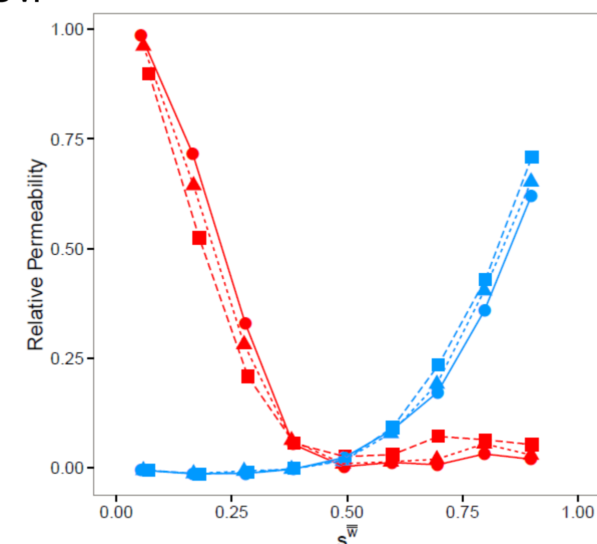
Figure 6. Relative permeability curves determined from pore-scale multiphase LB simulations within a sandstone reservoir for three contact angles 20°, 45°, and 70°.
