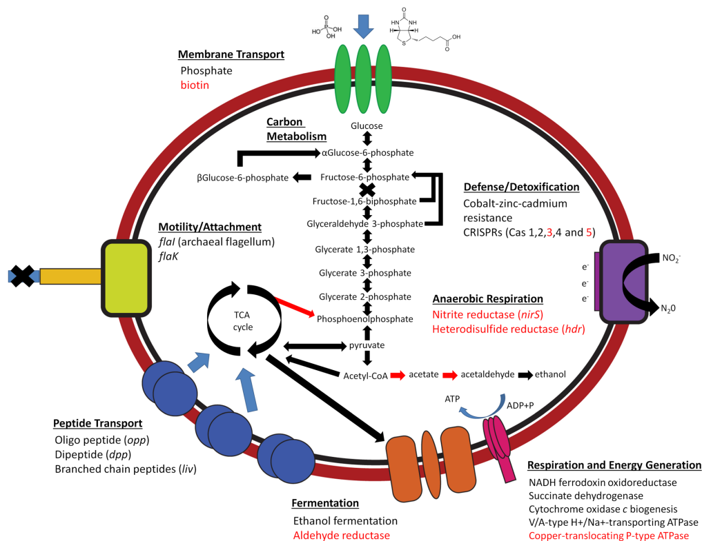
FIGURE 2 | Predicted metabolisms of combined NAG1 single-amplified genome (SAG) assembly and MLP metagenomic assembly at Great Boiling Spring (GBS), Nevada. Red text and arrows indicate genes and proteins that are unique to GBS NAG1 genomes.
