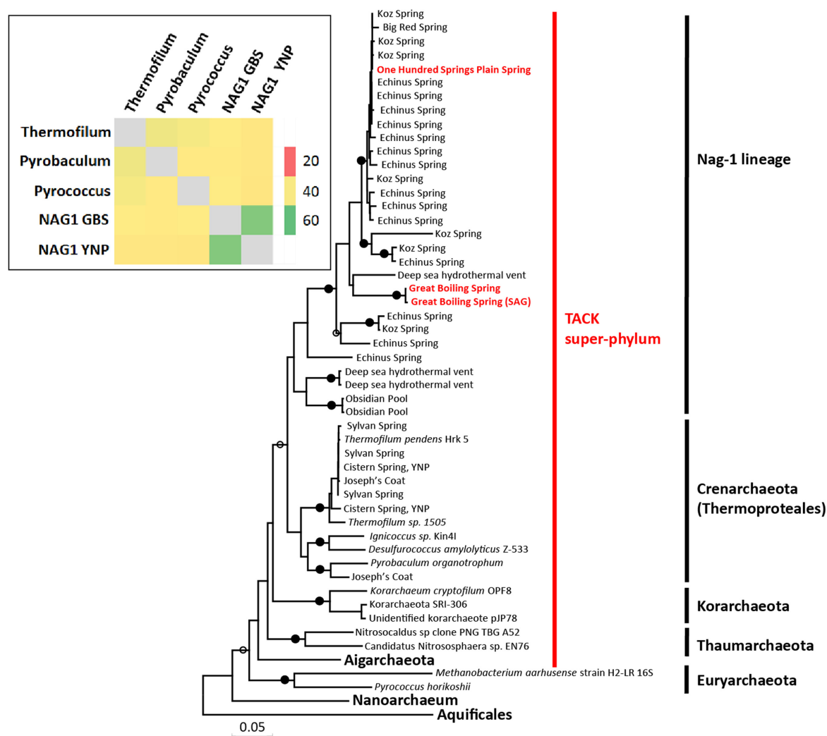
FIGURE 1 | Maximum-likelihood phylogeny of partial 16S rRNA genes (1020 bp) containing sequenced members of the NAG1 phylum (>85% nucleotide identity), as well as members of the Crenarchaeota sequenced from hot springs and other well-known archaeal phyla. Hot springs locations where NAG1 sequences were isolated and sequenced are indicated next to the terminal branch in that clade. Black circles indicate bootstrap values >95%; open circles >70%. Scale bar indicates 0.05 substitutions per site. Insert (upper left); heat map of average amino acid (AAI) values among the NAG1 genomes and select genomes in the Crenarchaeota and Euryarchaeota. See Supplementary Figure S1 for GenBank IDs.
