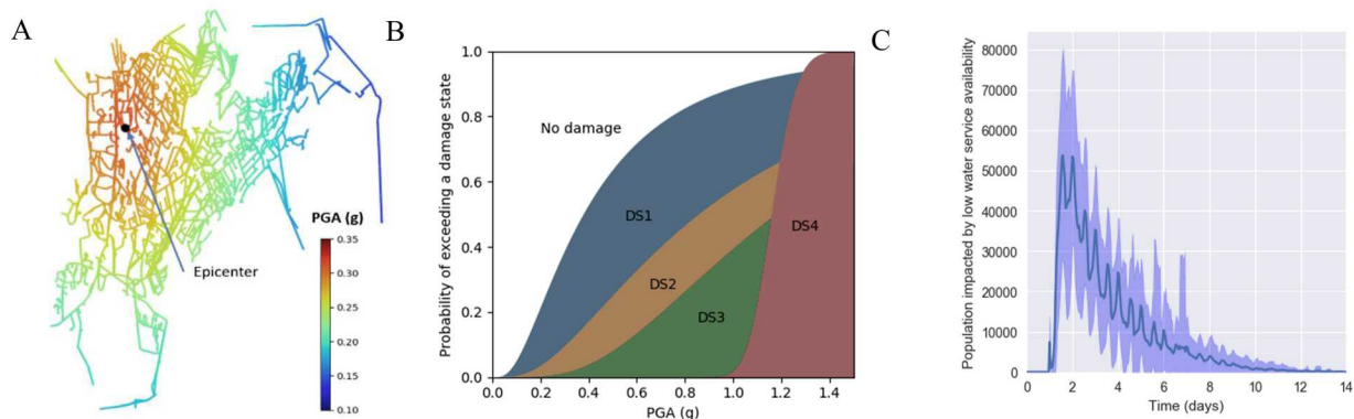
Figure 3. (A) Simulated peak ground acceleration (PGA) from a magnitude 6.5 earthquake, (B) fragility curves defining tank damage states, and (C) stochastic analysis results for the population impacted by low water service availability following an earthquake (mean value and shaded region covering 2 standard deviations).
