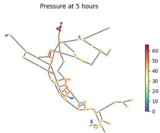
Figure 6. Network graphic created from the simple example.
