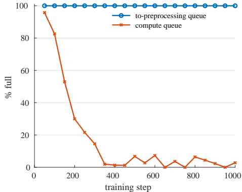
Fig. 2: For the default single pipeline, the preprocessing queue is always full, while the compute queue empties quickly. Thus the preprocessing task is the bottleneck.
