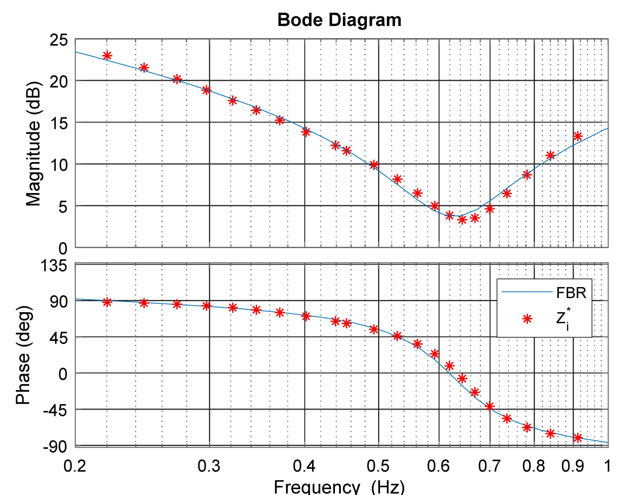
Figure 3: Bode plot comparing SID matching with Impedance complex conjugate.
