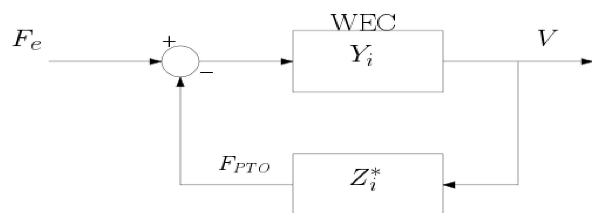
Figure 1: Complex Conjugate Controller
