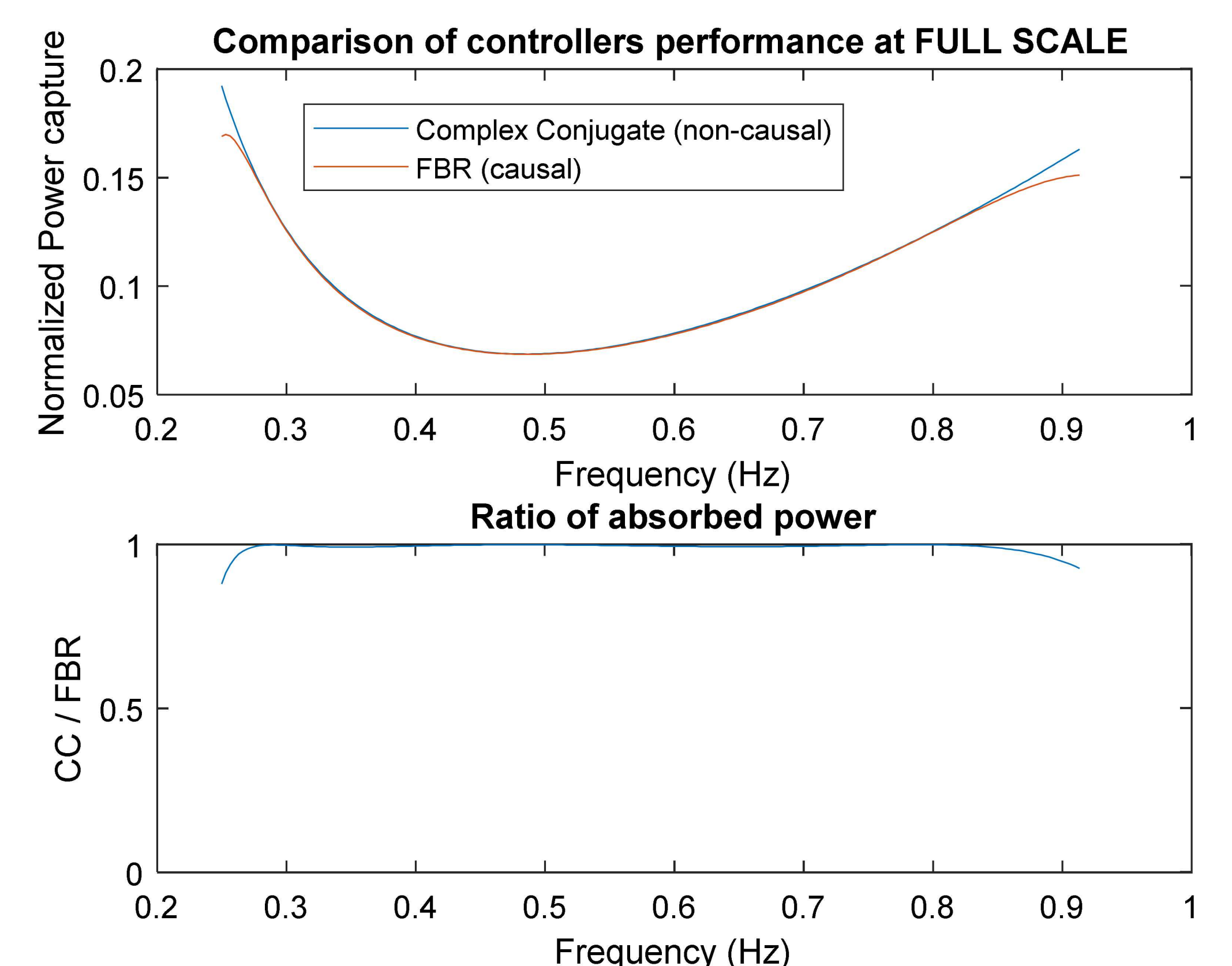
Figure 4: Comparison of the Power Absorbed by the CC control and the FBR Control
