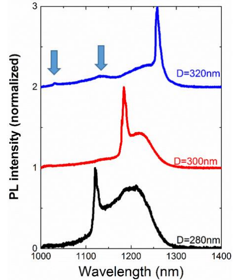
Figure 4. PL spectra measured from three different nano-cylinder array samples where the resonators diameter has been varied.
