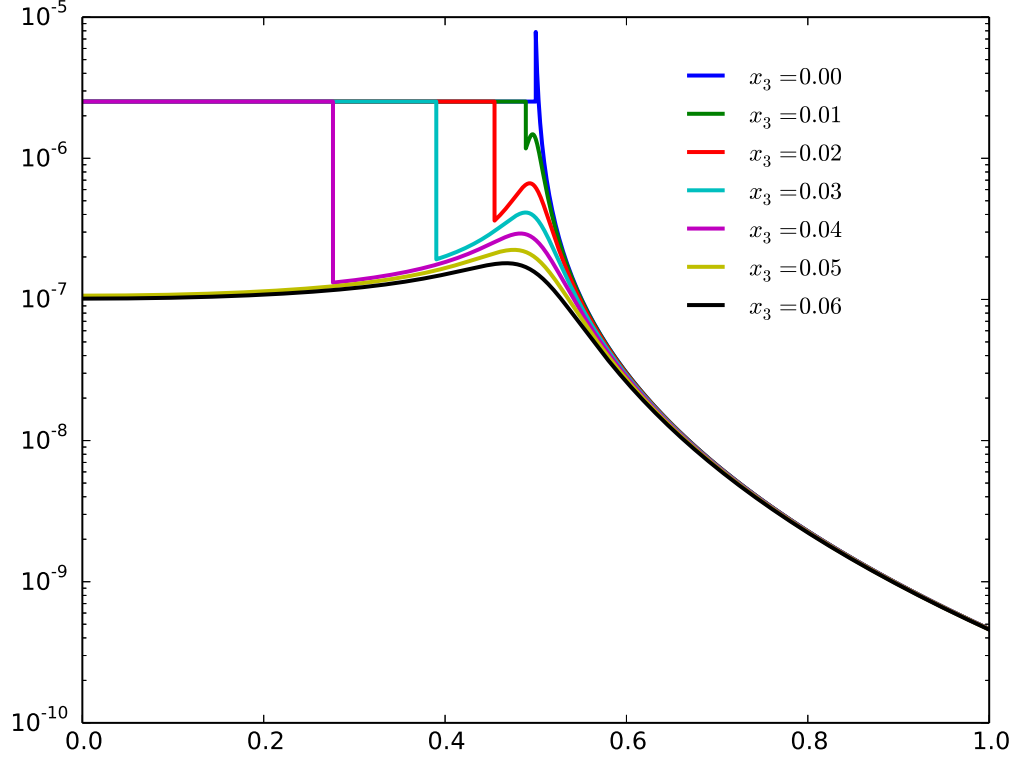
Figure 3: Oblate ellipsoid; energy density versus x_1, x_2 = 0
