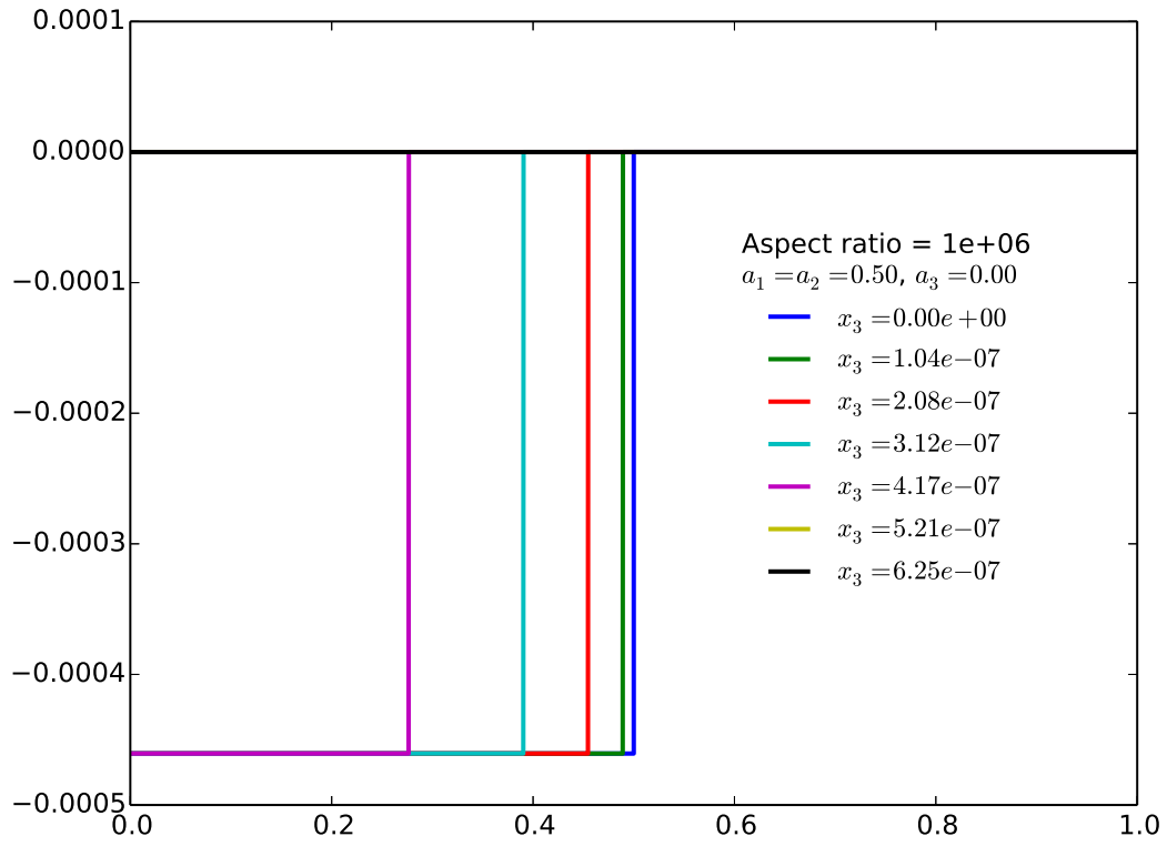
Figure 15: Oblate ellipsoid ( a_1 = a_2 = 0.5, a_3 = a_1/h, h = 1 \times 10^6 ); pressure p versus x_1 .
