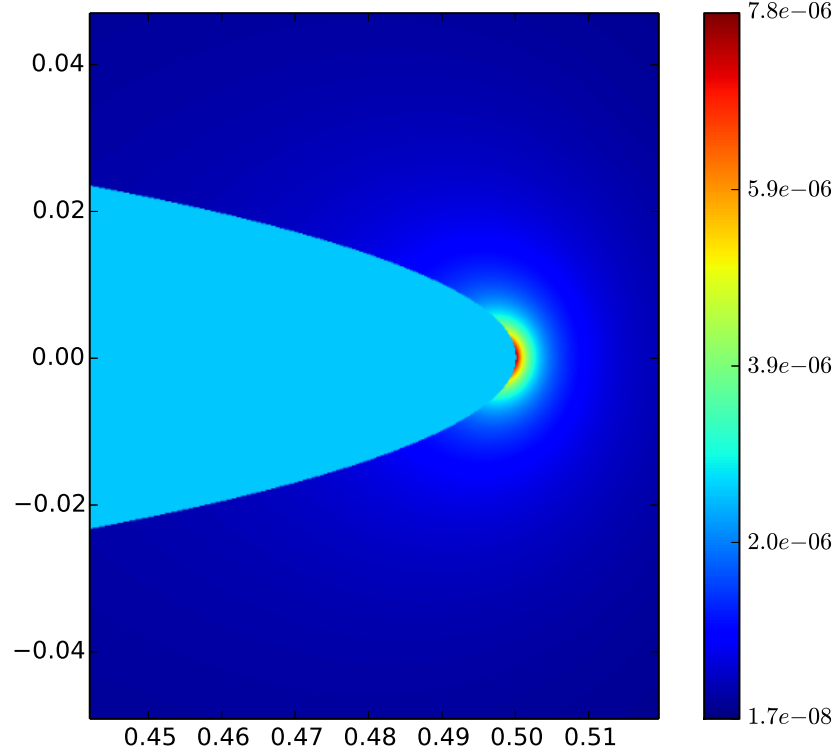
Figure 5: Oblate ellipsoid; energy density; zoom window shown in Figure 4.
