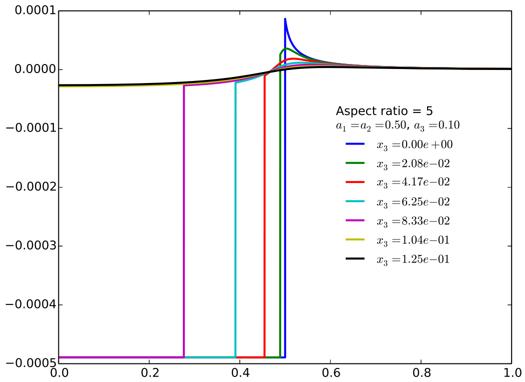
Figure 12: Oblate ellipsoid ( a_1 = a_2 = 0.5, a_3 = a_1/h, h = 5 ); pressure p versus x_1 .
