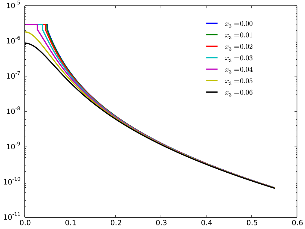
Figure 7: Prolate ellipsoid; energy density versus x_2 , x_1 = 0
