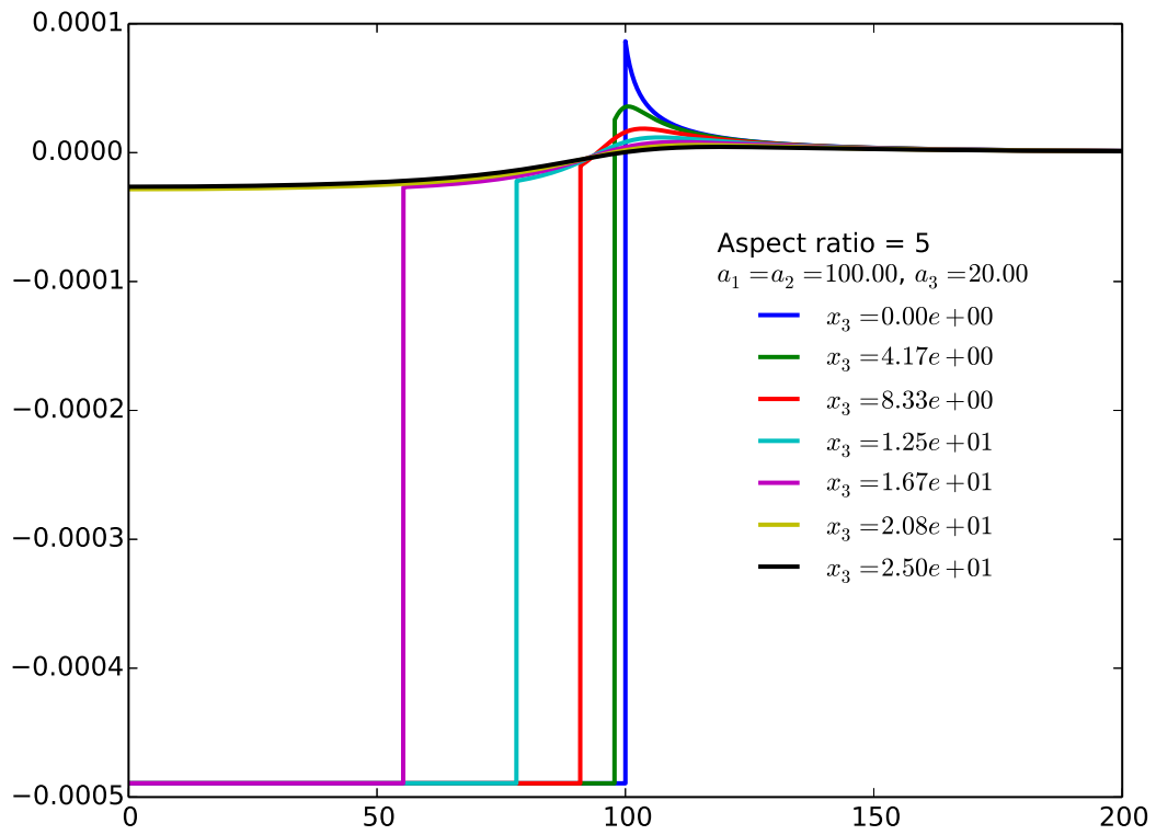
Figure 13: Oblate ellipsoid ( a_1 = a_2 = 100.0 , a_3 = a_1/h , h = 5 ); pressure p versus x_1 .
