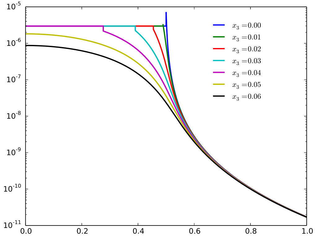
Figure 6: Prolate ellipsoid; energy density versus x_1 , x_2 = 0
