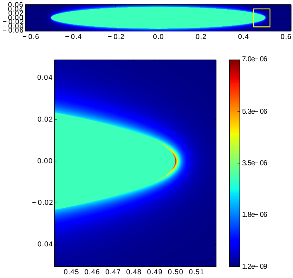
Figure 10: Prolate ellipsoid; energy density; top ' x_1 - x_3 ' plane at x_2 = 0 , bottom zoom window.
