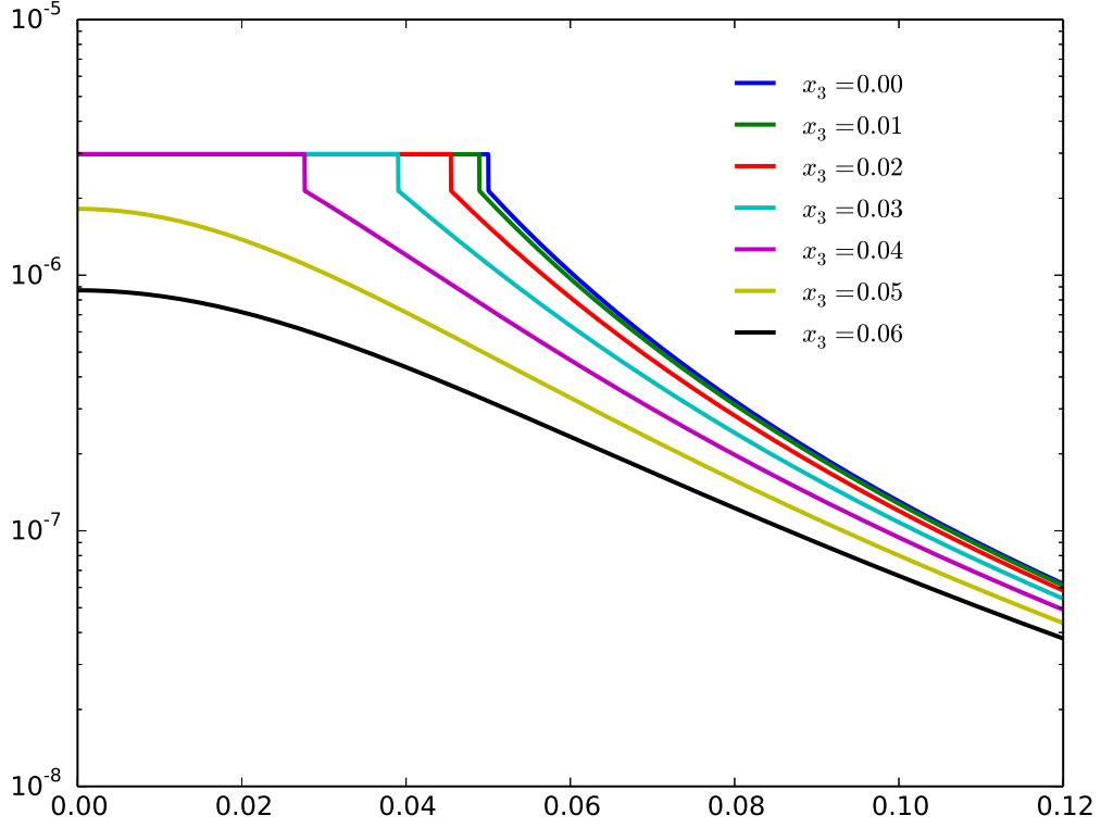
Figure 8: Prolate ellipsoid; energy density versus zoomed x_2 , x_1 = 0
