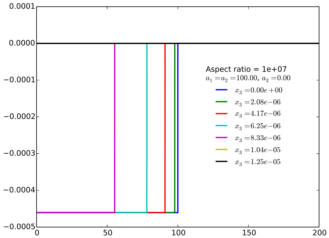
Figure 14: Oblate ellipsoid ( a_1 = a_2 = 100.0, a_3 = a_1/h, h = 1 \times 10^7 ); pressure p versus x_1 .
