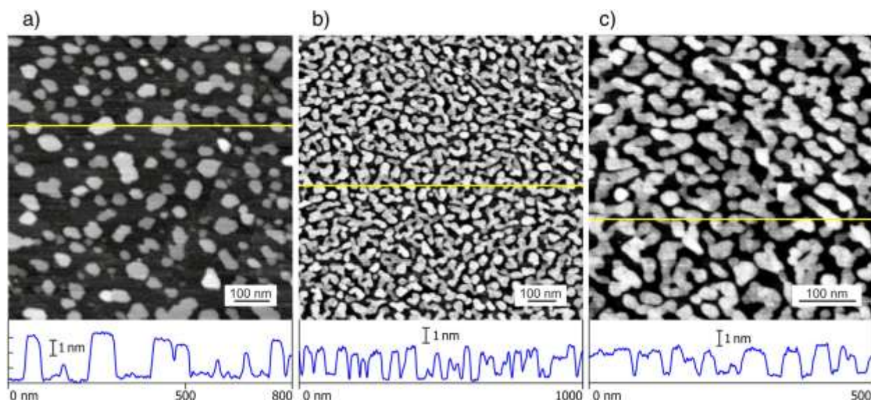
Figure 6-1. Co-deposition of water and methane. (a) 800 nm \times 800 nm STM image of Pt(111) after 8 min simultaneous exposure at 140 K to 5 \times 10^{-9} mbar water and 10^{-5} mbar of methane. (b,c) STM images of a film grown via 15 min co-deposition of 5 \times 10^{-9} mbar water and 0.1 mbar of methane. Fields of view are 1 \mu\text{m}^2 and 500 \text{ nm} \times 500 \text{ nm} , respectively. None of the images reveal any evidence of clathrate formation; pure water-ice films evolved instead.
