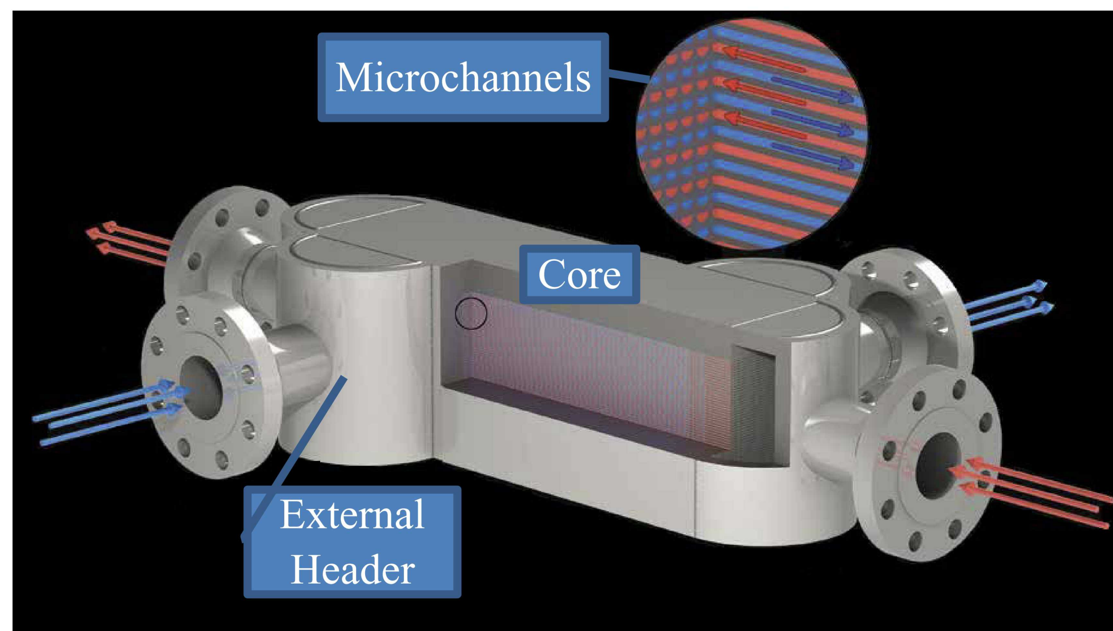
Microchannel heat exchanger configuration with semi-circular headers, [VPE]
