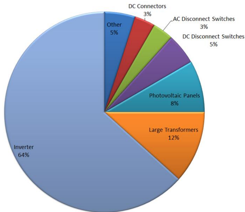
Figure 7. Component Contribution to System Energy Loss – Example
