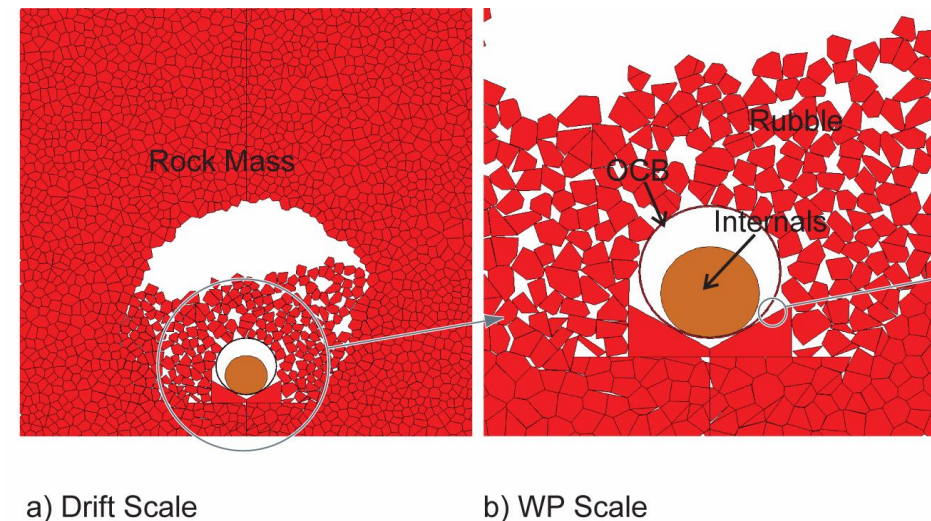
Below Model for Rubble-Waste Package Interactions (DOE/RW- 0573 Rev. 1, Figure 2.3.4-88)
