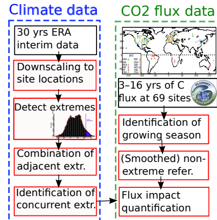
Figure 2. Conceptual overview of the different data streams and successive steps of our analysis.
