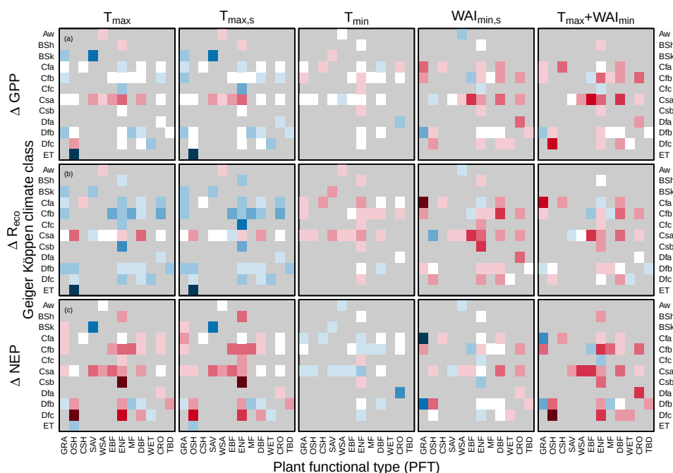
Figure 7. Z-transformed flux differences Differences between z -transformed CO 2 fluxes during extreme events and reference periods for the different extreme-event types and the different fluxes ( \Delta z = z_{\text{extr}} - z_{\text{ref}} ; see Eqs. 2 and 3 for details) of the different extreme-event types on GPP, R_{\text{eco}} and NEP (rows 1–3) separated according to plant functional types (PFT) (x axis in each plot; see Table A1 for the abbreviations used) and Geiger–Köppen climate class (y axis in each plot; see Table A2 for the abbreviations used) for different types of extreme events (columns 1–5: heat ( T_{\text{max}} ), heat alone ( T_{\text{max},s} ), cold ( T_{\text{min},s} ), drought alone ( \text{WAI}_{\text{min},s} ), and combined heat and drought ( T_{\text{max}} + \text{WAI}_{\text{min}} )). Shades of red indicate reductions of different size in the respective fluxes; shades of blue indicate increases. Refer to Figs. 5 and 6 for a visualization or quantification of the actual magnitude of these impacts.
