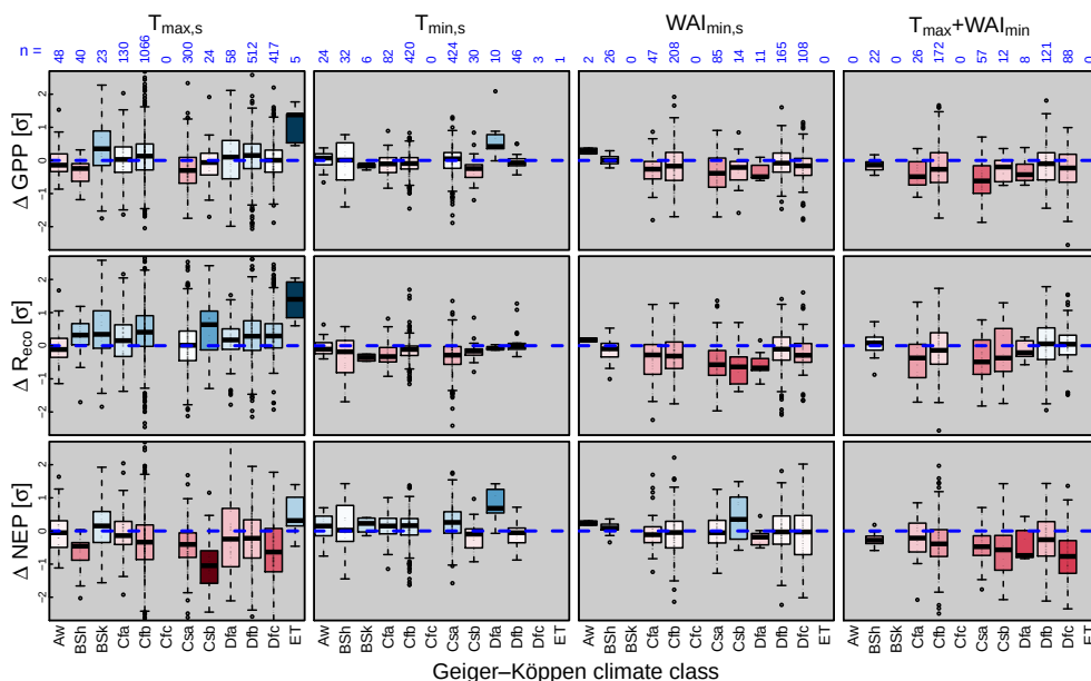
Figure 6. The influence of the ecosystem's ecoclimatic zone on the extreme-event impact. Shown are the differences between z -transformed CO 2 fluxes during extreme events and reference periods ( \Delta z = z_{\text{extr}} - z_{\text{ref}} ; see Eqs. 2 and 3 for details) for the different extreme-event types and the different fluxes according to the Geiger-Köppen climate class (Table A2 for the abbreviations used) of the respective ecosystem. (See Fig. 4 for a detailed description of the box plots shown.)
