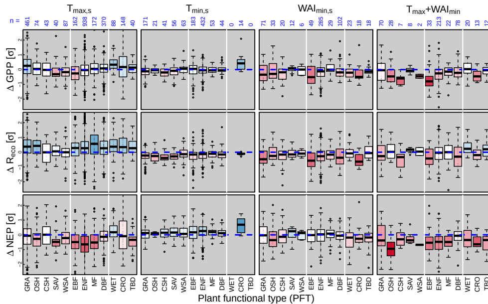
Figure 5. The influence of the ecosystem's plant functional type (PFT) on the extreme-event impact. Shown are the differences between z -transformed CO 2 fluxes during extreme events and reference periods for the different extreme-event types and the different fluxes ( \Delta z = z_{\text{extr}} - z_{\text{ref}} ; see Eqs. 2 and 3 for details) according to the PFT (see Table A1 for the abbreviations used) of the respective ecosystem (Fig. 4 for a detailed description of the box plots shown).
