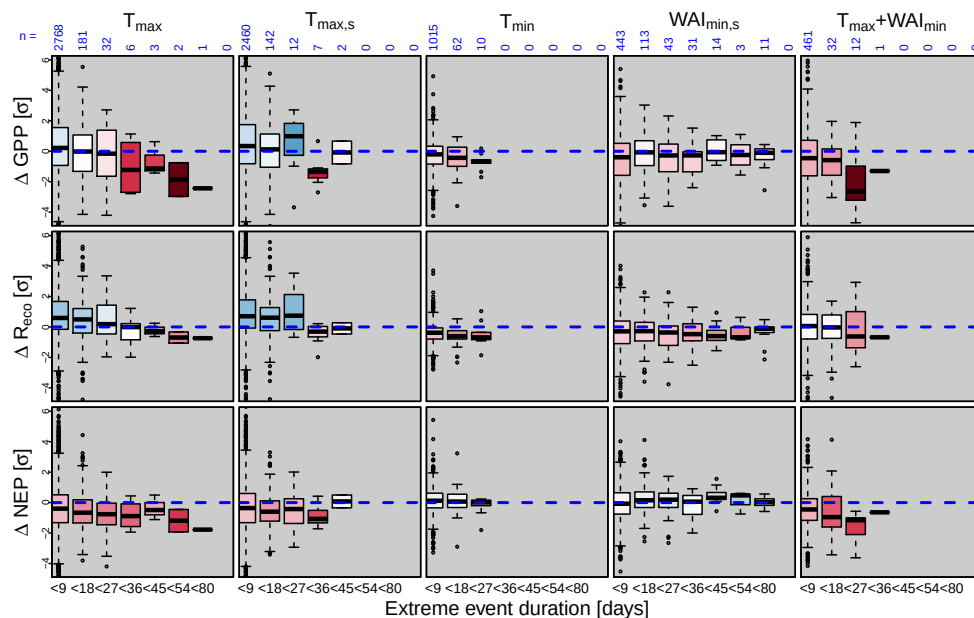
Figure 4. Influence of extreme-event duration on extreme-event impact. Shown are normalized flux differences between extreme events and a reference period ( \Delta z = z_{\text{extr}} - z_{\text{ref}} ; see Eqs. 2 and 3 for details) for gross primary production (GPP), ecosystem respiration ( R_{\text{eco}} ) and net ecosystem production (NEP) (in rows 1–3) for a selection of different extreme-event types (in columns 1–5: heat ( T_{\text{max}} ), heat only ( T_{\text{max},s} ), cold ( T_{\text{min}} ), drought only ( \text{WAI}_{\text{min},s} ), and combined drought and heat ( T_{\text{max}} + \text{WAI}_{\text{min}} ); see Table 1 for details on all extreme types). Blue numbers at the top margin of the figure denote the amount of extreme events in each class. Blue numbers at the top margin of the figure denote the amount of extreme events in each class.
