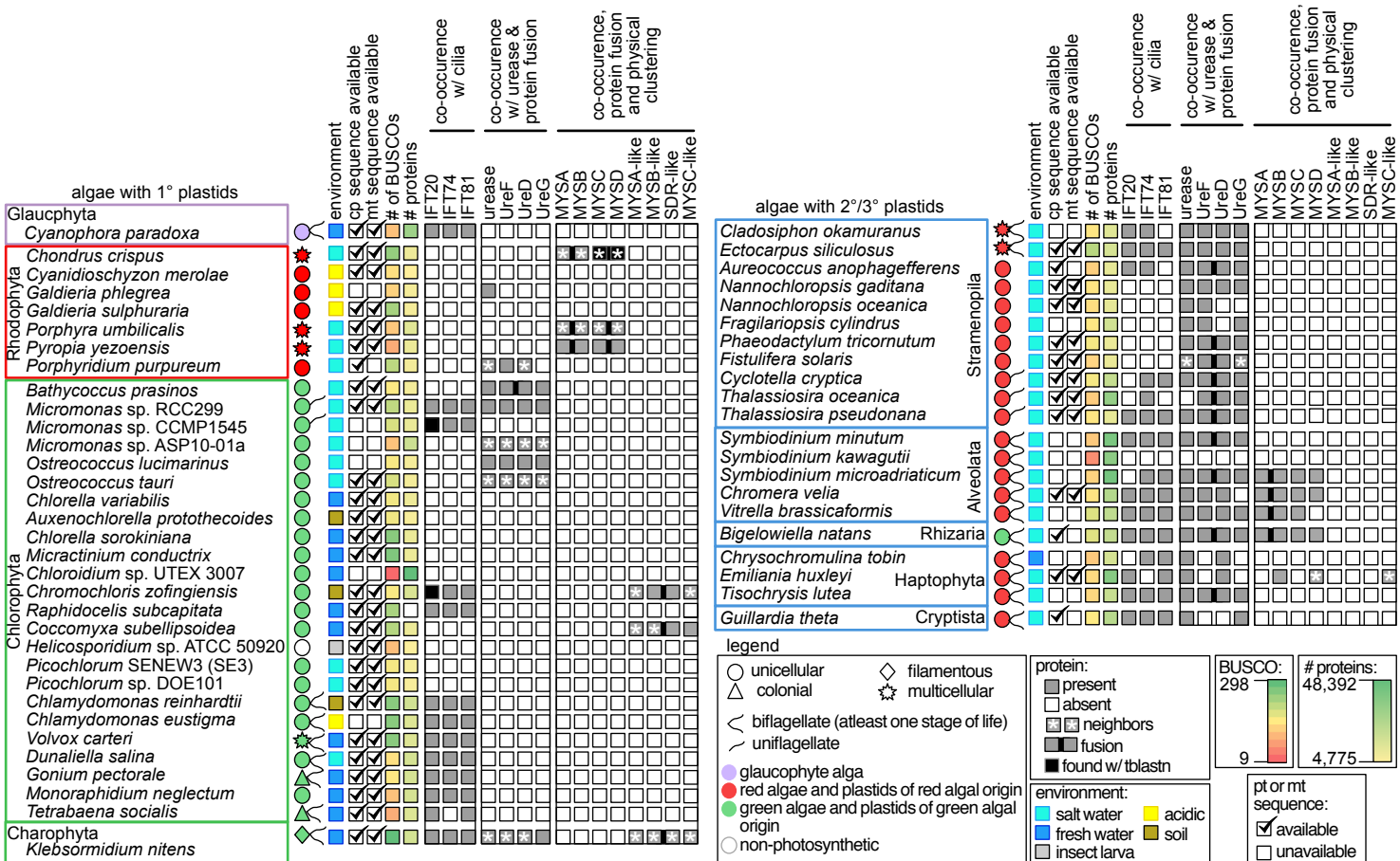
Figure 4. A list of published algal proteomes predicted from whole-genome sequencing projects (as of June 2018). Citations for each genome are available in Table 1. Icons to the right of the name designate cellularity, whether the alga has cilia, and whether the alga (or the origin of the plastid from algae with 2/3 plastids) is from the glaucophyte, red, or green lineage. Helicosporidium sp. ATCC 50920 is from the Chlorophyta lineage but has recently lost photosynthetic capacity (211). The most common environment from which each alga has been isolated is also given. For most, but not all algae listed, both the chloroplast-localized (cp) and mitochondrion-localized (mt) genome sequences are also publicly available; availability is indicated with a checked box. The quality/completeness of the predicted proteome is indicated with a heatmap representing the number of complete BUSCOs detected (out of 303). The number of total proteins in each proteome is also shown as a heatmap. Phylogenetic profiles require high quality genomes and gene models for confidence that the absence of a gene is due to evolution rather than a gap in the sequence. For instance, the Galdieria phlegrea urease assembly factors were found by targeted sequencing (174), but these genes are not present in the public genome sequence. In some cases, a missing protein is due to an inaccurate gene model and can be recovered by searching the genome with tblastn. Whether a gene/protein was lost (or never acquired) instead of missing from the assembly can be better predicted if that gene/protein is also missing from closely related whole-genomes (for instance from the same genus). Additionally, the absence of functionally related proteins, such as cohorts in the same pathway, can provide support for gene loss. Comparative genomics-based analyses present hypotheses about the biology of organisms. As an example, protein components of intraflagellar transport (IFT, 3 components are shown here) are only encoded by genomes belonging to algae that have cilia. Although cilia have not been described in C. zofingiensis and Raphidocelis subcapitata , the presence of genes related to cilia biogenesis and biology supports the presence of cilia in a yet to be described stage of life (188). The co-occurrence of urease and assembly factors provide an example of how proteins that interact with each other in the cell co-occur. As seen previously, two or more proteins may be fused and proteins may be encoded by genes that are next door to one another in the genome. Both of these observations strengthen functional association between these enzymes. Although neighborhoods of functionally related genes are thought not to be as prevalent in eukaryotic genomes as in prokaryotes (because eukaryotes typically lack polycistronic mRNA), physical proximity of some functionally related genes has been observed in algal genomes, as shown here for genes encoding urease and assembly factors and for genes predicted to be responsible for biosynthesis of UV-absorbing/screening mycosporine-like amino acids (MAAs) (32). Orthology between red algal MAA-biosynthesis proteins with related proteins in green algae is not clear, but physical clustering of the corresponding genes supports a functional link between these green algal homologs, which leads to the prediction that these proteins may be responsible for MAA biosynthesis or, likely, a similar product since the MYSB homolog is uniquely fused to a protein from the short-chain dehydrogenases/reductases (SDR) family. While protein fusions can be an artifact of inaccurate gene models, the presence of at least two protein fusions from independent genomes is a good indication that the fusion is real.
