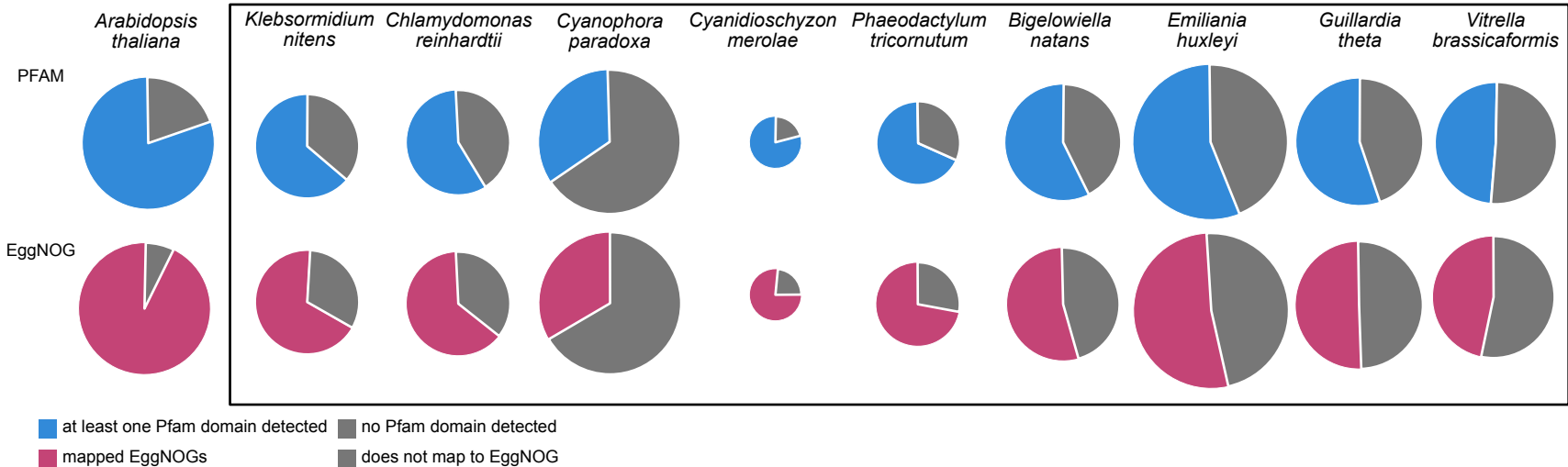
Figure 3. Algal genomes provide a reservoir of undiscovered functional capabilities. As an indicator of the amount of protein function yet to be discovered in algae, the number of predicted proteins from each whole-genome sequence, which contains at least one Pfam-A domain (using hmmsearch with Pfam trusted score cutoffs) (81) or maps to an orthologous group from the EggNOG database using DIAMOND (113), is shown. For comparison, the same analyses for the choice reference land plant Arabidopsis thaliana is also shown. The pie charts are scaled relative to the total size of each predicted proteome. For each of the major lineages of algae (streptophyte algae, chlorophyte algae, glaucophytes, red algae, stramenopiles, rhizarians, haptophytes, cryptophytes and alveolates) only one representative is shown and was chosen as having the highest number of complete BUSCOs compared to other predicted proteomes from closely related algae. Although the proportion of each proteome that maps to Pfam or EggNOG is roughly similar, the two are not perfectly overlapping. For instance, for C. paradoxa , about 2,300 proteins have at least one Pfam domain but do not map to EggNOG, while about 2,200 proteins map to EggNOG but do not have a Pfam domain. These analyses are conservative and serve to illustrate the distance between algal proteomes and sequences presently in databases. For instance, a more sensitive method, Domain Annotation by a Multi-objective Approach (DAMA) and CLADE, was recently used to detect conserved domains in 99% of the proteins in P. tricornutum (178). Assessing the number of proteins in these algae where the function is known or can be confidently predicted based on sequence similarity to a database such as NCBI's RefSeq (172), Uniprot (47), EggNOG or a match to Pfam's domain models is difficult/impossible to determine quantitatively. As part of Gene Ontology's Reference Genome Project (89), a comprehensive set of GO annotations for the A. thaliana genome is available, and, as of 2018, 30% of the genes in the A. thaliana genome is associated with an experimentally supported GO term for either molecular function or biological process (39).
