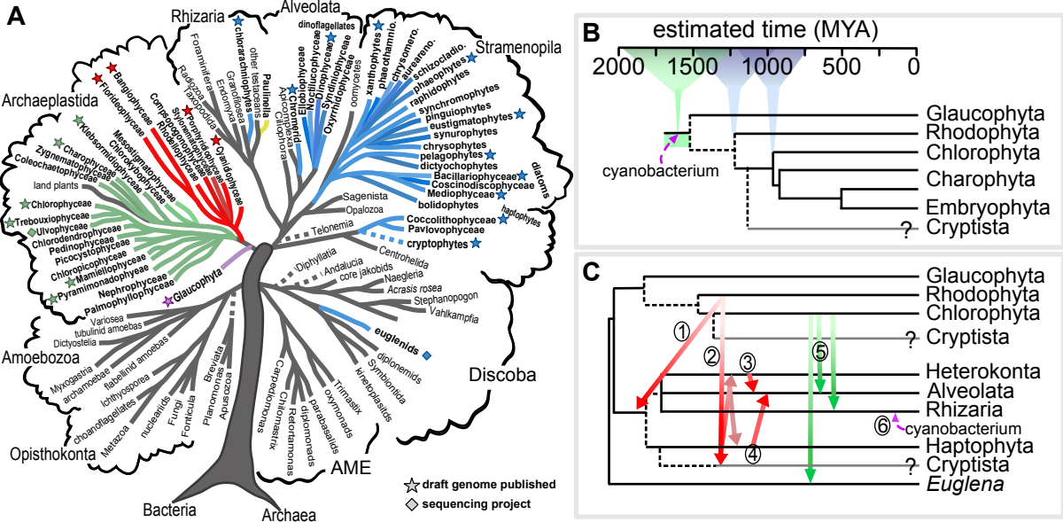
Figure 1. A , a cartoon depiction of the eukaryotic tree of life adapted from Baldauf, 2003 (15) and incorporating phylogenetic relationships of algal classes from (62; 123; 233). Branches containing algae are colored green for green algae from Chlorophyta and Streptophyta, red for rhodophytes, purple for glaucophytes and blue for algae whose photosynthetic plastids are derived from endosymbiosis of a eukaryotic alga (i.e. secondary or tertiary endosymbiosis). For each lineage of algae shown in the tree, the presence of at least one publicly released whole-genome sequence or sequencing project is indicated with a star or diamond, respectively. B , the major lineages of Archaeplastida. The ranges of estimated time MYA (million years ago) for the endosymbiotic event (green) and last common ancestors (blue) are based on molecular clock estimates from (66; 92; 101; 102; 104; 115; 127; 190; 237; 241). Affinity between Cryptista and Archaeplastida observed in (36) is represented with a dotted line. Of the algal lineages within Archaeplastida, Charophyta, which contains the streptophyte algae, is polyphyletic. C , various theories for the transfer of plastids and genes from Archaeplastida to protists: 1, the chromalveolate hypothesis proposed by Cavalier-Smith (43) suggests that endosymbiosis of a red alga happened only once in a common ancestor of algae bearing chlorophyll c -containing plastids, with all non-plastid relatives being examples of “former algae”. 2, in recent years, the chromalveolate hypothesis has been superseded by higher order eukaryote-to-eukaryote hypotheses. Shown here is the cryptophyte-first hypothesis proposed by Stiller, et al. (207), where a cryptophyte was the original host of a red alga-derived plastid, which was subsequently spread to an ancestral ochrophyte within Heterokonta then to haptophytes. 3, as an example of an extension of the cryptophyte-first hypothesis, the Vitrella brassicaformis plastid may be derived from an ochrophyte (195). 4, the modern-day plastid in dinoflagellates from Karenia is derived from a haptophyte, which replaced the peridinin plastid that is found in other dinoflagellates. 5, three independent events between green algae and protists. 6, Paulinella chromatophores are derived from endosymbiosis of a cyanobacterium.
