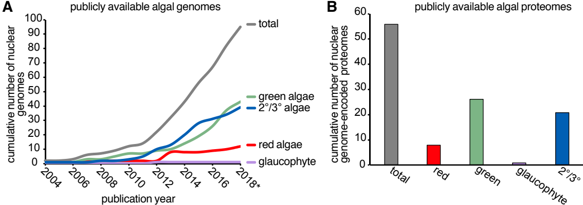
Figure 2. As second- and third-generation sequencing technologies have increased the speed and decreased the cost of whole-genome sequencing, access to algal nuclear genomes is growing. A , the cumulative number of publications that report the sequencing of a nuclear genome from the algal group is given (total) and the cumulative number of genomes for each of the major algal lineages. The asterisk signifies as of June 2018. B , roughly half of these genome-sequencing projects are accompanied by a public release of gene models and predicted protein sequences.
