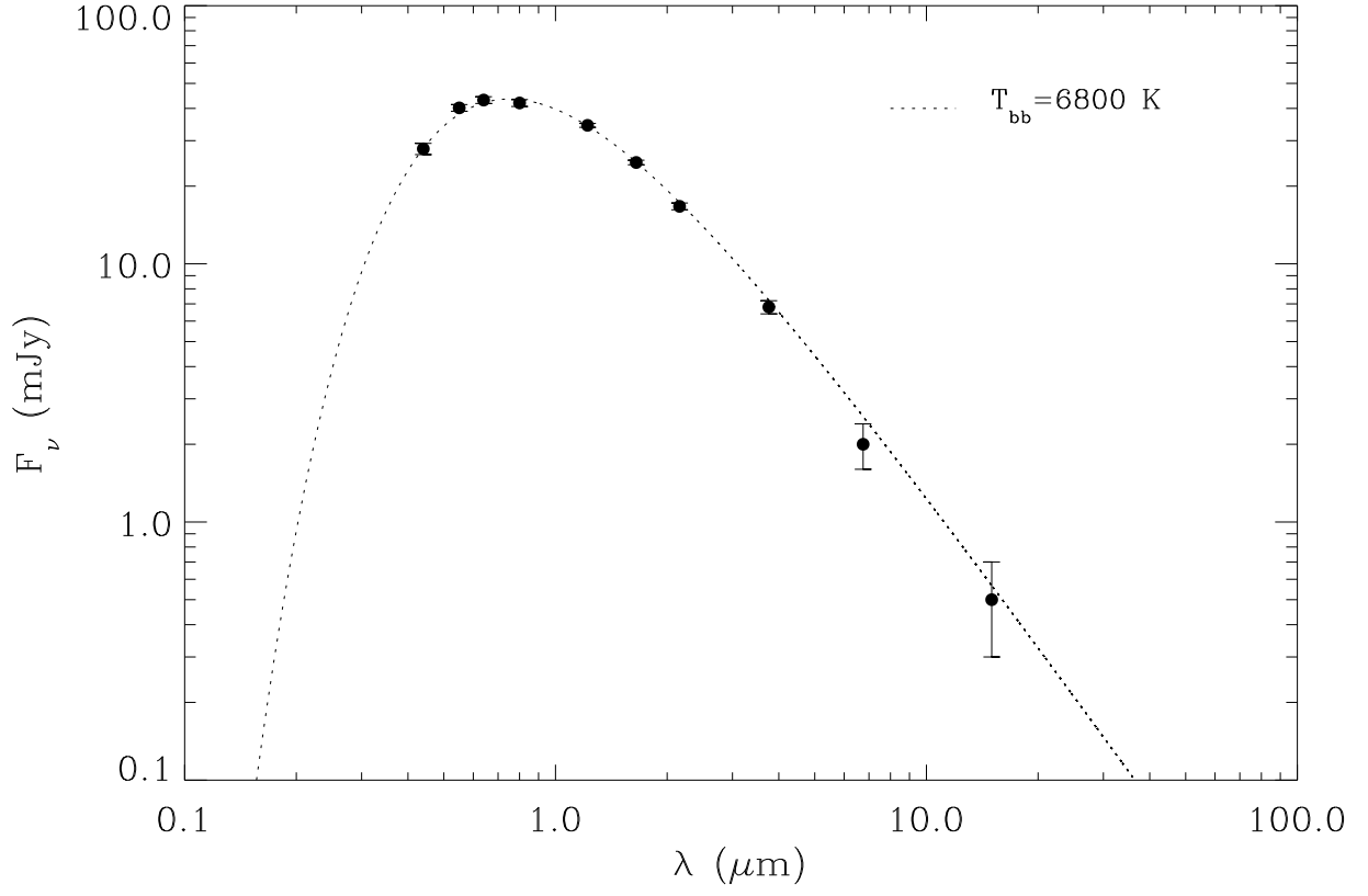
Fig. 3.— Spectral energy distribution of van Maanen 2 from the data in Table 1. Overplotted is a 6800 K blackbody demonstrating that the data reveal no excess emission in the infrared and are consistent with a single star.
