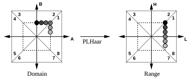
Figure 3. The PLHaar transform's rotation in L_\infty space. Numbered octants are shown.
