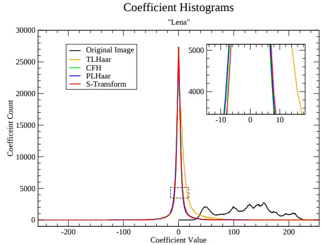
Figure 9. Histograms of the “Lena” image, and the S-Transform, PLHaar, TLHaar, and CFH coefficients.
