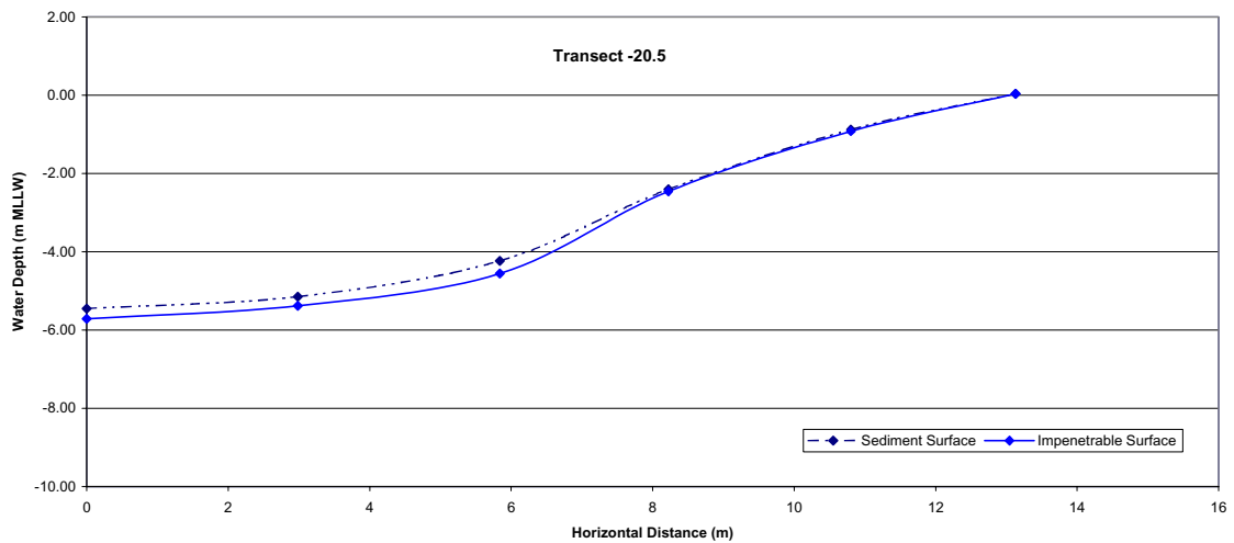
Figure 3-14. Underwater Survey Profiles for Transects -12.5, -16.5, and -20.5
