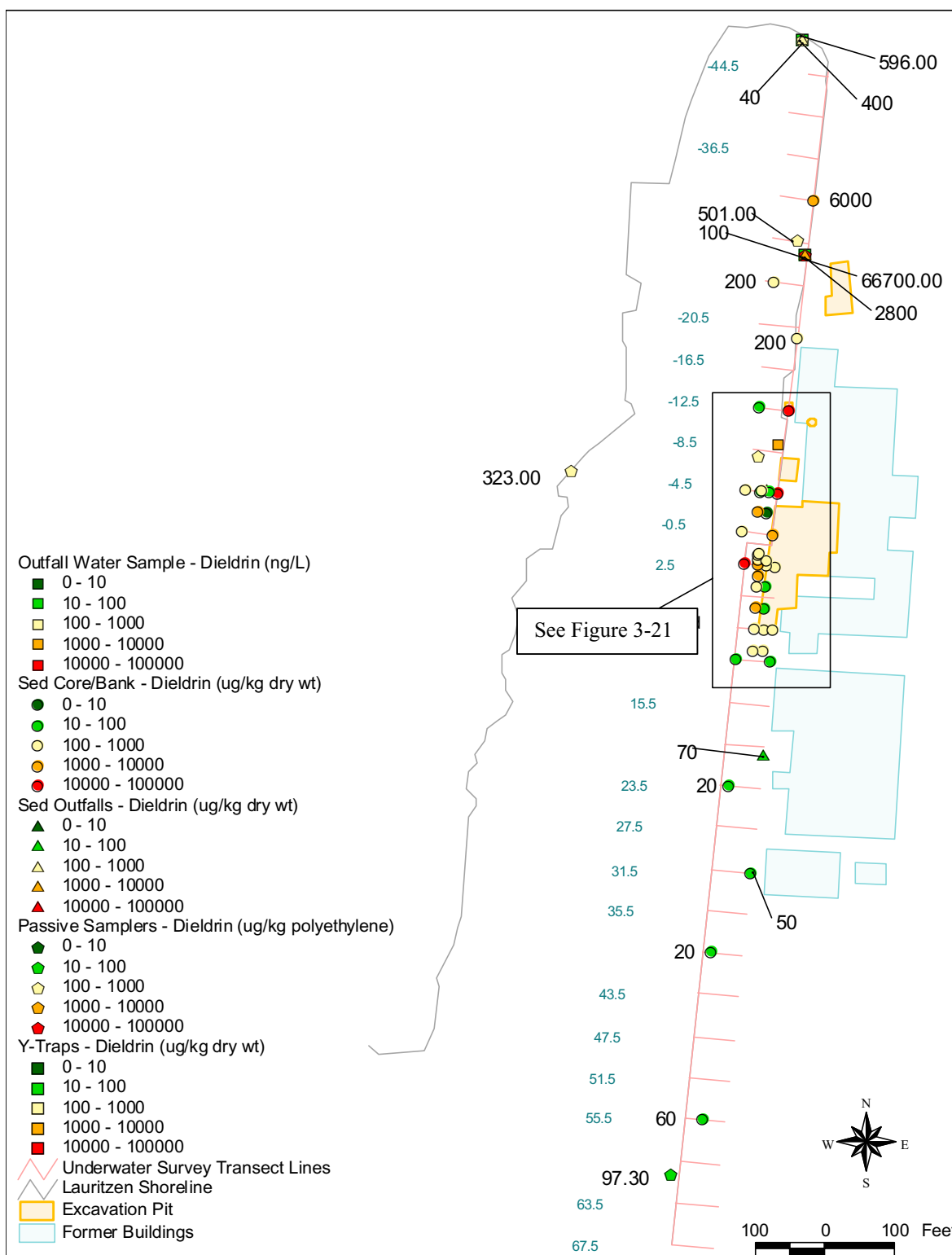
Figure 3-20. Dieldrin Concentrations in Sediment Core and Embankment Soil Samples Throughout Lauritzen Channel
