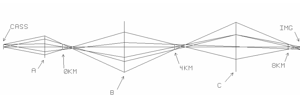
Figure 2- 22: A solution using flat DM's and the minimum number of optics (A, B, and C). The diameters of the optics are large (2.7m). The overall length is 92.3m.
