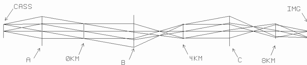
Figure 2- 20: A design using the minimum number of optics possible under the Hardy order-of-correction assumption. There are 3 optics in addition to the 3 DM's. Overall length is 35.6m.
