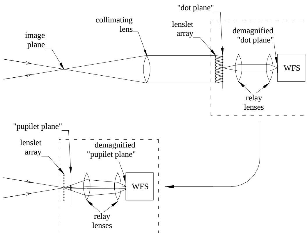
Figure 3- 17: Conversion of a SH WFS to a PWFS. Top figure: Converging light from the left comes to a focus and is then collimated by a collimating lens. The collimating lens creates a pupil downstream, where the lenslet array is placed. The lenslets produce a series of images or dots at the focal plane of the lenslets or “dot plane”. Subsequent relay optics scale the dots as appropriate for the WFS CCD. For clarity, light from only one dot is shown after the dot plane. Bottom figure: to convert SH WFS to PWFS, remove collimating lens and translate lenslet array, relay optics, and WFS CCD upstream until the lenslet array is at the focus of the incoming beam. The lenslets now produce “pupilets” at the lenslet focal plane, i.e., where the dots were in the top figure. Thus, the relay optics will relay the pupilets to the WFS CCD.
