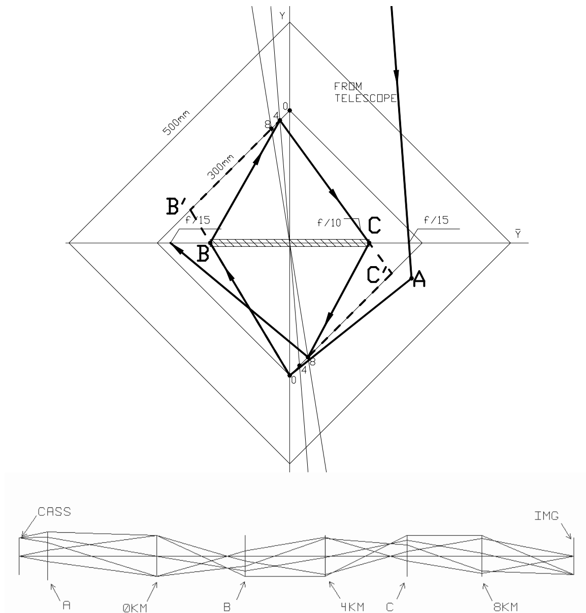
Figure 2- 21: Minimum length solution for minimum number of optics under Hardy constraints. The fact that B and C are at image planes may be problematic since any dust on these optics would appear in focus. This may be alleviated at a minor cost in length as shown by moving the relay optics away from the image plane, illustrated by the dashed line above. Some length could be reduced by moving “A” closer to the telescope focus; this position for “A” is used for clarity in the drawing. The overall lengths of these layouts are 20.8m and 23.4m.
