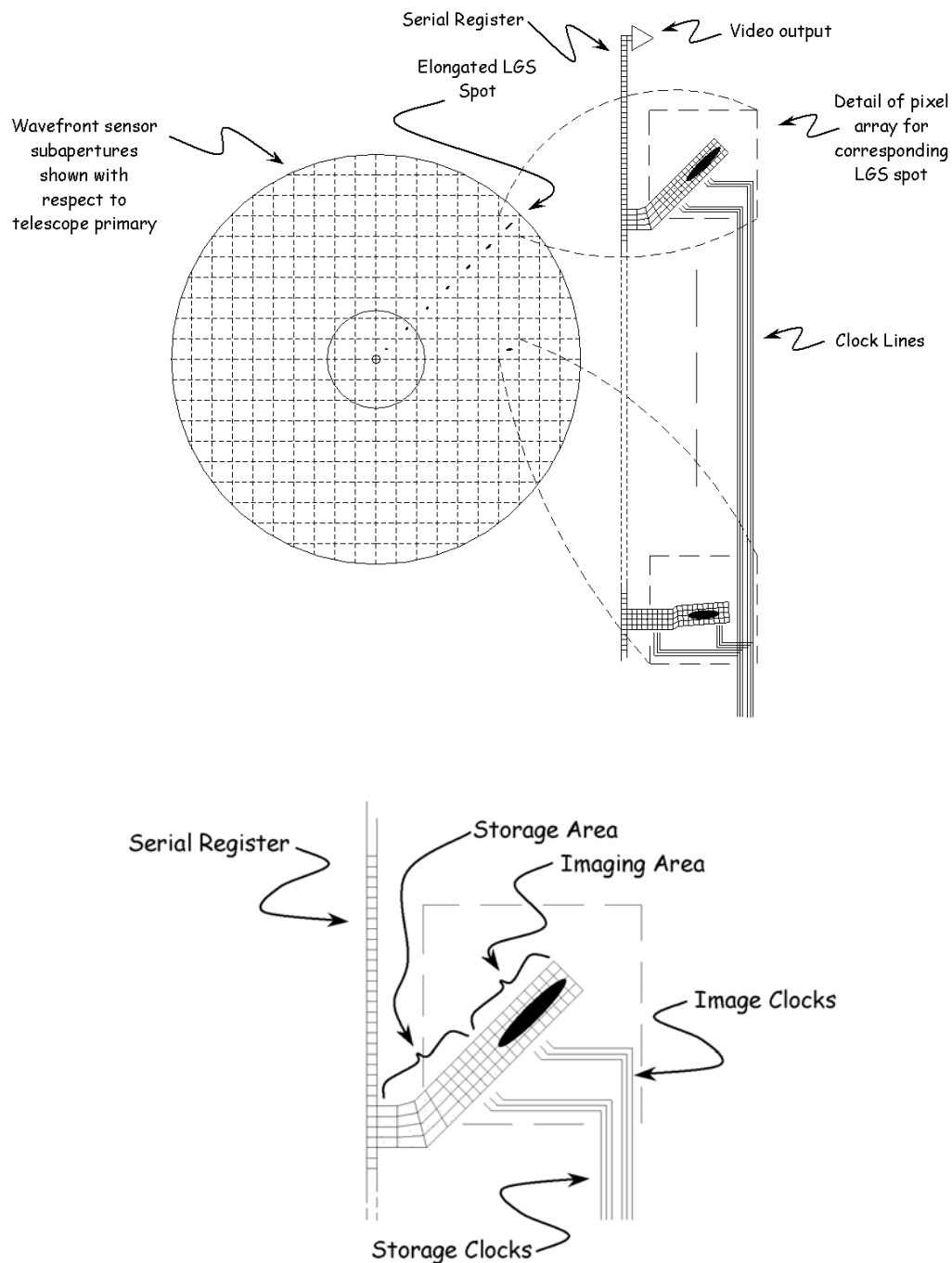
Figure 4- 10: Concept for WFS CCD customized for LGS spot elongation. Each subaperture presents a different size and orientation of LGS spot elongation. Each subaperture uses pixels that are aligned to the spot elongation for that subaperture. (from Beletic)
