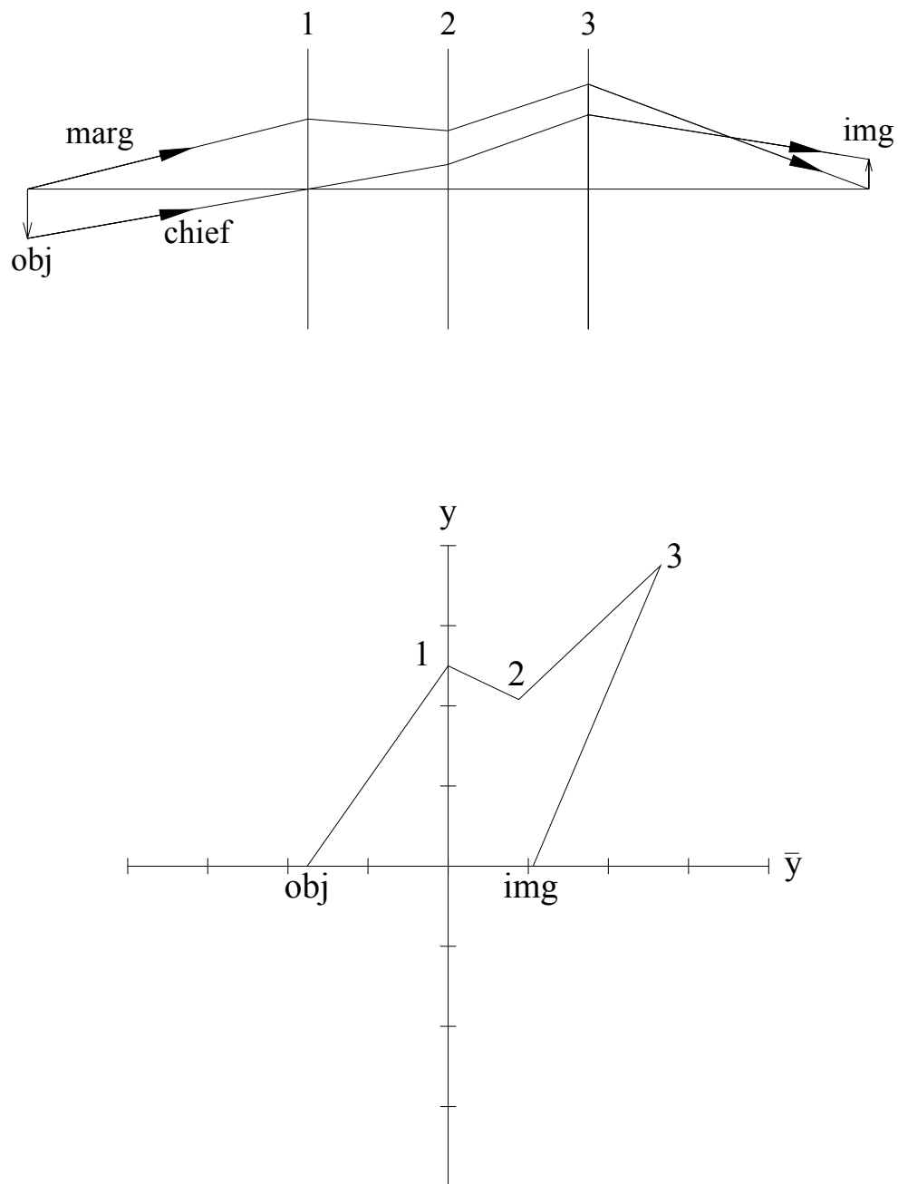
Figure 1- 8: A sample optical system in a conventional side-view (top) and as represented in a y, \bar{y} diagram (bottom).
