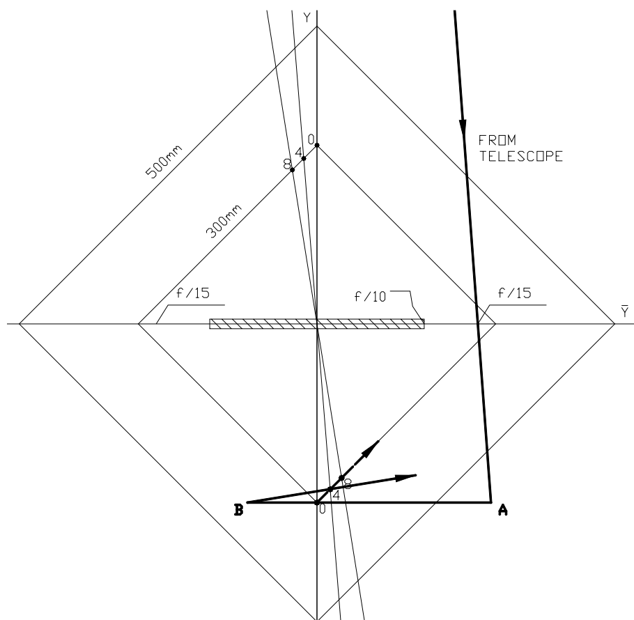
Figure 2- 13: Example of violating "sense of rotation" rule. The y, \bar{y} ray from A to B "picks up" the 0km DM, but the next segment (extending from B) that would pick up the 4km DM has the opposite sense of rotation about the origin, and so is not physically realizable. The y, \bar{y} ray from the telescope and from A to B has a clockwise rotation about the origin, whereas the ray from B to the 4km DM would be counter-clockwise. We can also see that any ray from the 0km DM to the 4km DM on the lower half of the diagram has counterclockwise rotation about the origin (ray from 0 to 4).
