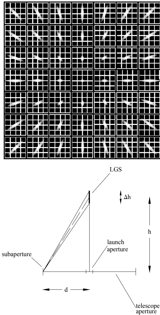
Figure 1- 7: (top) Schematic illustration of LGS spot elongation effect in a Shack-Hartmann WFS (from Goncharov). (bottom) Geometry of laser guide star showing spot elongation. The LGS, shown as a heavy line above the telescope, is located at an altitude of h with a depth of \Delta h . The elongation varies with the distance of the subaperture from the launch aperture ( d ); the left-most subaperture shown here. The angular elongation from the perspective of this subaperture is \Delta\theta = (\Delta h/h)(d/h) = \Delta h d / h^2 .
