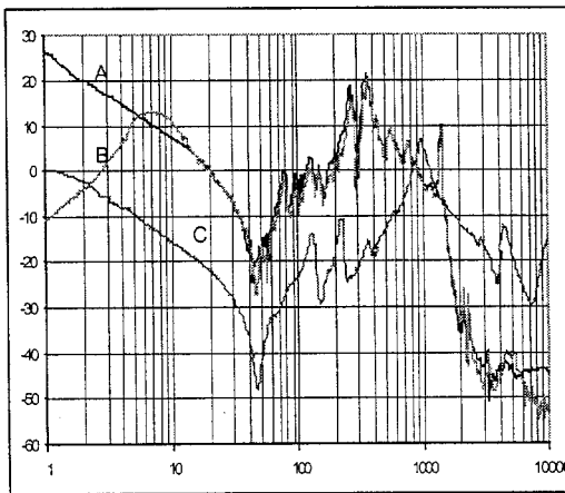
Figure 4. Capstan Drive Velocity Loop Transfer TFs
