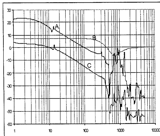
Figure 3. Velocity Loop Transfer Functions (TFs)
