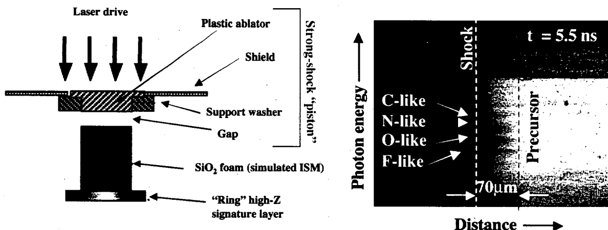
Figure 6. The schematic on the left shows a radiative shock experiment fielded on Omega. Spectrally resolved precursor shock data in silica foam is shown on the right.
