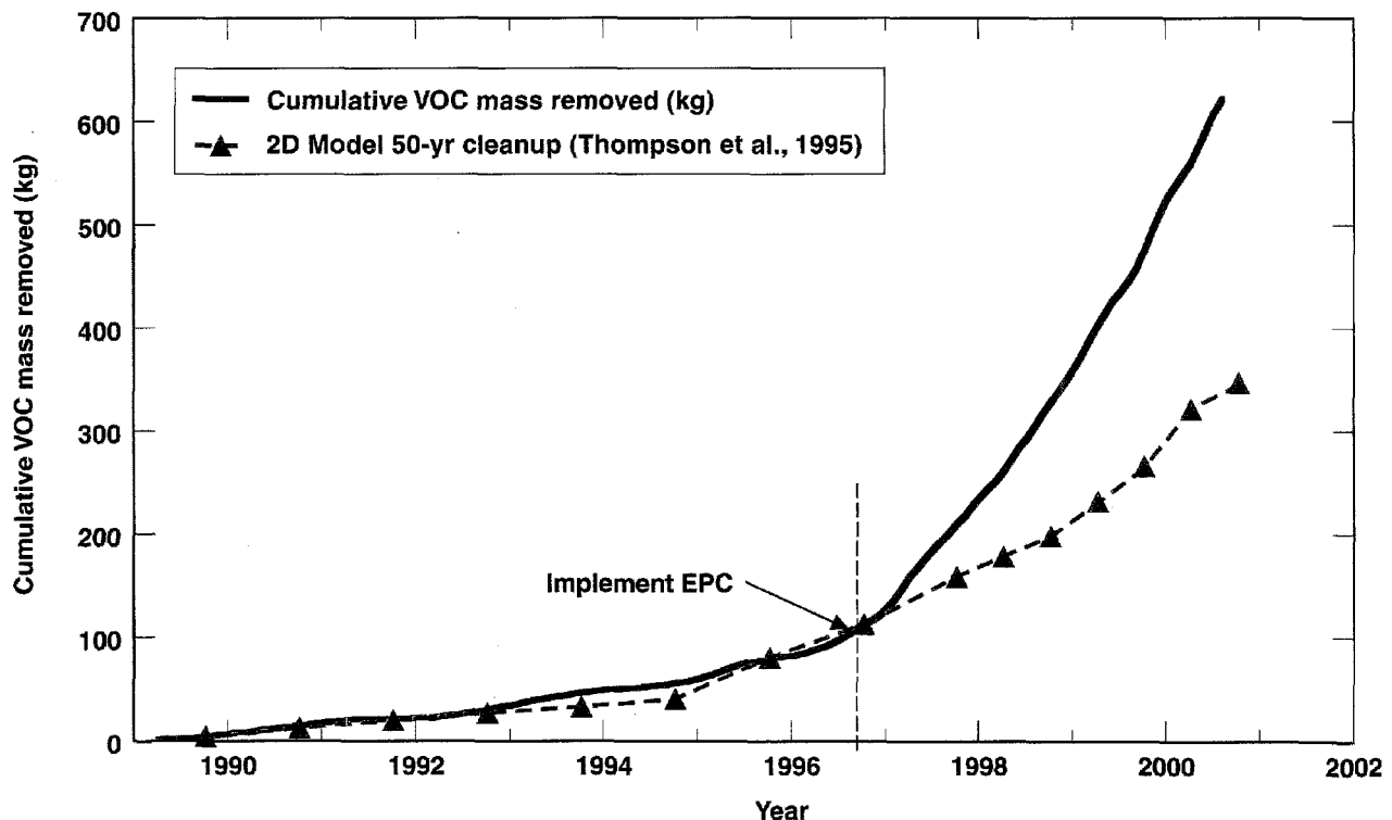
Figure 3. Engineered Plume Collapse (EPC) is rapidly removing mass.
