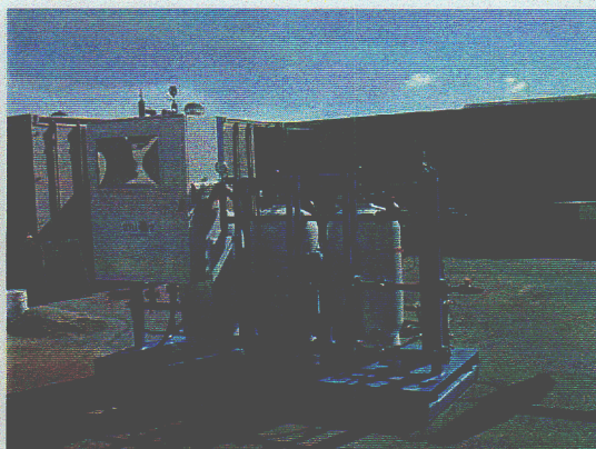
Granular Activated Treatment Unit (GTU)
