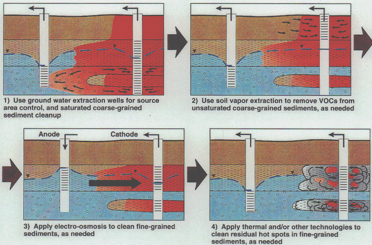
Figure 4. Phased Source Remediation (PSR) strategy.
