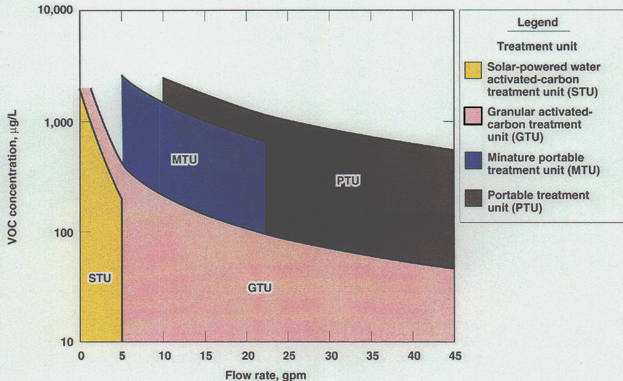
Figure 2. Treatment unit options.
