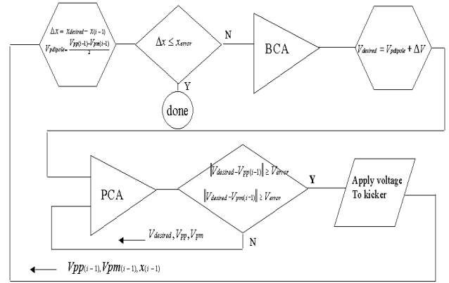
Figure 3 Kicker Control System
