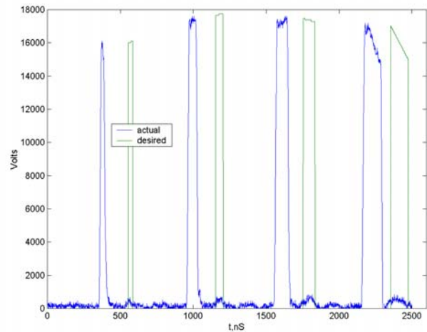
Figure 7 Four-pulse burst with amplitude modulation
