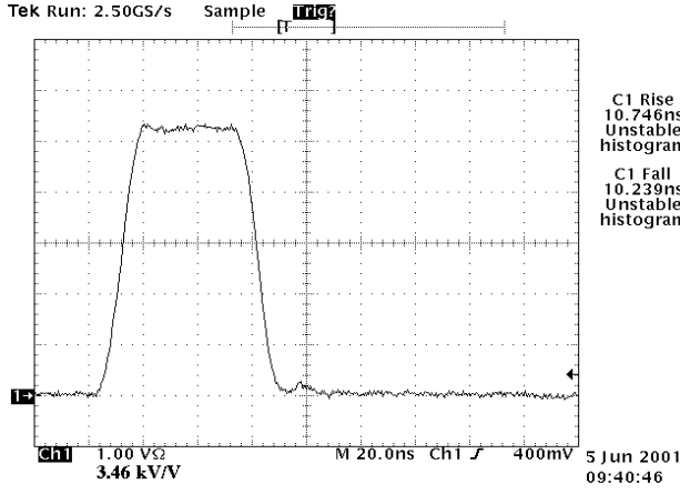
Figure 2 Modulator output voltage
