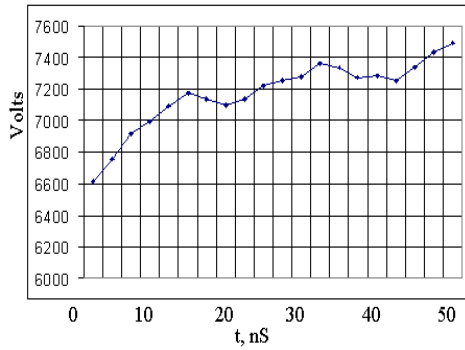
Figure 4b Modulator output
