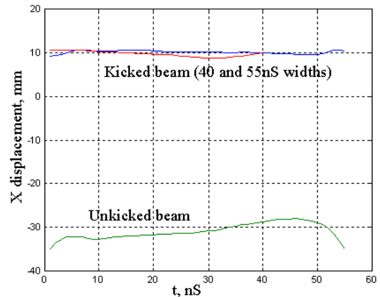
Figure 4a kicked and un-kicked beam position for 40 and 55ns wide beam pulses on ETAII
