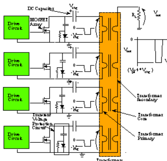
Figure 1 Solid-state modulator and block diagram
