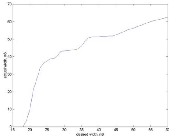
Figure 5 MOSFET switch output pulsewidth versus desired width
