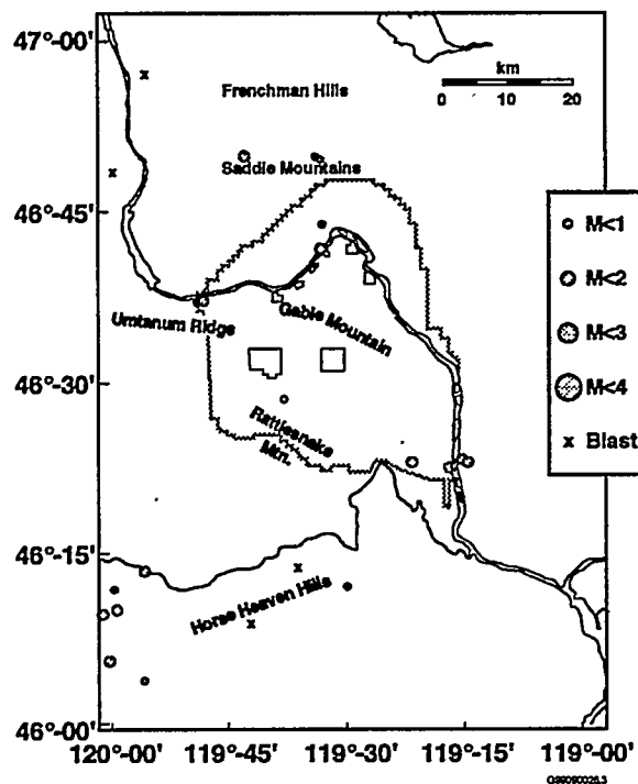
Figure 4.4. Locations of all Events that Occurred Between October 1, 1998 and September 21, 1999 Shown by Quarter (Coda Length Magnitude ( M_c ) scale is shown at the side of the map)
