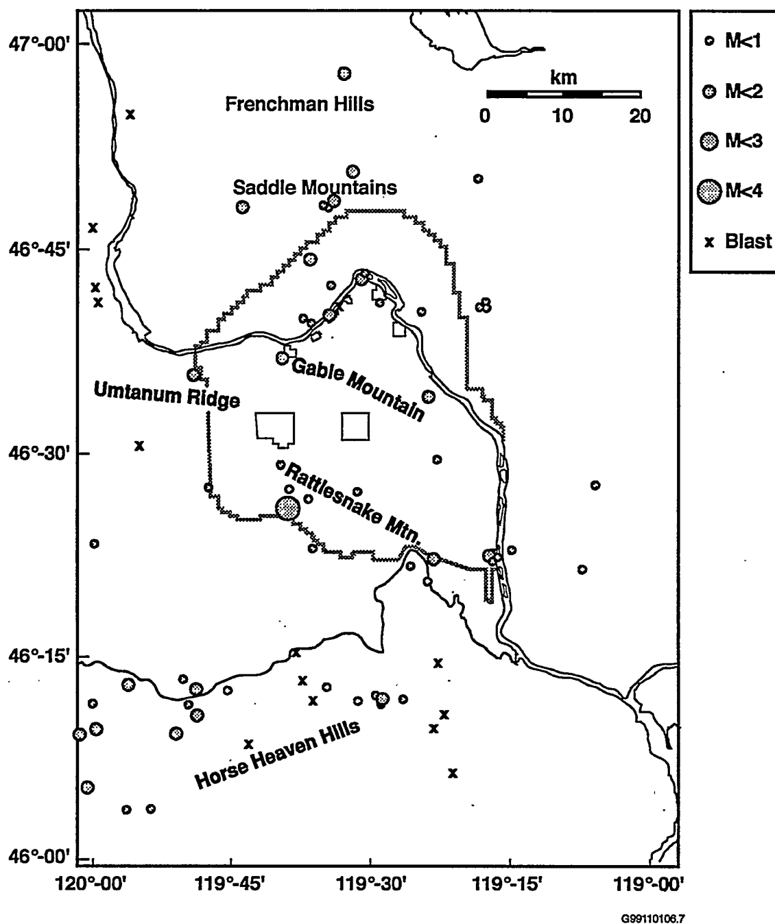
Figure 4.5. Locations of all Events Recorded During FY 1999
