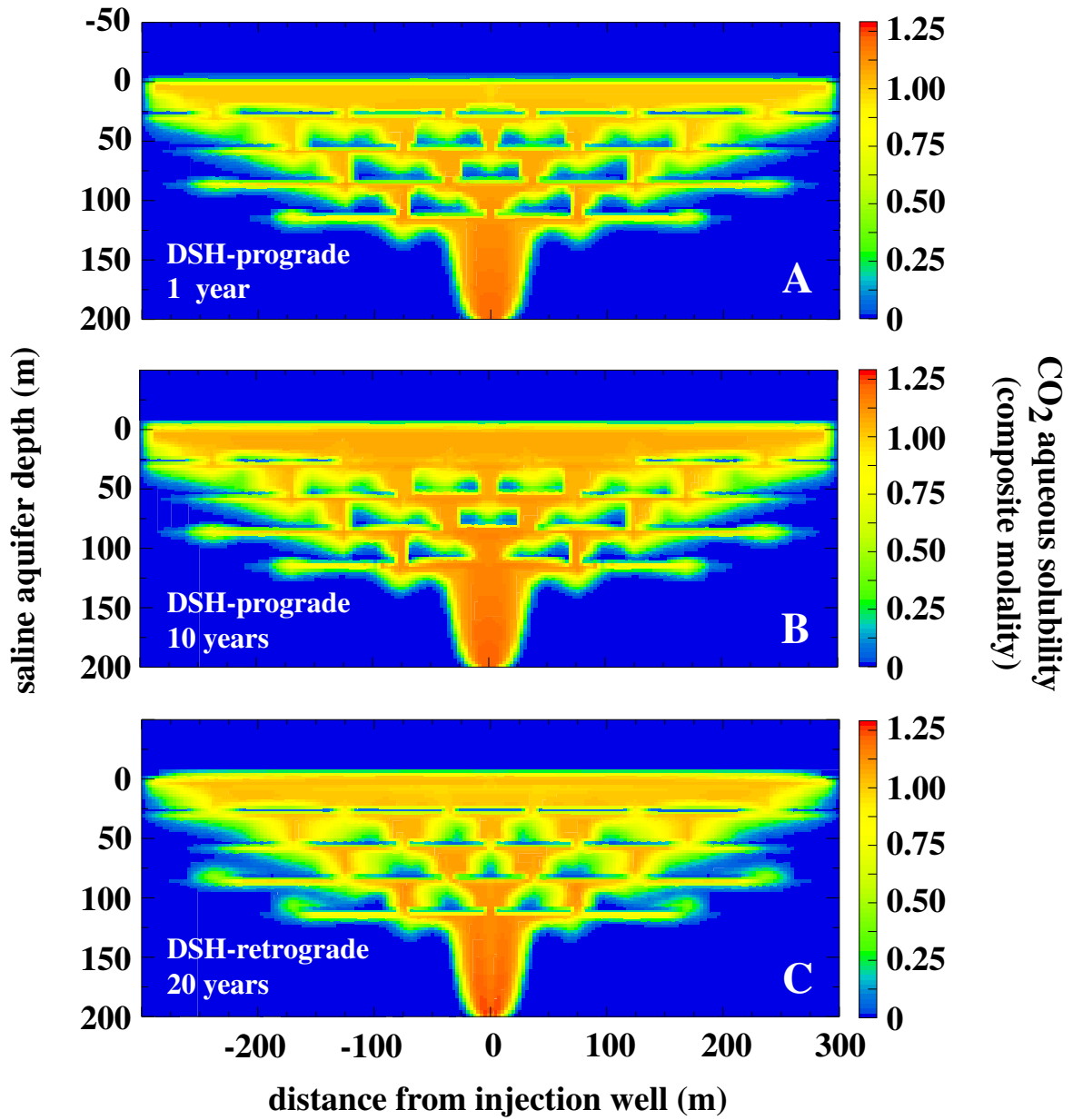
Figure 9: Evolution of \text{CO}_2 aqueous solubility (composite molality of all carbon-bearing aqueous solutes) in model DSH during prograde (1 and 10 years) and retrograde (20 years) sequestration.
