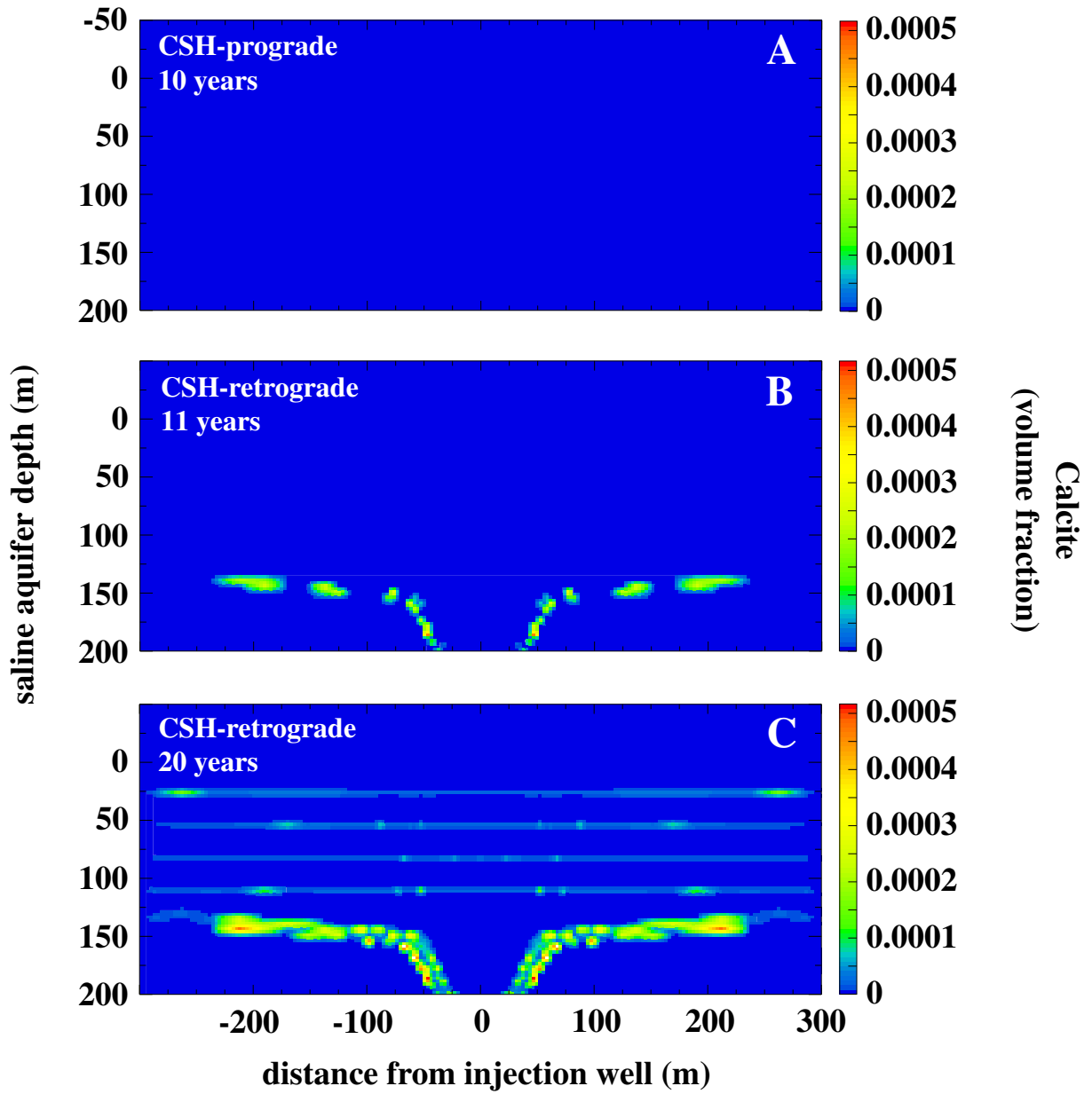
Figure 20: Evolution of Calcite [\text{CaCO}_3] precipitation within the saline aquifer and intra-aquifer shales of model CSH during prograde (10 years, no precipitation) and retrograde (11 and 20 years) sequestration.
