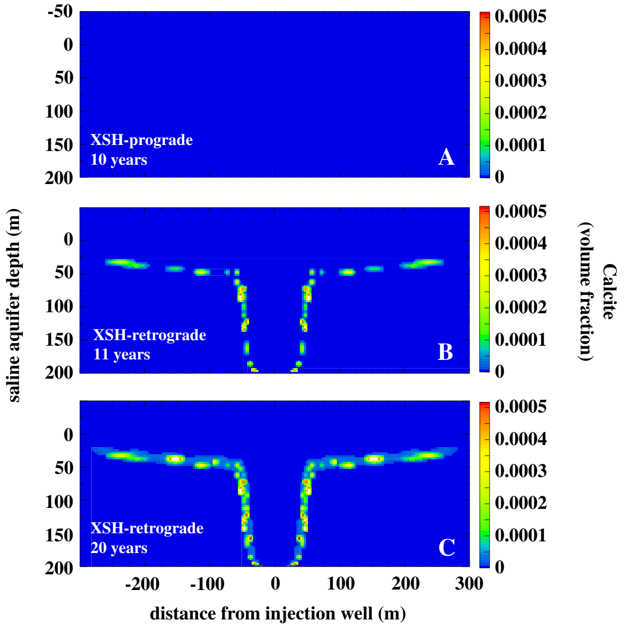
Figure 19: Evolution of Calcite [\text{CaCO}_3] precipitation within the saline aquifer of model XSH during prograde (10 years, no precipitation) and retrograde (11 and 20 years) sequestration.
