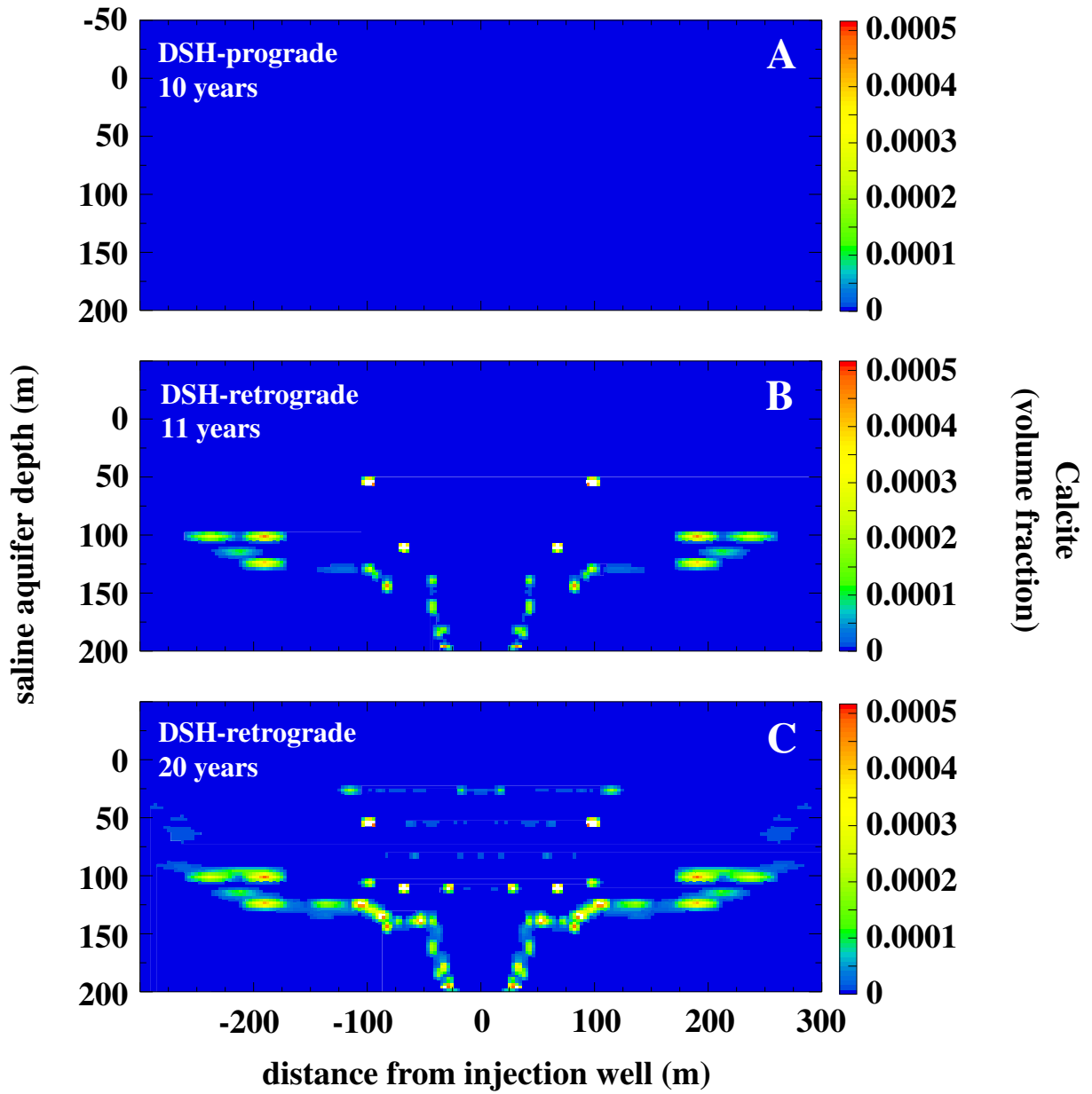
Figure 21: Evolution of Calcite [\text{CaCO}_3] precipitation within the saline aquifer and intra-aquifer shales of model DSH during prograde (10 years, no precipitation) and retrograde (11 and 20 years) sequestration.
