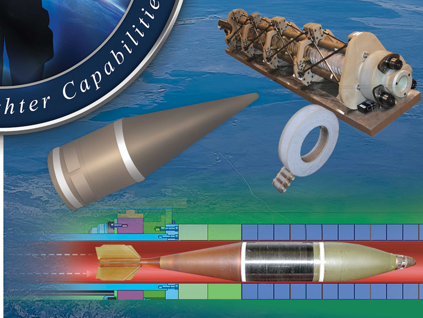
Sandia 120 mm Pulsed Induction Coilgun for Kinetic and Non-Kinetic Missions
