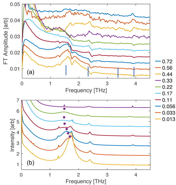
FIG. 5. (color online) Frequency spectrum of the optical reflectivity data in Fig. 3 extracted from (a) a Fourier-transform (FT) after background subtraction, and (b) the linear prediction procedure discussed in the text [27]. The incident fluence for each trace is indicated next to the FT traces (in mJ/cm²). The purple dots in (b) mark the frequency of the LP component ascribed to the soft-mode. Vertical bars indicate the frequencies of the most prominent phonon modes of SmTe₃ observed in Raman scattering [17].
