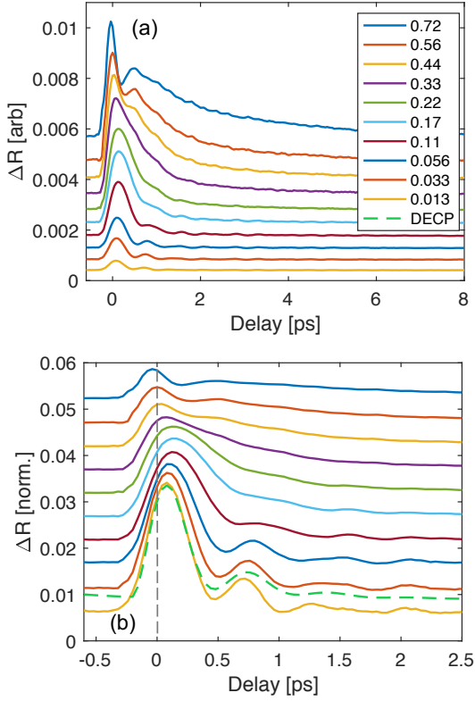
FIG. 3. (color online) (a) Differential reflectivity at a wavelength of 800 nm as a function of pump-probe delay. The pump wavelength was 800nm and the incident fluence for each trace is labeled in the caption in \text{mJ}/\text{cm}^2 . (b) Zoomed view of the data in (a) normalized by the incident fluence. The dashed curve is a DECP fit of the 0.033 \text{ mJ}/\text{cm}^2 with \Omega/2\pi = 1.55 \text{ THz} , \gamma = 2.5 \text{ THz} , \beta = 1.95 \text{ THz} . The vertical dashed line marks the t = 0 point.
