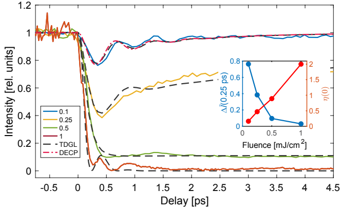
FIG. 6. (color online) Time dependent Ginzburg-Landau model of the dynamics of the order parameter. The solid lines are the time dependence of the structure factor for the (17 q ) reflection as in Fig. 2 (a). The dark dashed lines are the solutions to the TDGL for the values reported in Table I. For comparison, the dashed-dotted line shows the DECP fit from Fig. 2. The inset shows the fluence dependence of the measured intensity \tilde{I}(0.25 \text{ ps}) and the fitted value of \eta(0) (from table I).
