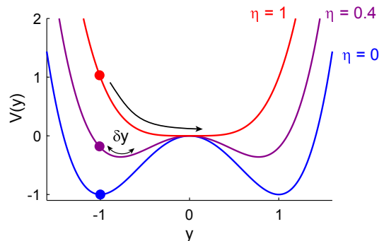
FIG. 1. (color online) Normalized Ginzburg-Landau potential V(y) of the anharmonic lattice dynamics model for various levels of excitation.
