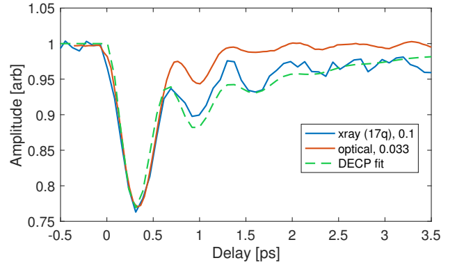
FIG. 4. (color online) Comparison between x-ray and optical data for the lowest fluence. The dashed line is the DECP fit of the x-ray data in Fig. 2.
