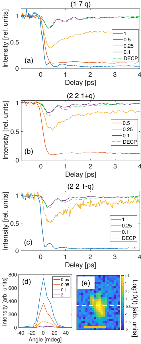
FIG. 2. (color online) (a-c) Dynamics of CDW X-ray diffraction, \tilde{I} , for several incident fluences for CDW peaks (a) (1 7 q), (b) (2 2 1+q) and (c) (2 2 1-q). The caption in (a-c) indicates the incident fluence in mJ/cm 2 . The green dashed line is a fit using Eq. (10), the parameters of the fit (given in the text) are the same for all panels. (d) lineout of the intensity across the detector along the dashed line indicated in (e). Panel (e) shows the detector image of the (17q) CDW Bragg peak, the horizontal scale bars is 9 \times 10^{-4} \text{ \AA}^{-1} , the intensity scale is logarithmic.
