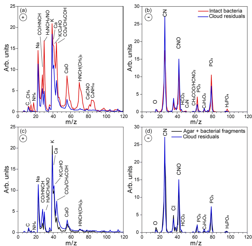
Figure 6. Positive (a) and negative (b) ion average mass spectra of cloud residuals sampled during Expansion 1 (blue) superimposed on the average MS of intact bacteria (red). Panels (c) and (d) show the same cloud residuals average MS superimposed on the reference average MS of the small particle mode, composed of Pseudomonas syringae bacterial fragments mixed with agar (black).
