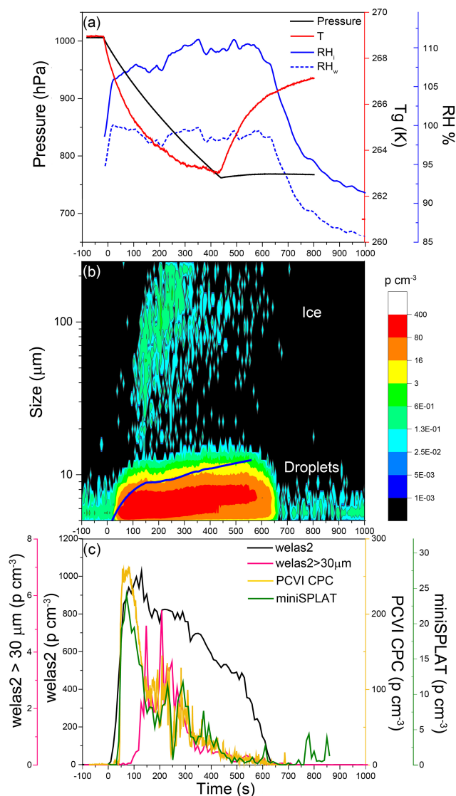
Figure 9. Data from Expansion 2 with PF CGina bacteria. (a) The pressure (black) and the temperature of the gas (red) inside the AIDA chamber. The measured RH with respect to ice ( \text{RH}_i ) and water ( \text{RH}_w ) is indicated in solid and dashed blue lines, respectively; (b) the size distributions of the particles measured with welas2 during the expansion. Particles smaller than \sim 15 \mu\text{m} are liquid droplets, while larger particles are ice. The PCVI cut size is shown by the blue trace. (c) The welas2-measured total particle number concentrations (black) and the number concentrations of particles larger than 30 \mu\text{m} (pink). The number concentrations of particles transmitted by the PCVI and measured by CPC and miniSPLAT are marked in yellow and green, respectively.
