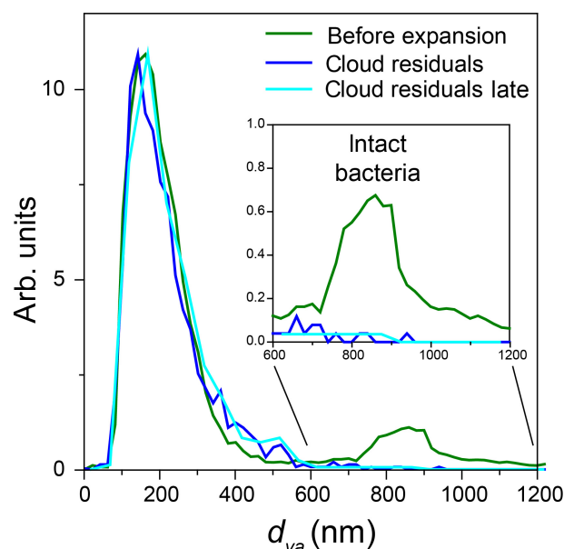
Figure 14. d_{va} size distribution, measured by miniSPLAT before Expansion 3 (green) with PF CGina bacteria, of cloud residuals (blue) and of cloud residuals measured during the later part of the expansion (302–557 s) when the number concentration of sampled droplets and ice crystals was nearly the same (light blue). The inset shows an expanded scale of the region of intact bacteria.
