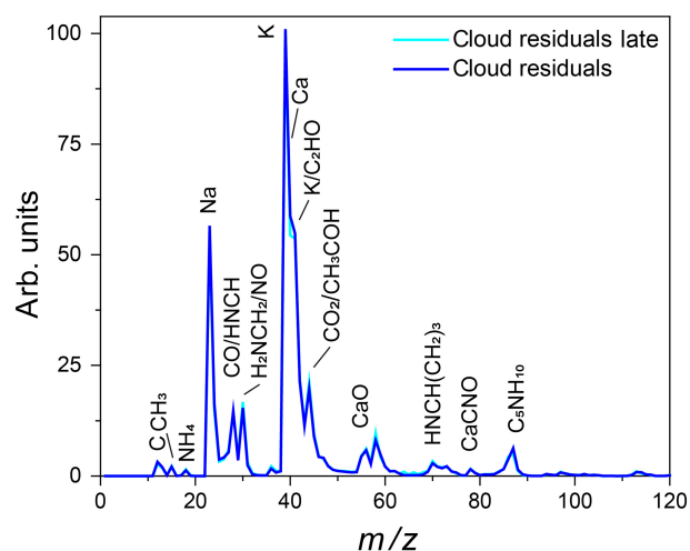
Figure 15. Average mass spectrum of cloud residuals measured during Expansion 3 (blue) with PF CGina bacteria super imposed on the average mass spectrum of particles characterized later in the expansion (302–557 s) when the number of sampled ice crystals and cloud droplets was comparable (light blue).
