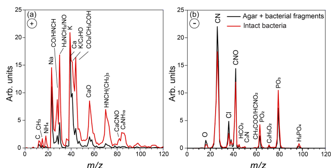
Figure 2. Positive (a) and negative (b) average mass spectra of the particles in the AIDA chamber, measured before Expansion 1. Reference mass spectra of the small size mode, made up of bacterial fragments mixed with agar, which includes particles smaller than 300 nm, are marked in black, and the mass spectra of the large size mode particles ( d_{va} > 70 nm), composed of intact Pseudomonas syringae bacterial cells, are marked in red.
