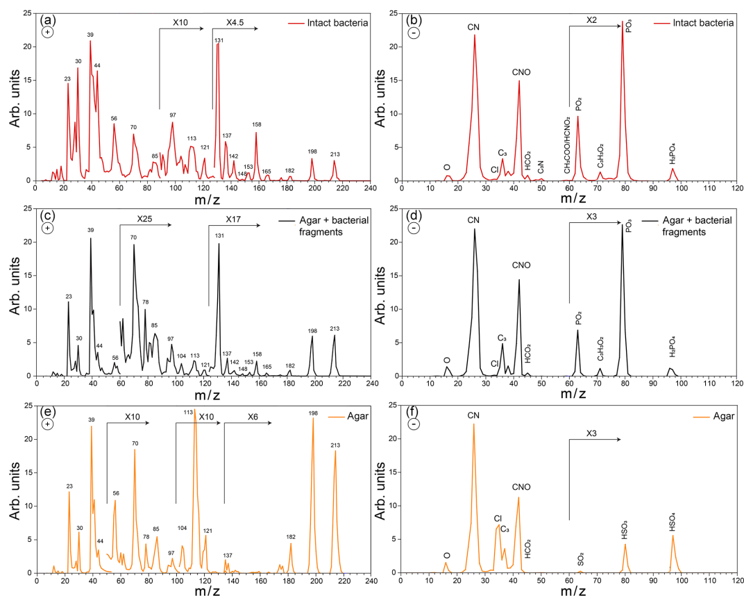
Figure 3. Positive (a) and negative (b) average mass spectra (MS) of intact Pseudomonas syringae bacteria measured before Expansion 1; positive (c) and negative (d) average MS of the small particle mode measured before Expansion 1; positive (e) and negative (f) average MS of pure agar particles measured in a separate experiment.
